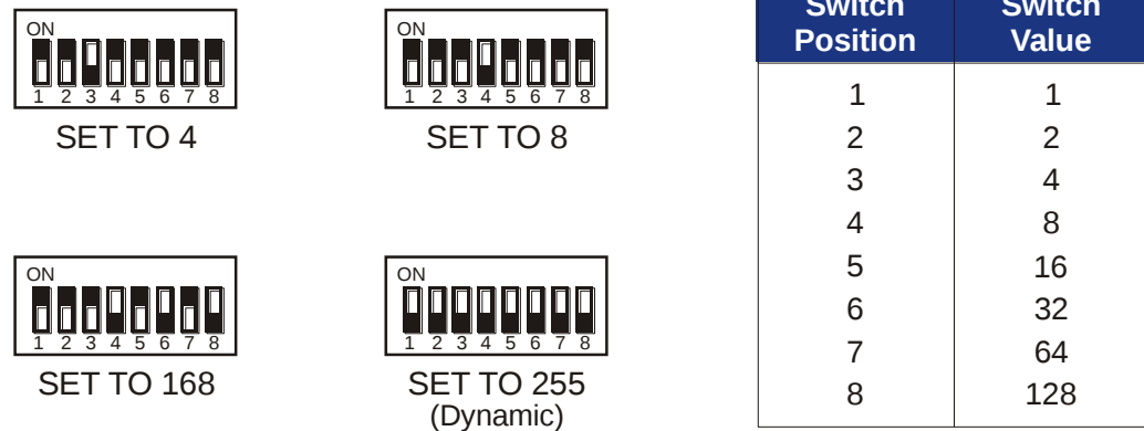
FIGURE 2-1: LOGICAL ADDRESS SWITCH SETTING EXAMPLES
