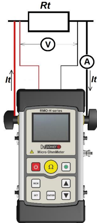
Figure 3-1: Connecting a test object to RMO-H
