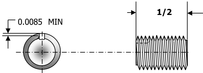
GO WORKING PLUG
