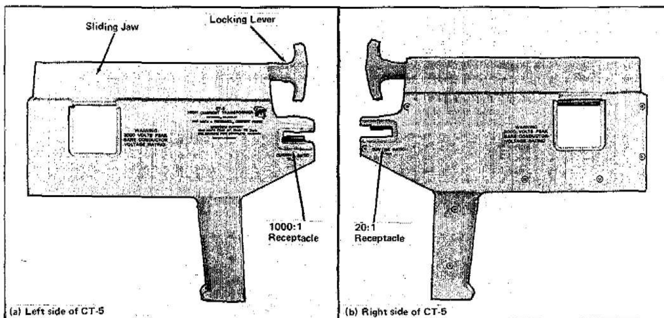
Fig. 2-1. CT-5, showing 1000:1 and 20:1 Current Ratio receptacles.
