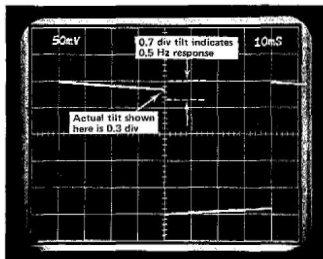
Fig. 4-2. Typical response of the CT-5 with P6042 to a low-frequency square wave signal. A tilt of 0.7 div indicates a -3 dB response of 0.5 Hz.
