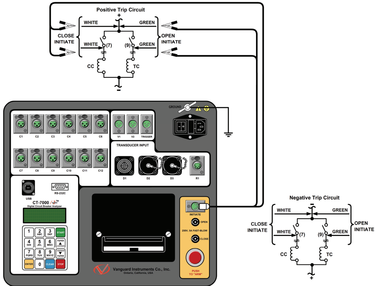
Figure 5. Typical DC Trip and DC Close Control Circuit Connection
