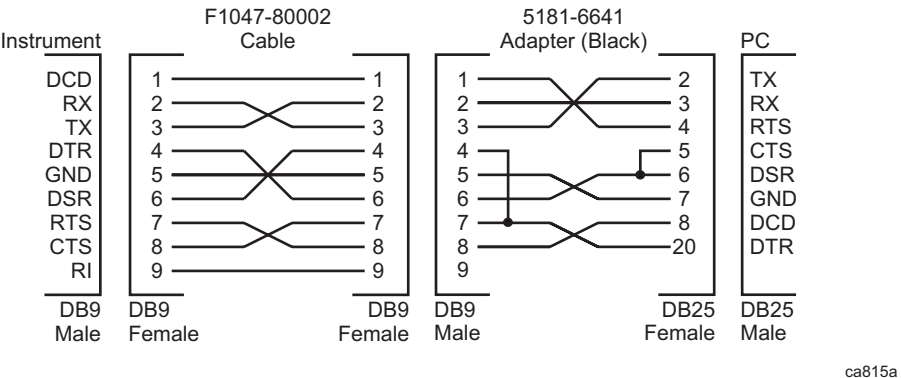
Figure 1-13 HP/Agilent F1047-80002 Cable with 5181-6641 Adapter
