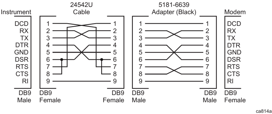
Figure 1-12 HP/Agilent 24542U Cable with 5181-6639 Adapter
