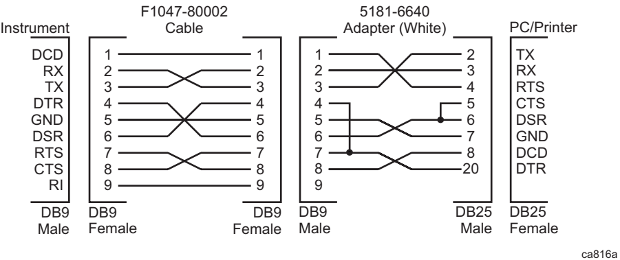
Figure 1-14 HP/Agilent F1047-80002 Cable with 5181-6640 Adapter
