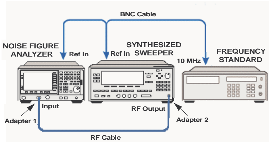
Figure 2-7 Frequency Accuracy test setup
