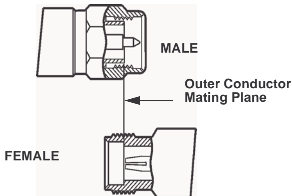
Figure D-2 Precision 3.5mm connectors
