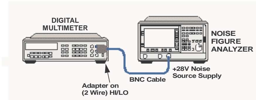
Figure 2-13 Equipment setup for Noise Source Supply Accuracy test
