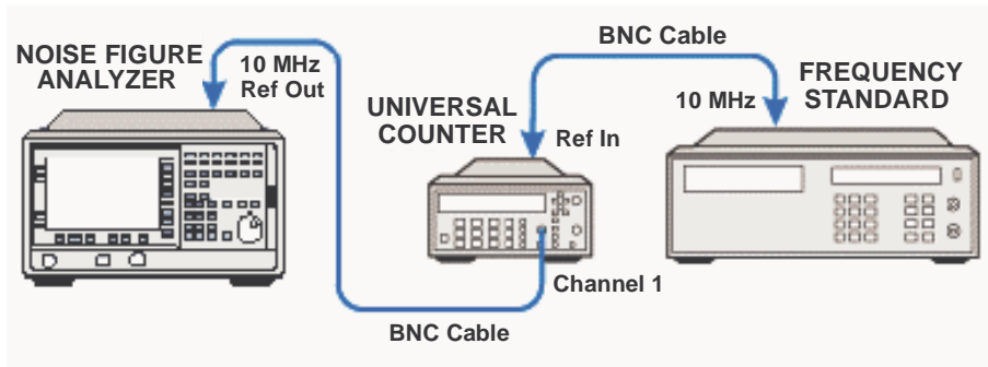
Figure 2-2 10 MHz Out Frequency Reference Adjustment Test Setup
