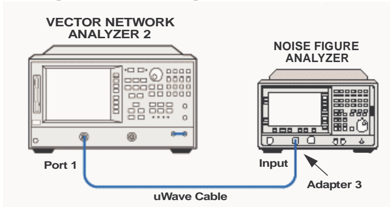
Figure 2-6 Input VSWR Test Setup 2
