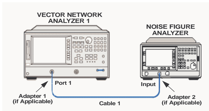
Figure 2-4 Input VSWR Test Setup 1
