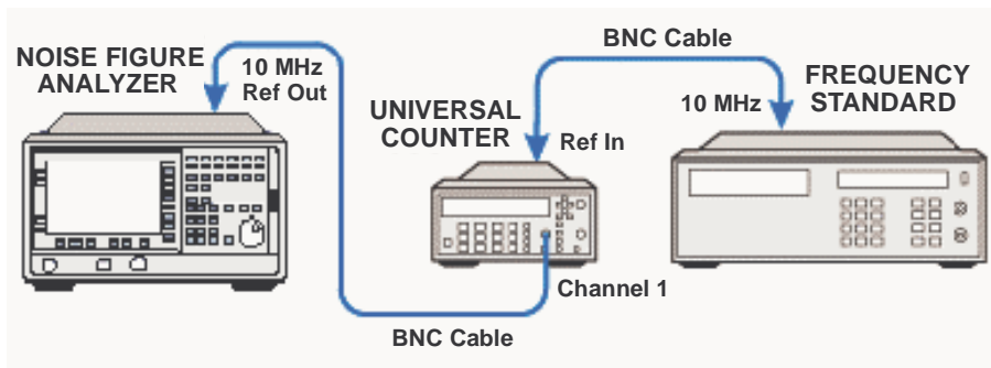
Figure 2-1 10 MHz Out Frequency Reference Accuracy Test Setup
