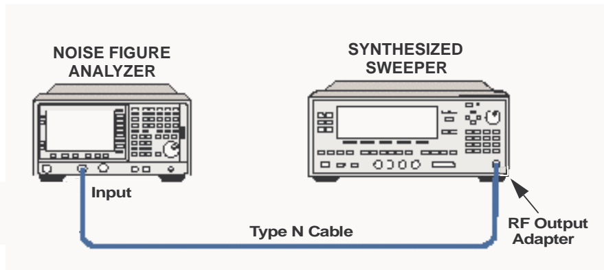
Figure 2-16 Gain Measurement Uncertainty Test Setup
