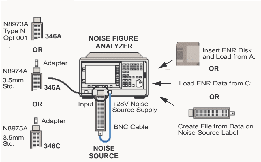
Figure 2-20 Instrument Noise Figure Test Setup
