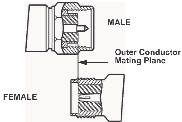
Figure D-3 SMA connectors
