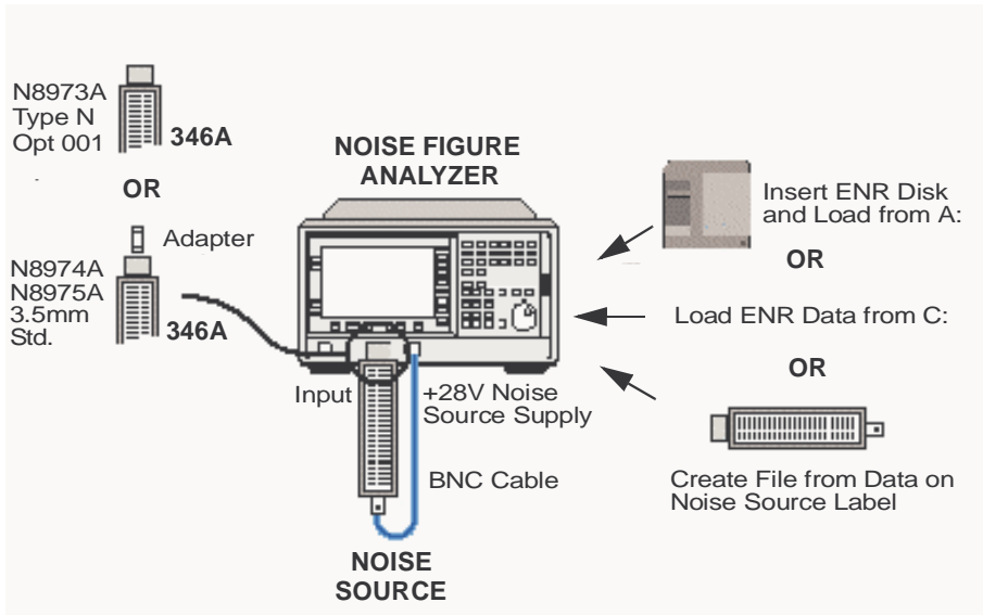
Figure 2-24 Measurement Jitter Test Setup
