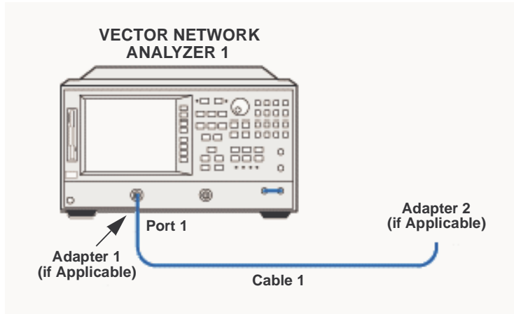
Figure 2-3 Input VSWR: Equipment Connection
