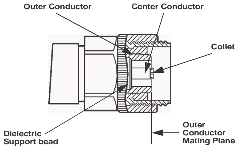
Figure D-1 Precision 7mm Connector
