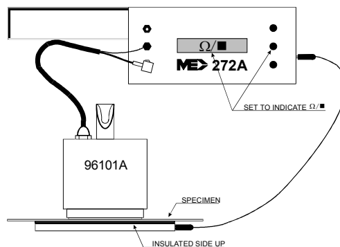
Figure 1 Setup for Surface Resistivity Measurement
