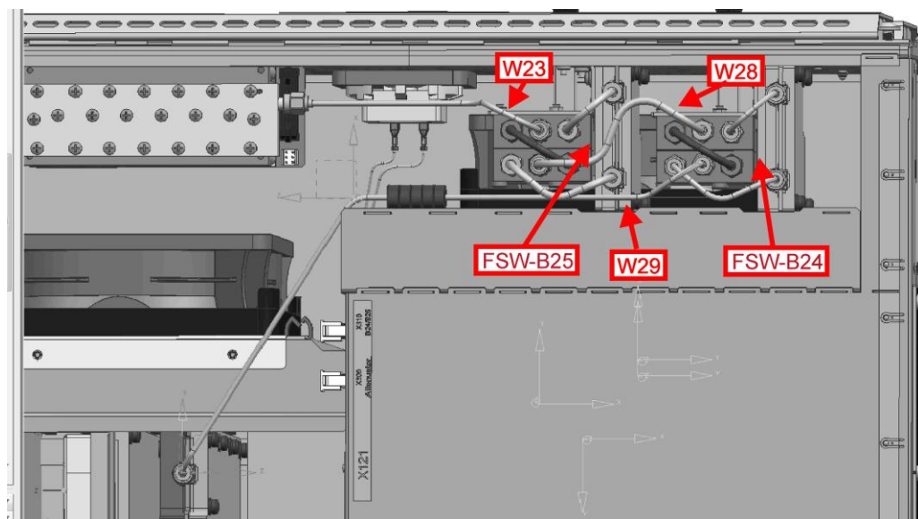
Figure 3-15: Cabling of an R&S FSW8 equipped with R&S FSW-B24 and B25
