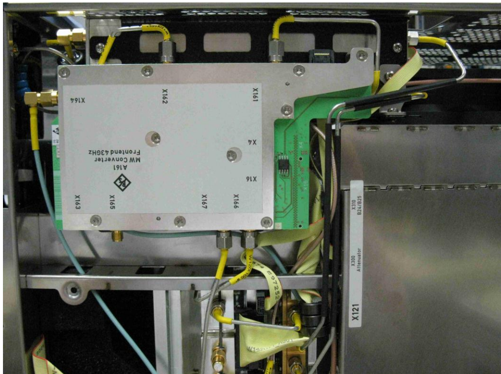
Figure 3-24: Cable routing on the lower side of an R&S FSW67 without option R&S FSW-B24 installed
