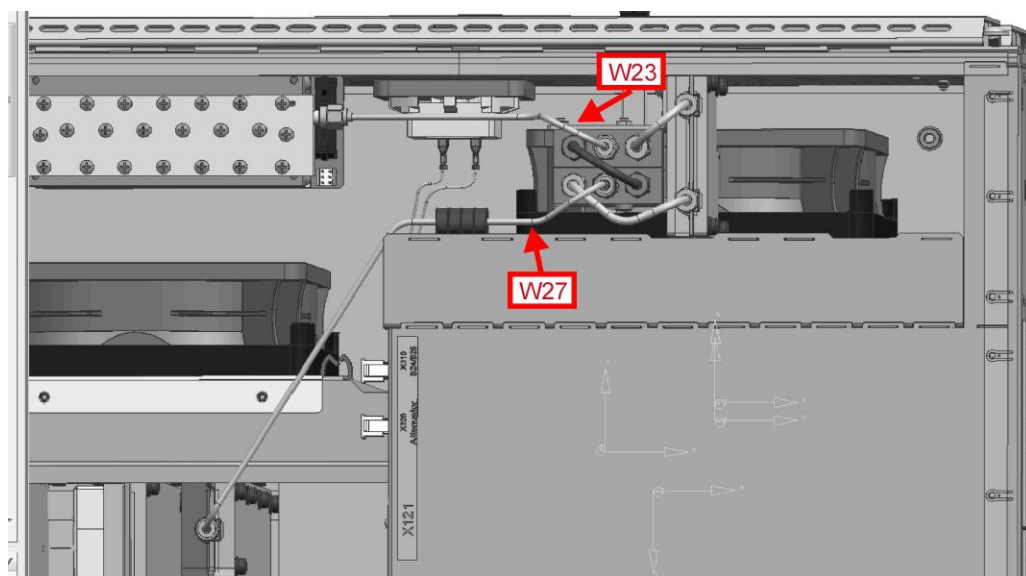
Figure 3-17: Cabling of an R&S FSW8 equipped with R&S FSW-B25
