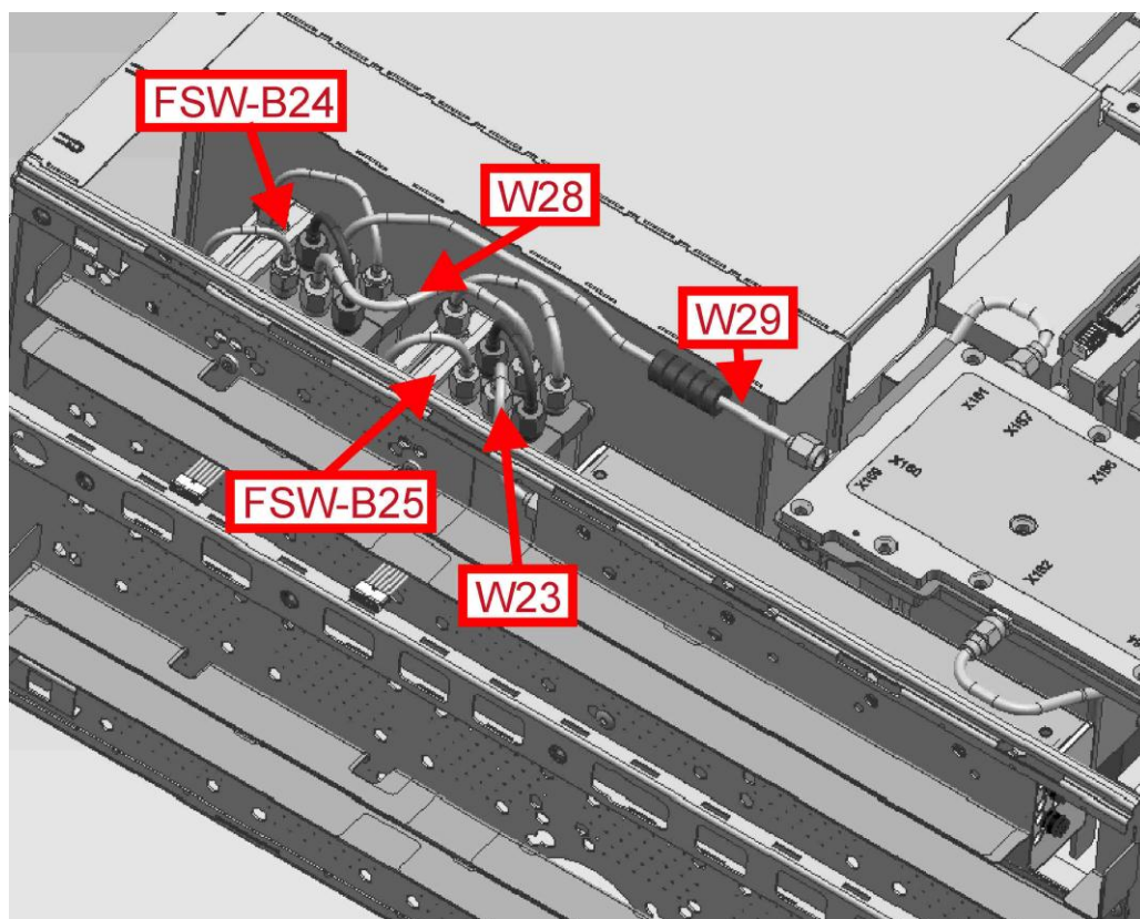
Figure 3-20: Cabling of an R&S FSW13/26 equipped with R&S FSW-B24 and B25
