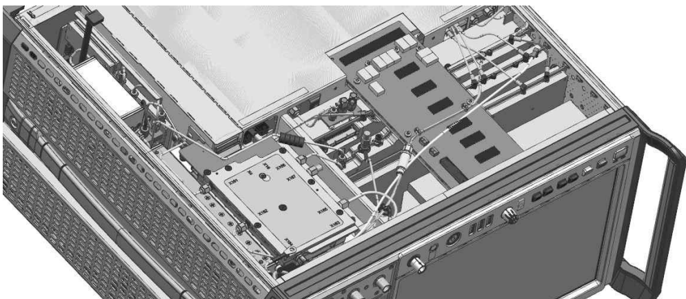
Figure 3-7: Cable routing on the lower side of an R&S FSW43 with option R&S FSW-B24 installed
