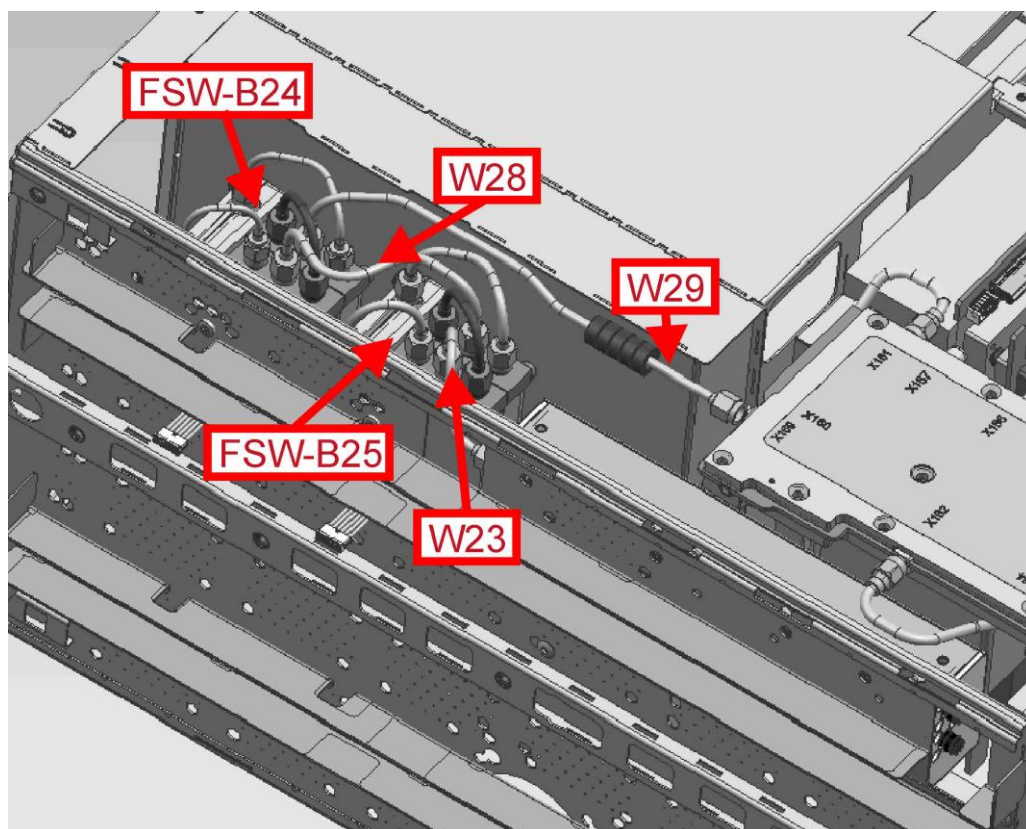
Figure 3-14: Cabling of an R&S FSW13/26 equipped with R&S FSW-B24 and B25
