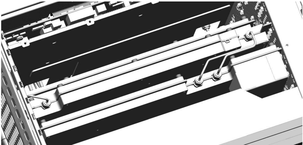
Figure 3-6: Cable routing on the upper side of an R&S FSW13/26/43 without options R&S FSW-B24 and R&S FSW-B25.
