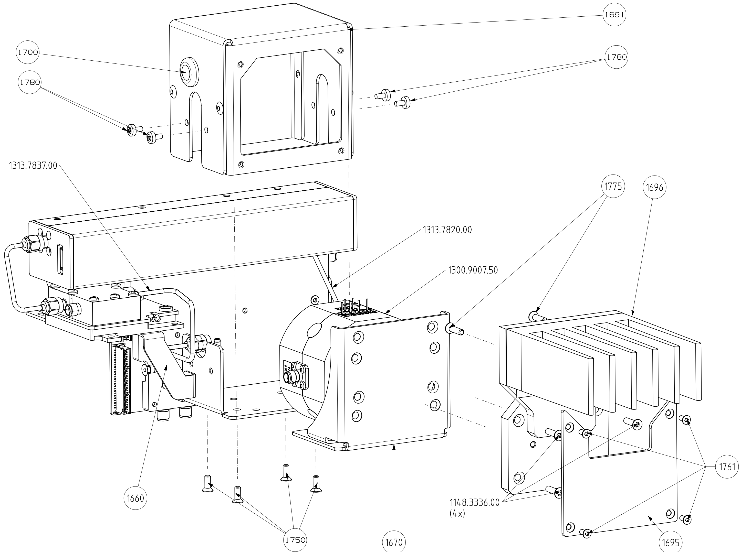
Pos. 1612 YIG Filter R&S VAR 50
