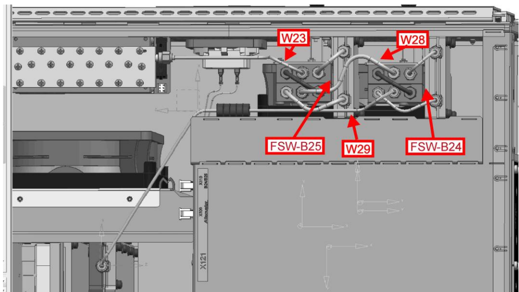
Figure 3-19: Cabling of an R&S FSW8 equipped with R&S FSW-B24 and B25
