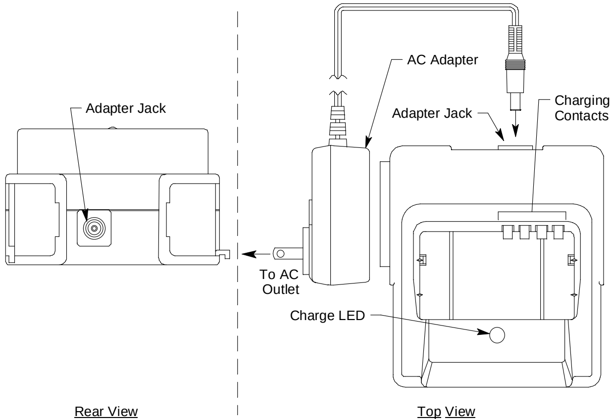
Figure 5: GX-2012 AC Powered Charging Station
