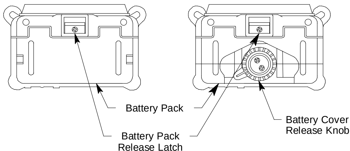
Figure 2: Components of the GX-2012, Bottom
