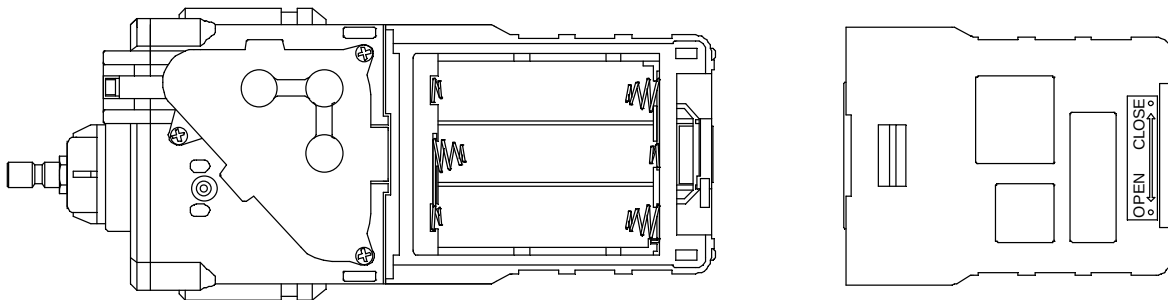
Figure 18: Installing the Alkaline Batteries
