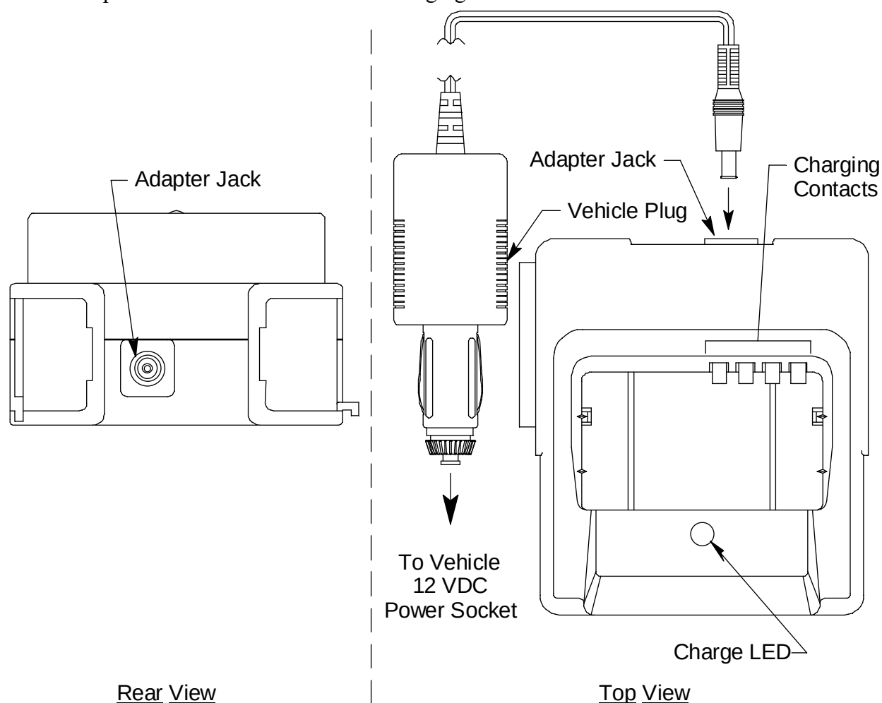
Figure 6: GX-2012 DC Powered Charging Station
