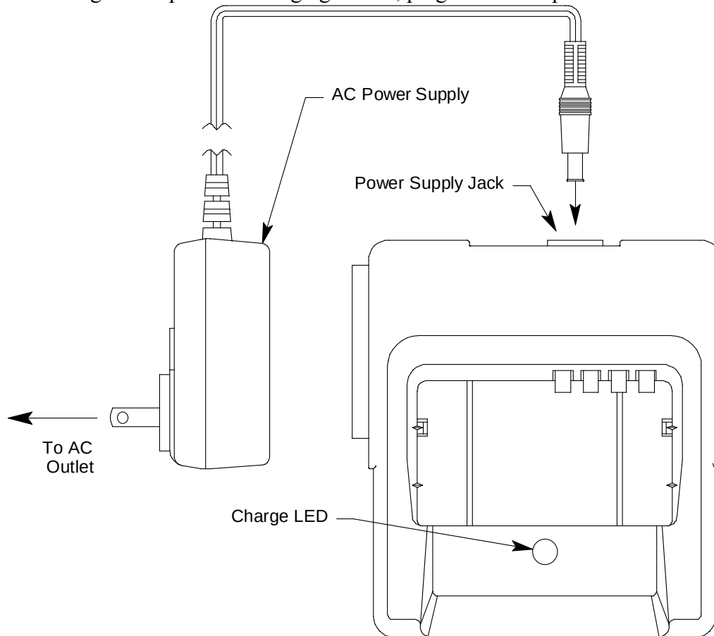
AC Powered Charging Station
