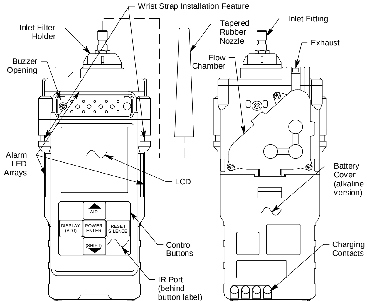
Figure 1: Components of the GX-2012, Front & Back
