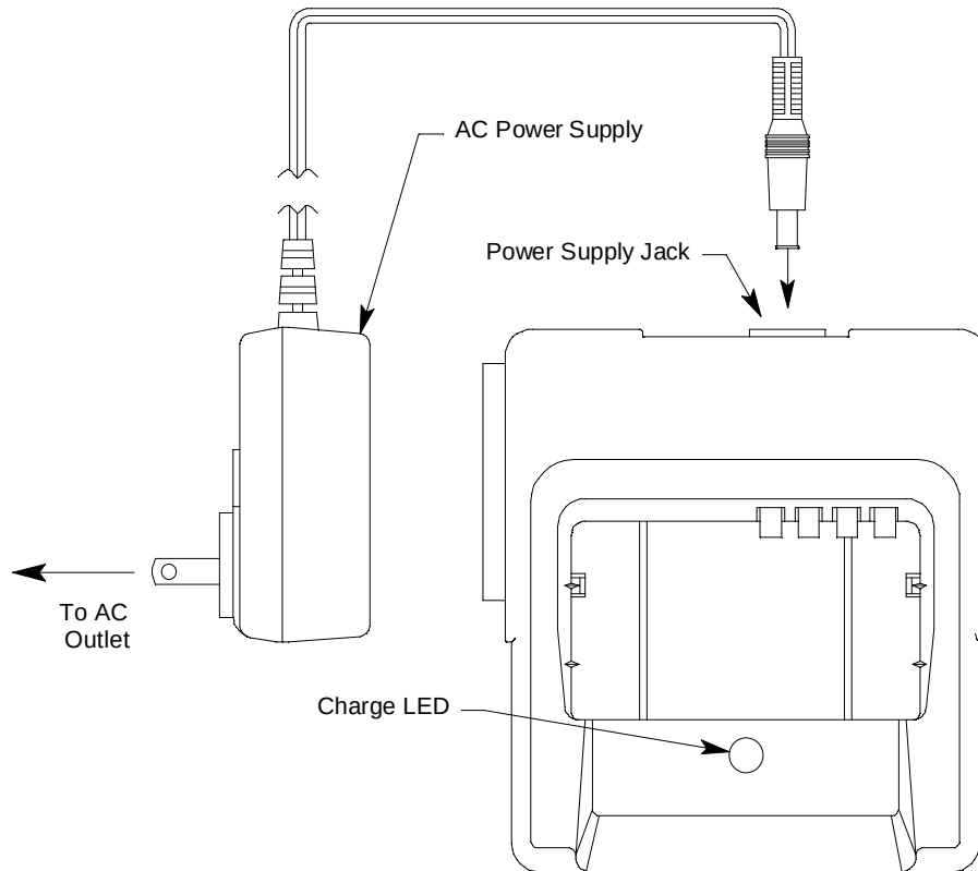
AC Powered Charging Station
