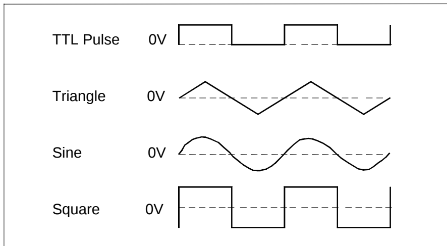
FIG. 3 OUTPUT WAVEFORMS AND PHASE RELATIONSHIPS
