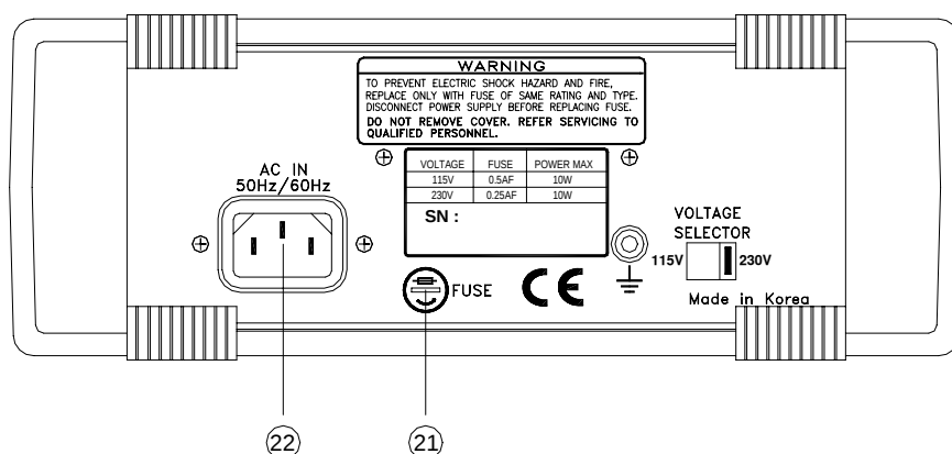
FIG 2. REAR PANEL
