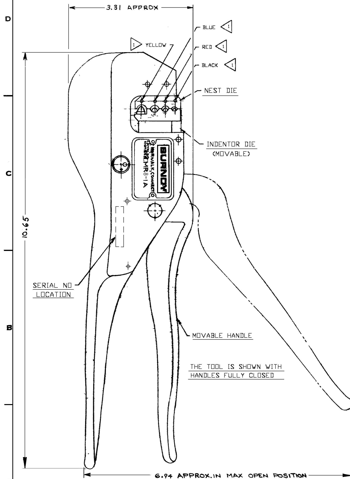
VIEW SHOWING HYTOOL WITH HANDLES FULLY OPENED
