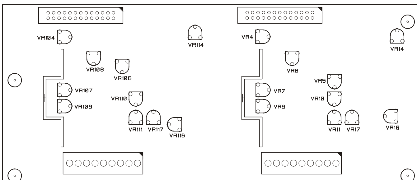
Control pcb calibration points (viewed from rear)
