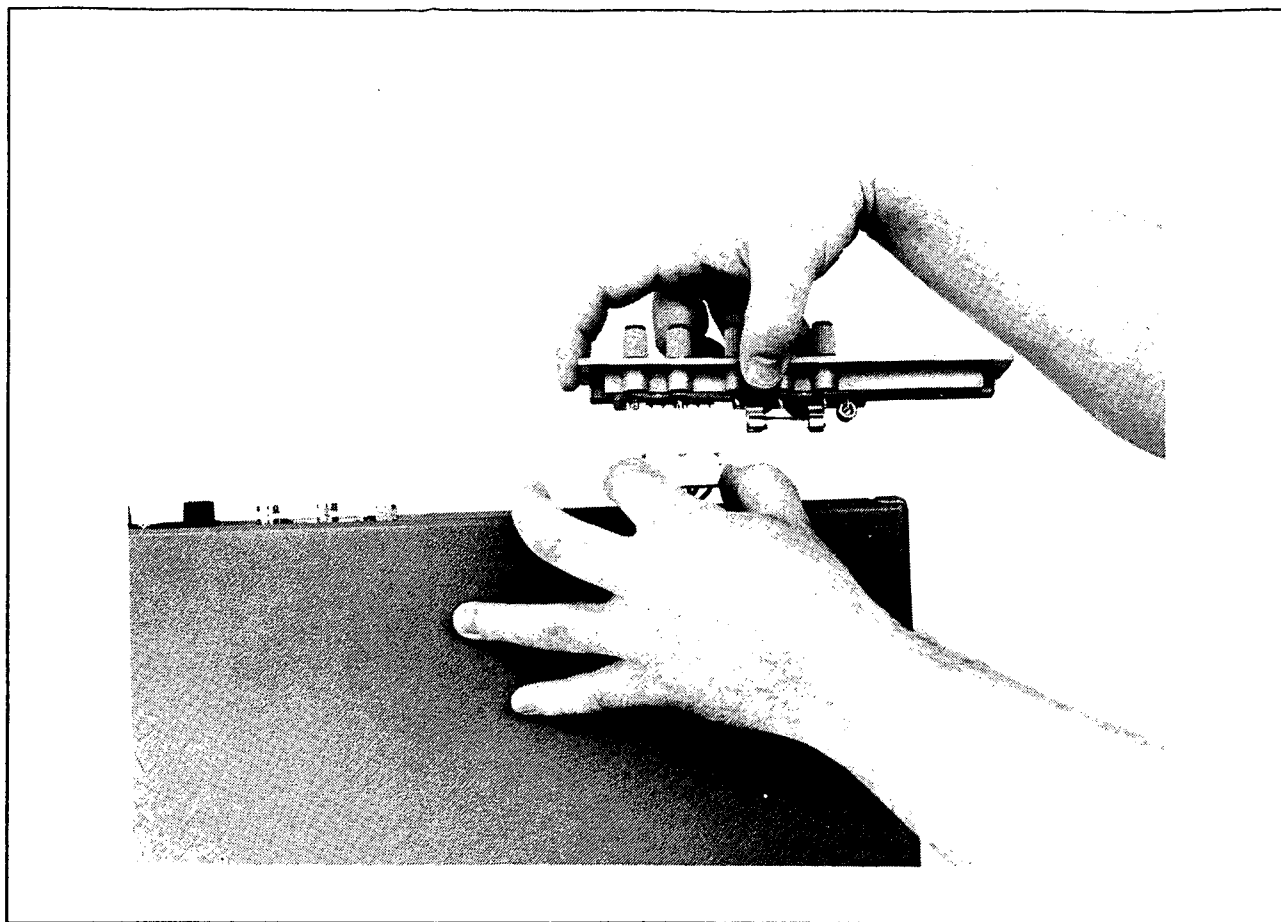
Figure 2-7. Rear Terminal Assembly Removal
