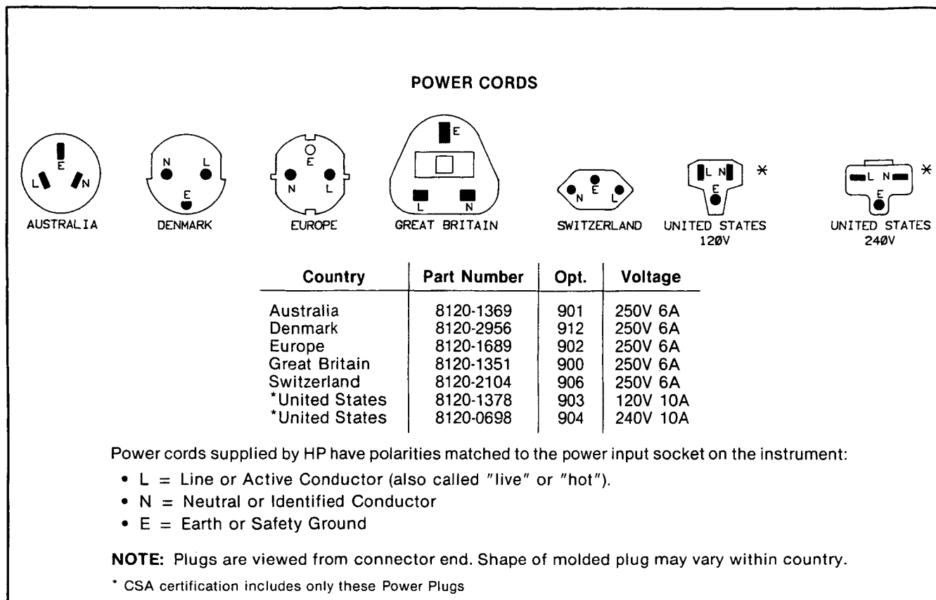
Figure 2-3. Power Cables
