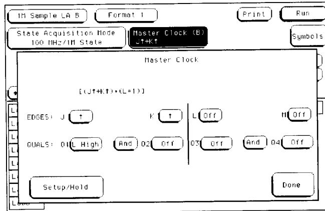
Clock menu in 100 MHz State mode
