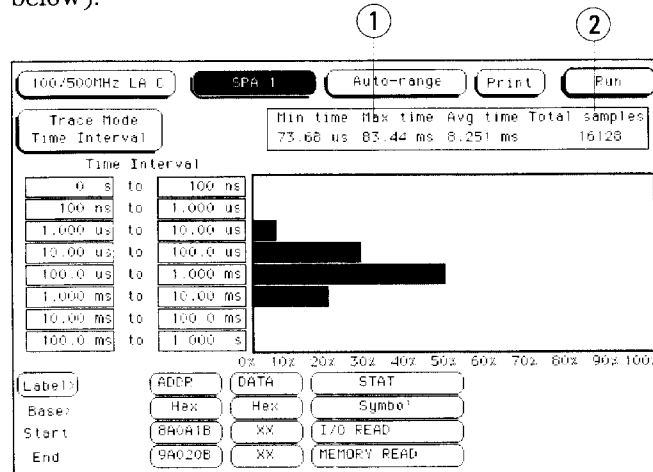
SPA Time Interval Menu with Statistics Called Out
