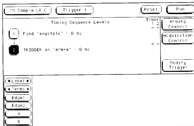
The Trigger Menu
