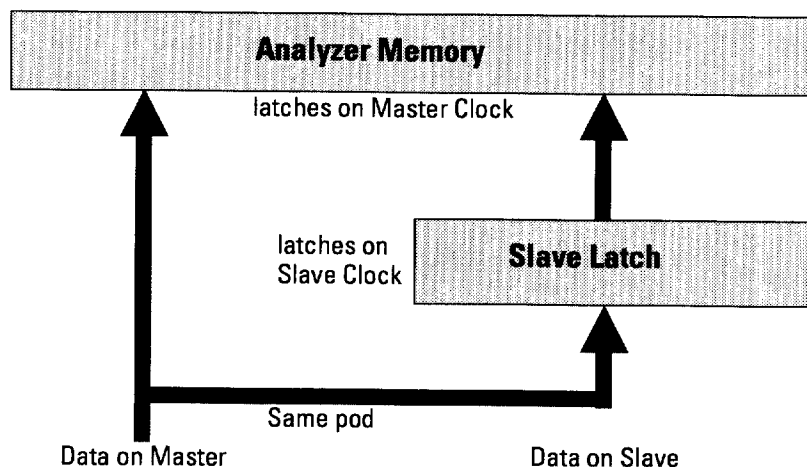
Latching Slave Data in Demultiplex Mode
