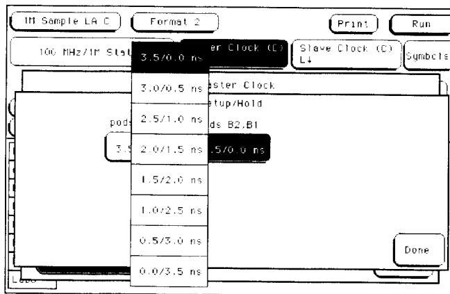
Setup and Hold Menu
