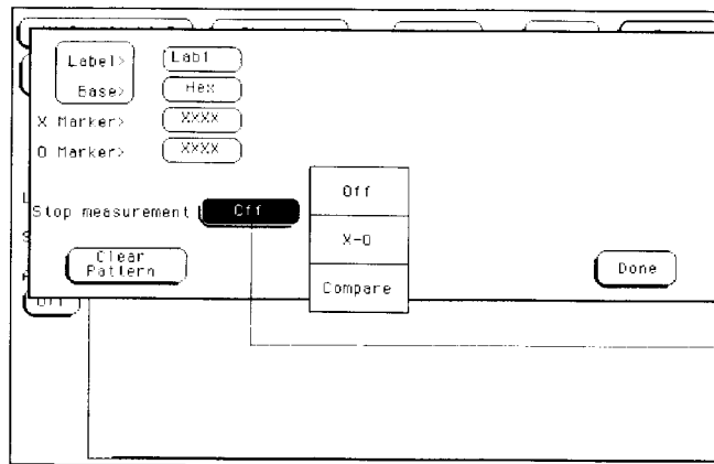
Stop Measurement Field and Pop-up Menu
