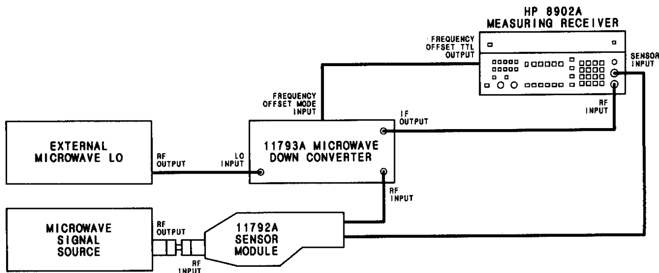
Figure 1. Sensor Module Interconnections
