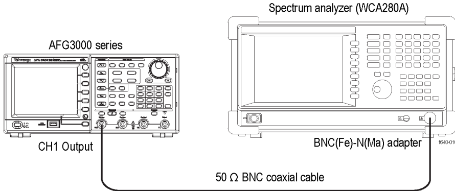
Figure 13: Spurious tests
