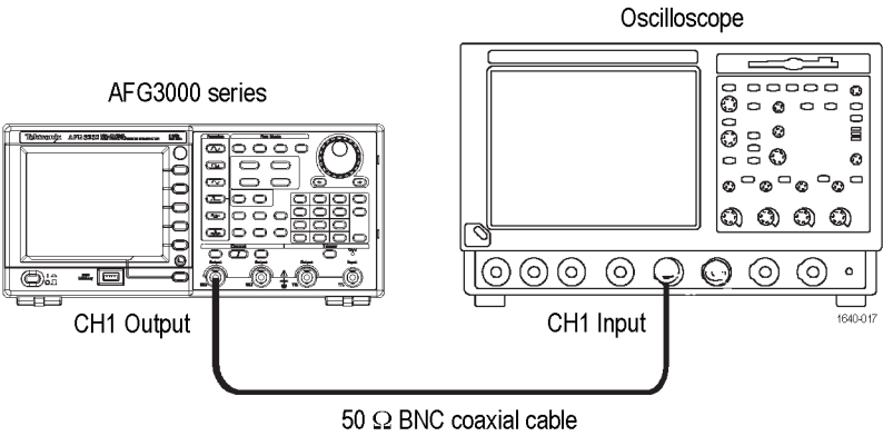
Figure 14: Rise-Fall time tests
