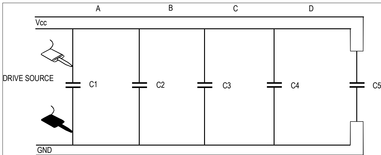
Isolation of Open Circuit Decoupling Capacitor
