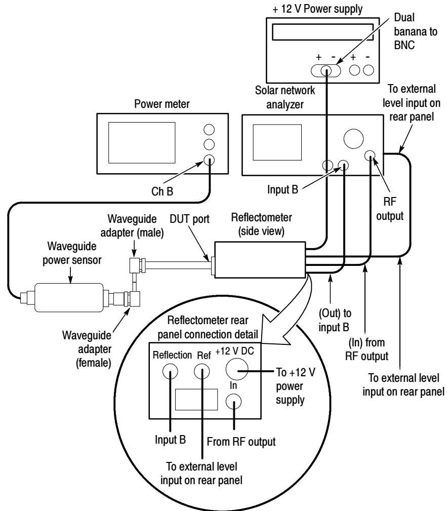
Figure 2-33: Adapter-loss hookup
