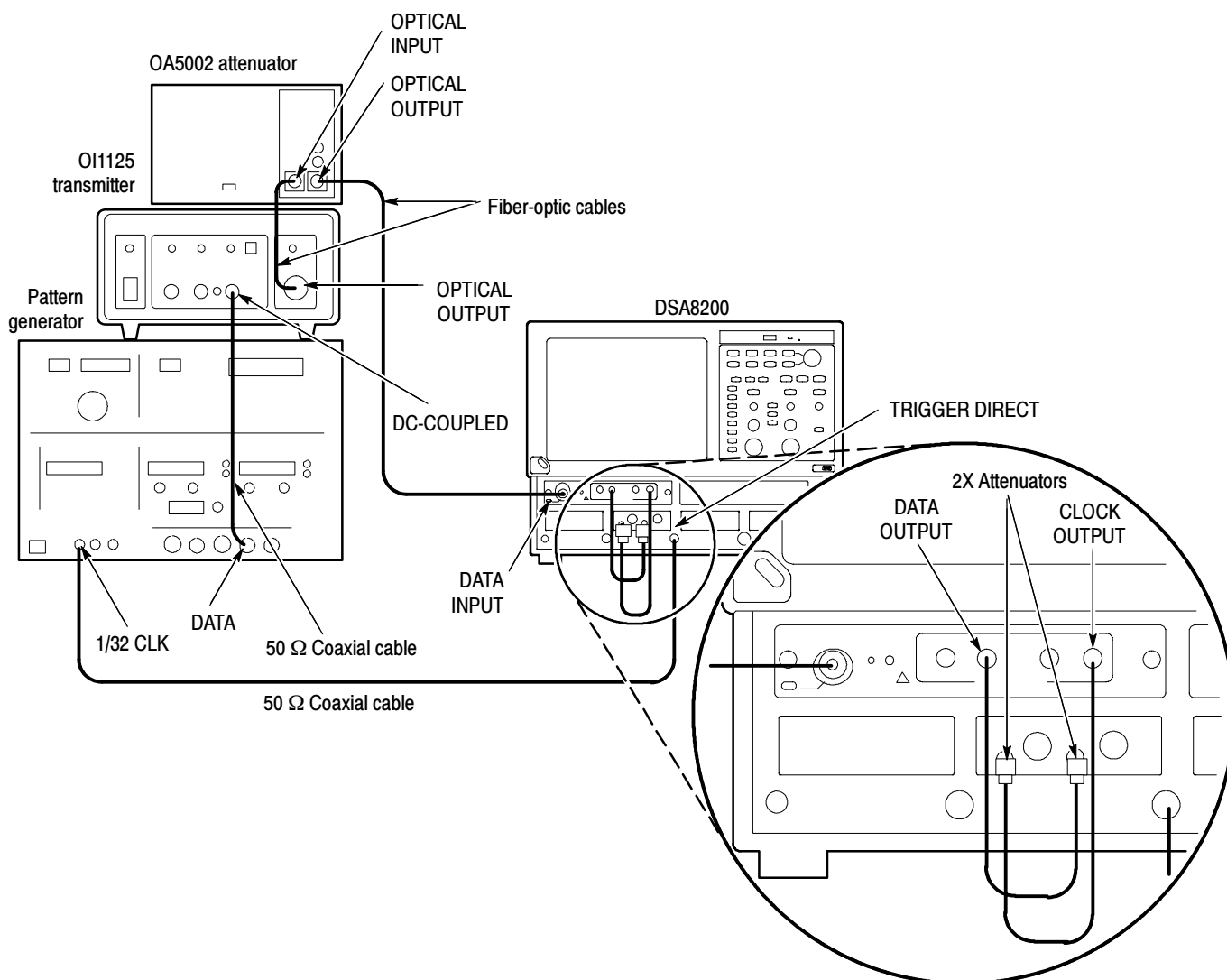
Figure 2- 44: Clock recovery optical sensitivity range and recovered clock timing jitter hookup
