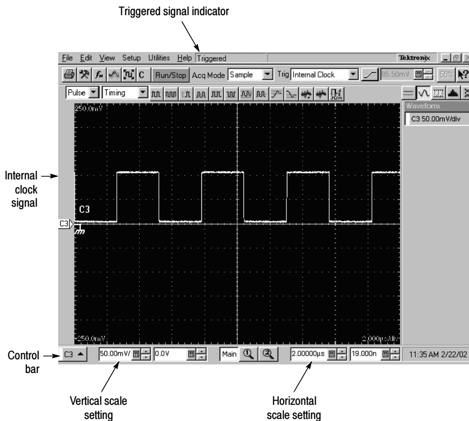
Figure 2-12: Signal triggered
