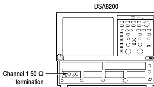
Figure 2-37: TDR system step response aberrations hookup
