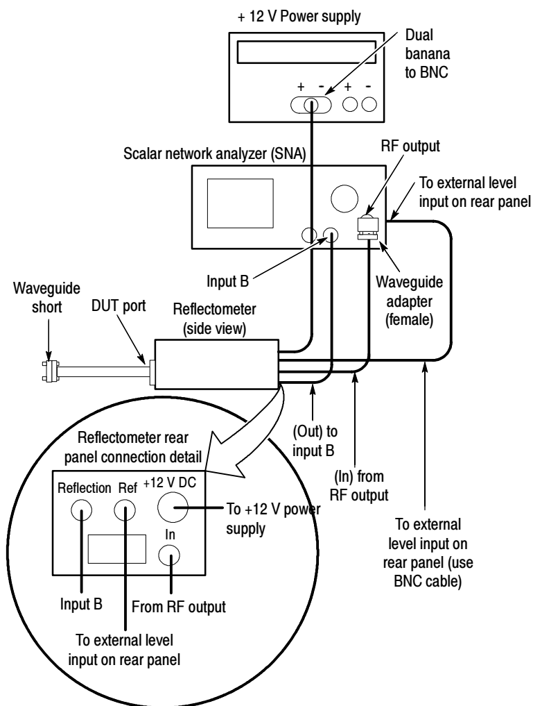
Figure 2- 30: SNA/Waveguide characterization
