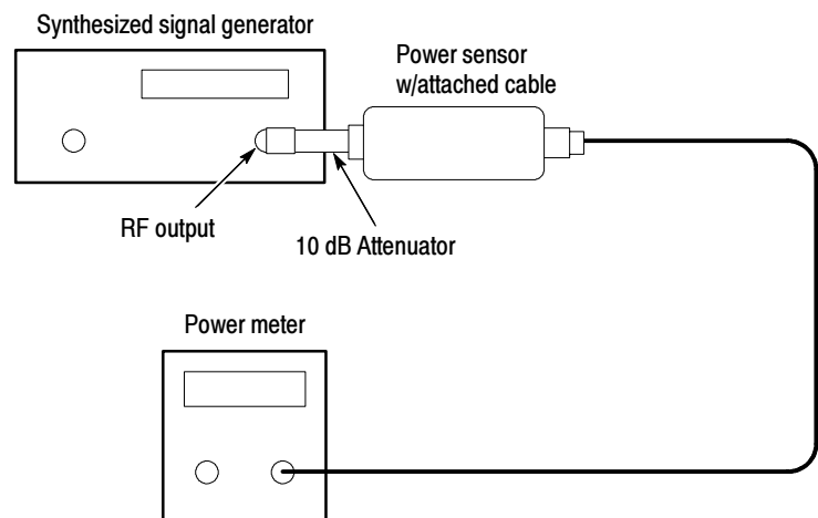
Figure 2- 26: Power-reference hookup
