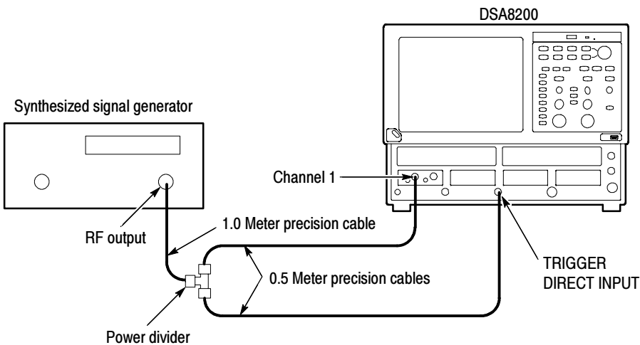
Figure 2- 19: External direct trigger jitter test hookup
