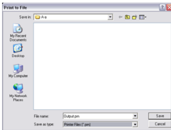
Figure 384. Print-to-File Browser.
