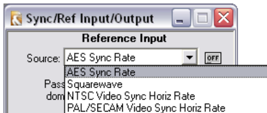
Figure 391. Sync/Ref Sources.
