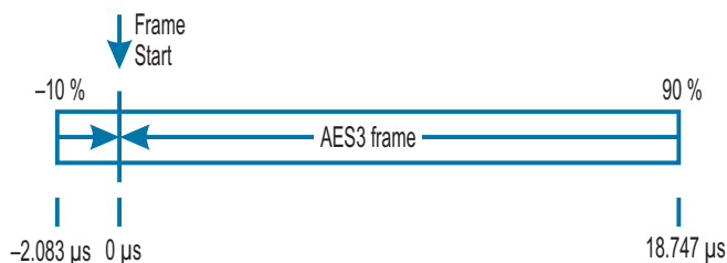
Figure 153. The Delay from Ref Out measurement range, showing times that correspond to a sample rate of 48 kHz.
