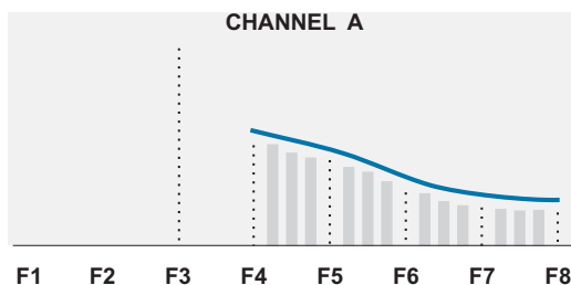
Figure 268. Example of a multitone distortion response.
