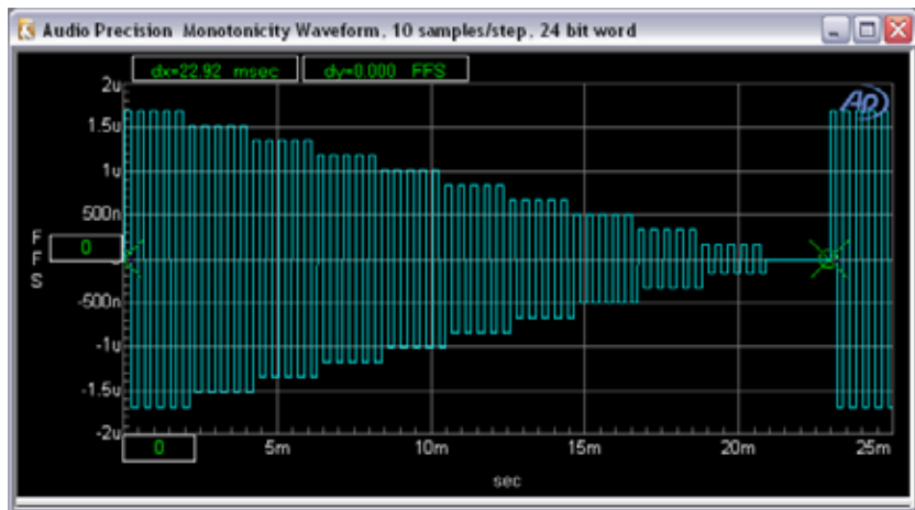
Figure 91. Monotonicity waveform. 24-bit resolution, 10 samples/step, 48 kHz sample rate.
