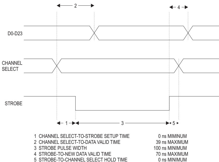
Figure 19. Parallel Output Port timing relationships.
