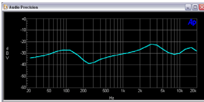
Figure 267. Typical Multitone Response measurement, amplitude vs. frequency.
