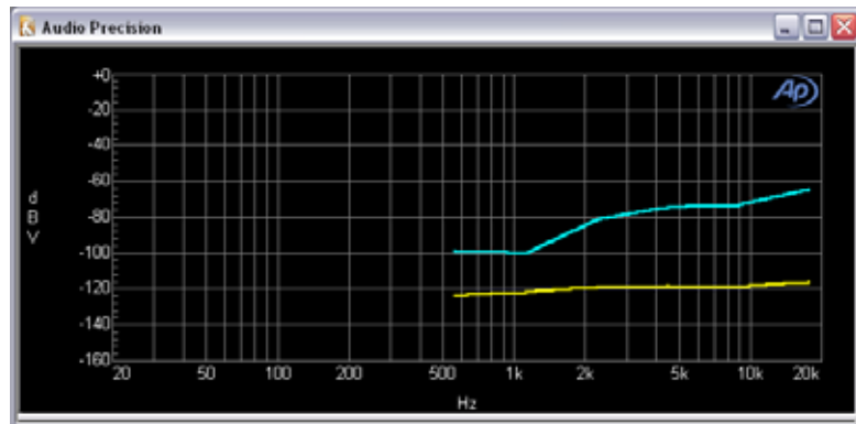
Figure 274. Typical Multitone Crosstalk measurement.
