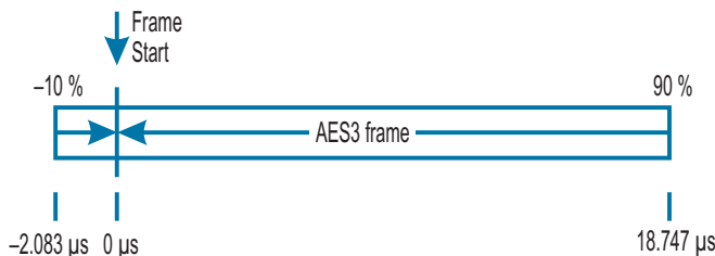
Figure 392. The Delay, In from Ref In measurement range, showing times that correspond to a sample rate of 48 kHz.
