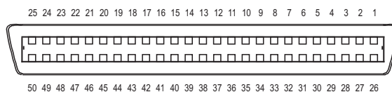
Figure 20. Parallel I/O connector pin locations.
