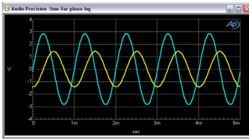
Figure 37. Sine (D/A): Var Phase , triggered on Channel A (the larger waveform). -90.00^\circ has been entered in Phase B-A field, causing B (the smaller waveform) to lag A.
