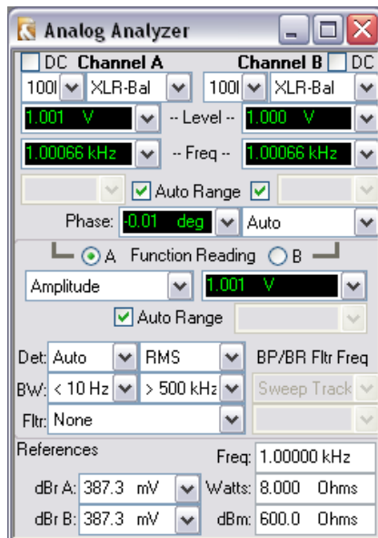
Figure 101. The 2700 series Analog Analyzer panel.
