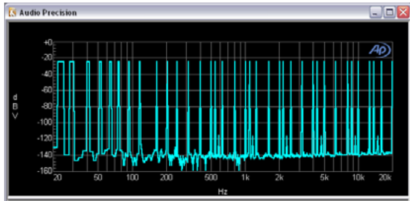
Figure 255. Spectrum View of Typical Multitone Stimulus Signal.
