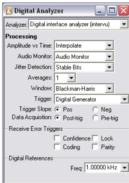
Figure 243. The Digital Interface Analyzer panel.
