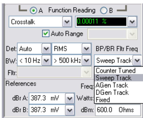
Figure 129. Analog Analyzer Function meter Bandpass/ Bandreject filter tuning.
