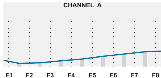
Figure 270. Example of a multitone noise response.
