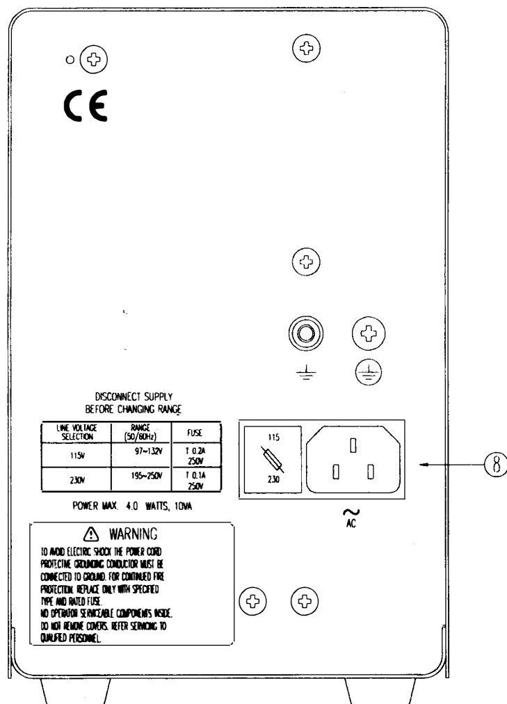
Rear Panel
