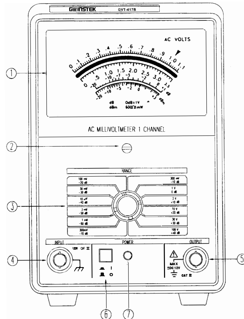
Front Panel
