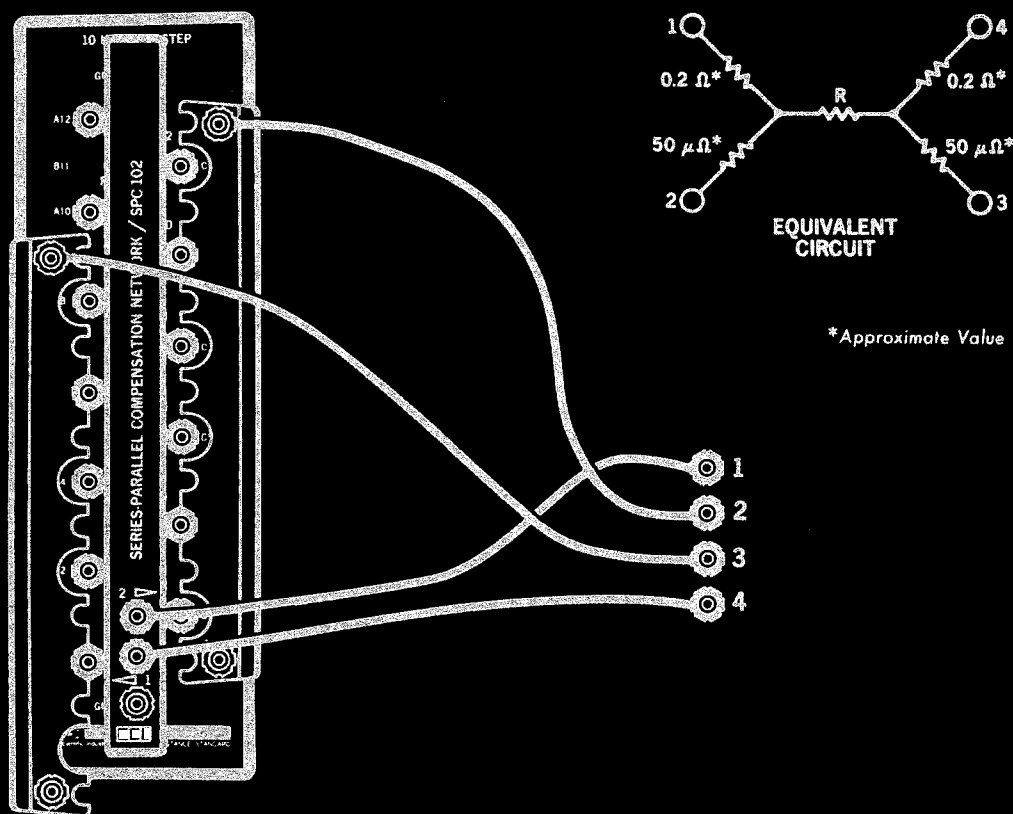
Figure 3-7. Series-Parallel Connection with Compensation Network
