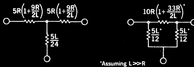
Figure 4-13. Fourth "T" to "Pi" Transform
