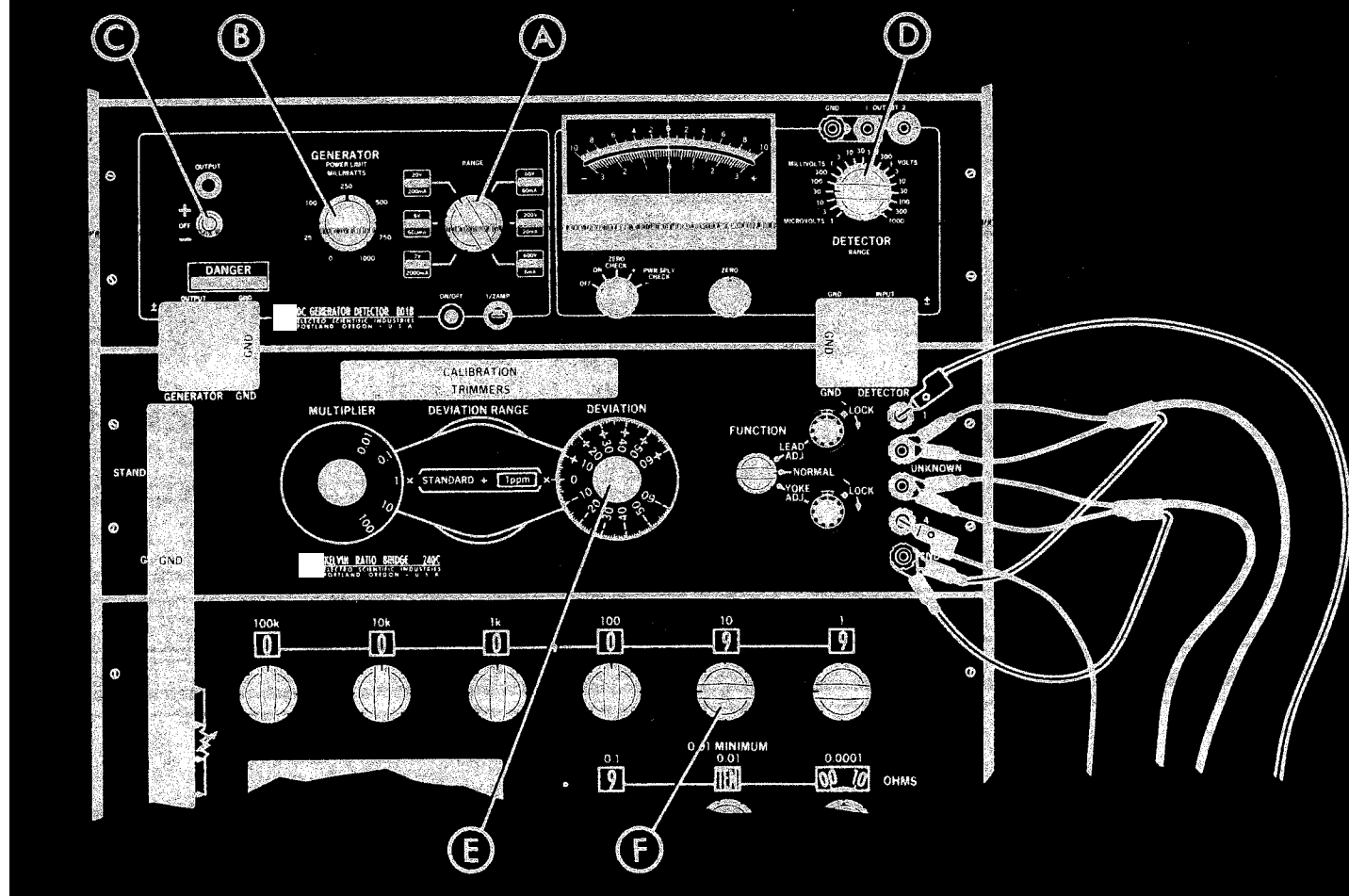
Figure 5-13. System Dial Settings
