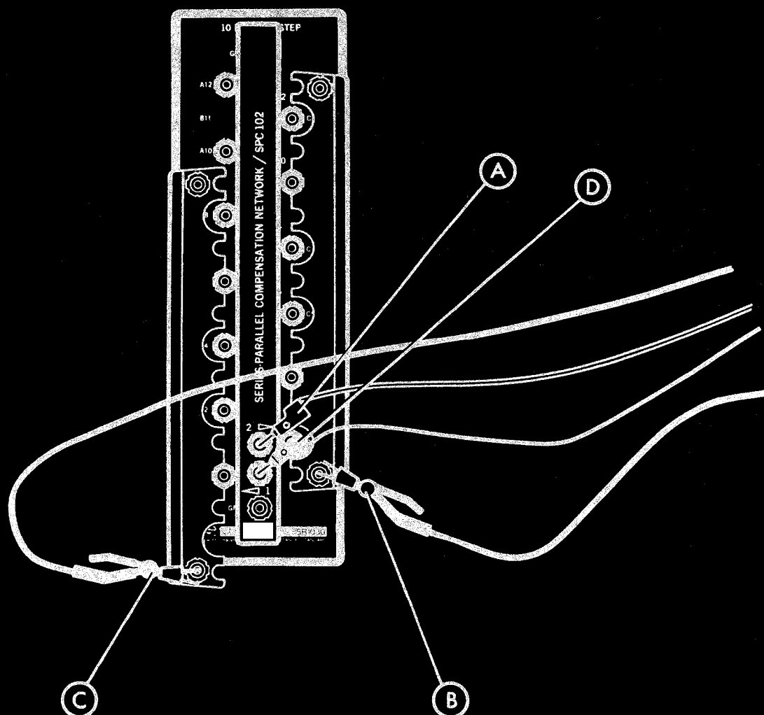
Figure 5-16. Lead Connections to SR1030 Series Parallel Set Up
