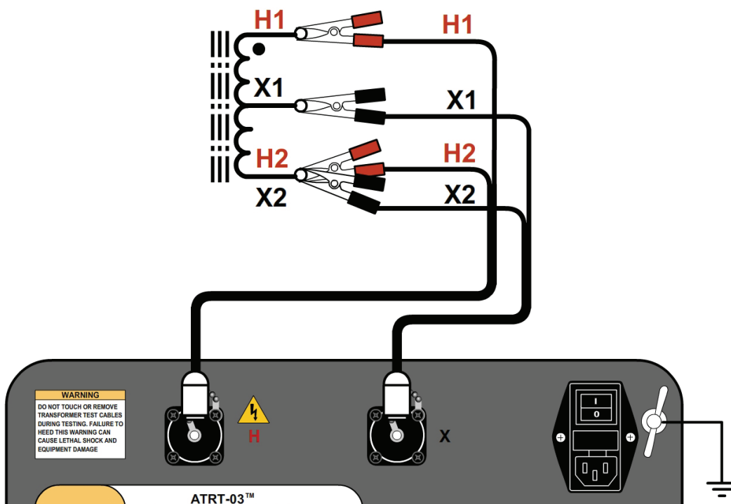
Figure 8. Typical Connections to a Single Phase Auto Transformer
