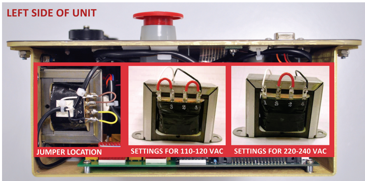
Figure 4. Voltage Selection Jumper Location and Settings
