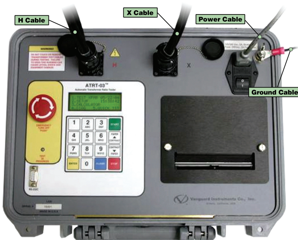
Figure 5. Typical Front Panel Cable Connections
