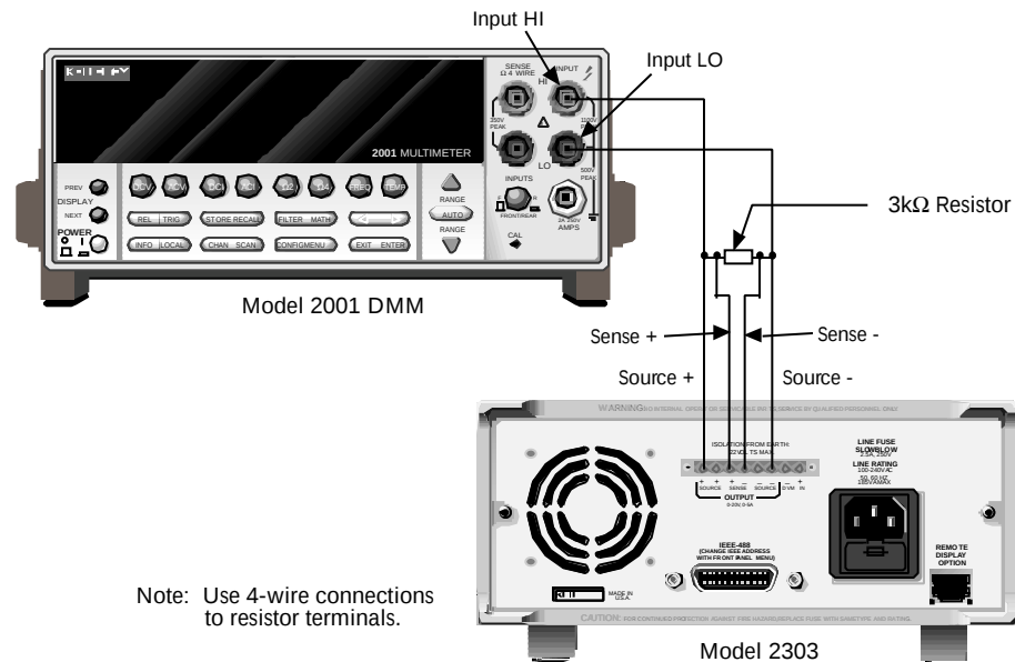
Figure 1-4 Connections for Model 2303 and 2303B 5mA current verification tests
