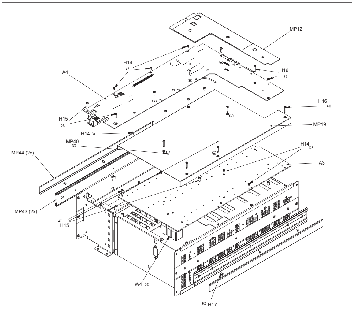
Figure 29. Replacement Parts (cont.)
