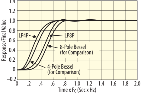
LP8P and LP4P Step Response
