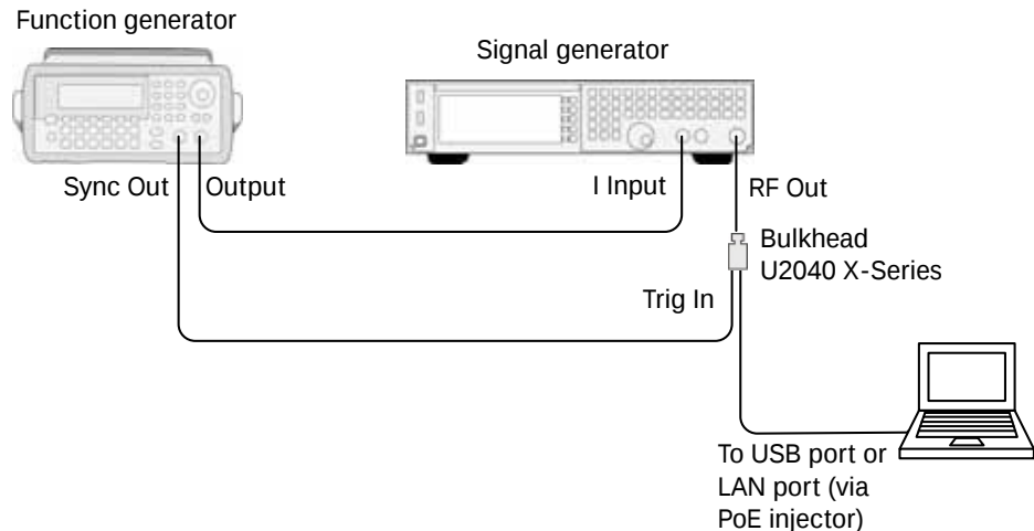
Figure 2-7 Equipment setup for rise time verification
