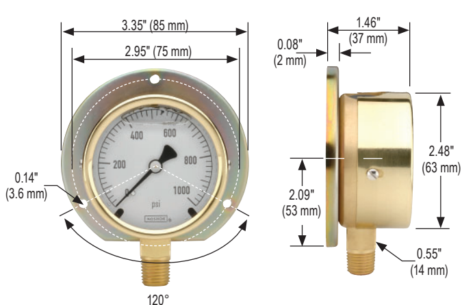
25-300 Rear Flange
