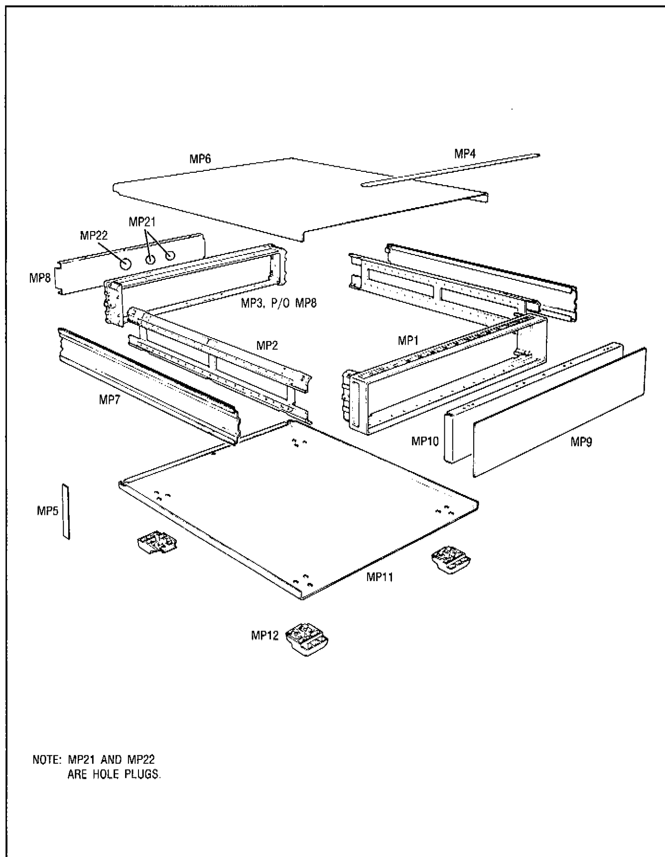
Figure 6. Cabinet Parts
