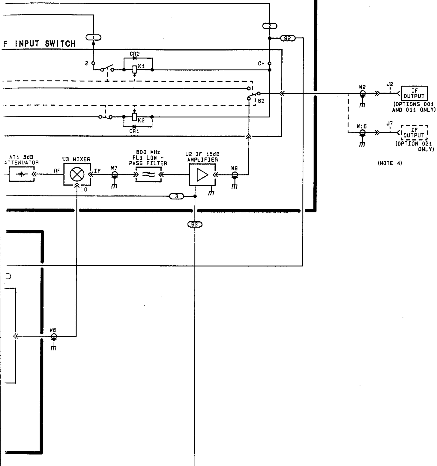
SS2 Figure 12. INPUT SIGNAL DOWN CONVERTER (Schematic Diagram for Options 001, 011, and 021)
