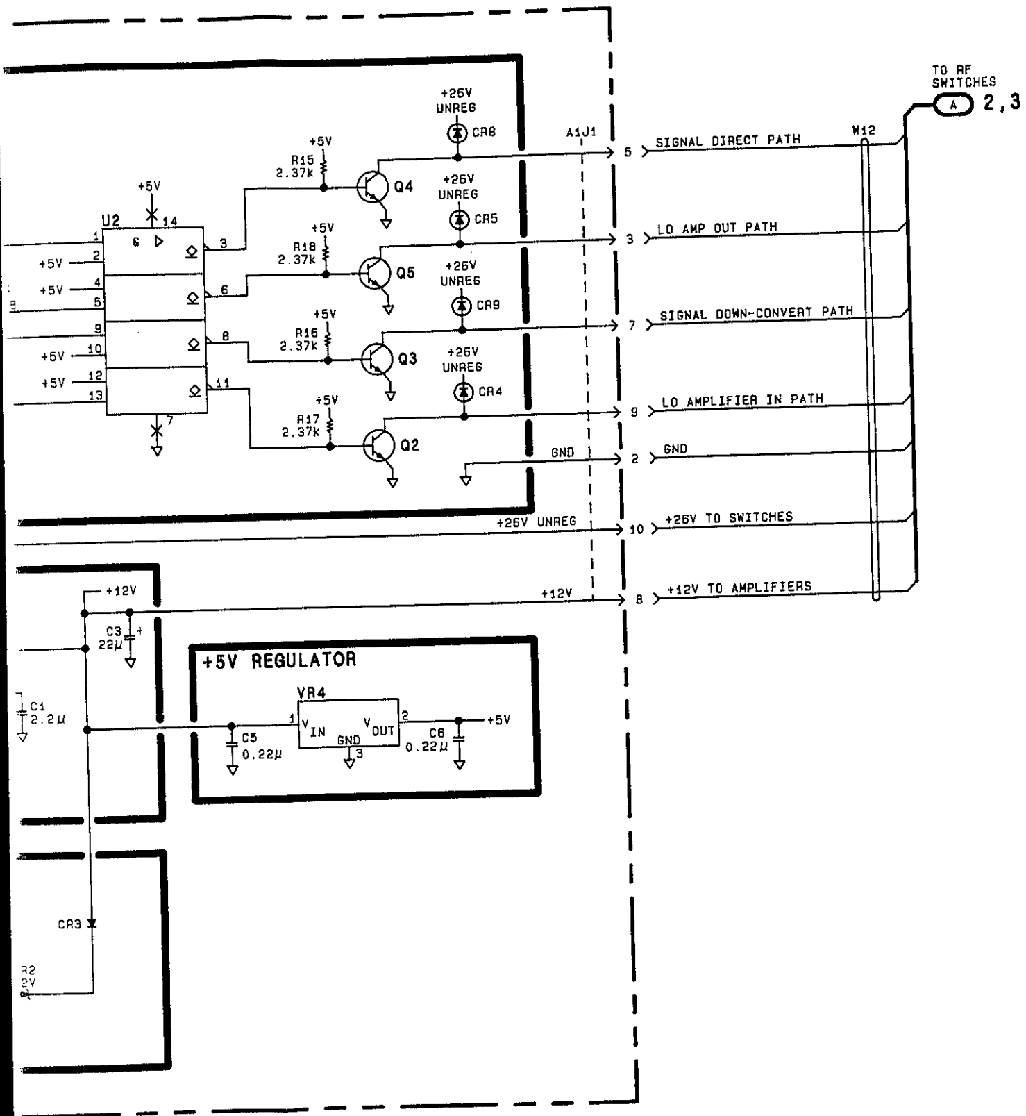
Figure 14. A1 SWITCH CONTROL ASSEMBLY, Schematic Diagram 43/44
