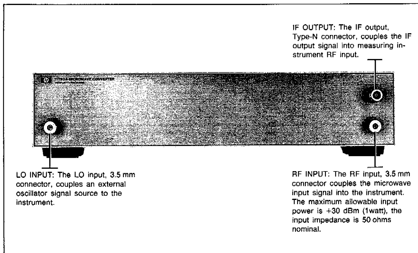
Figure 4. Front-Panel Features
