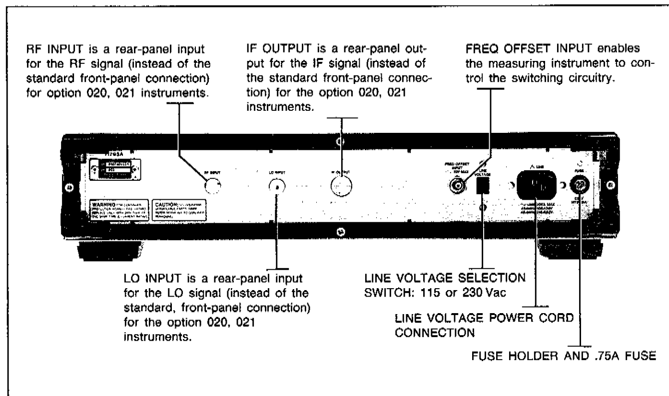
Figure 5. Rear-Panel Features
