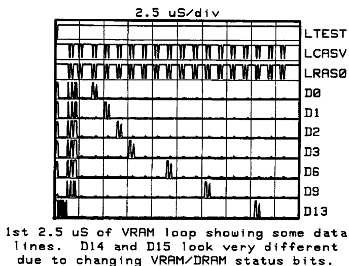
Figure 8-42. VRAM Loop
