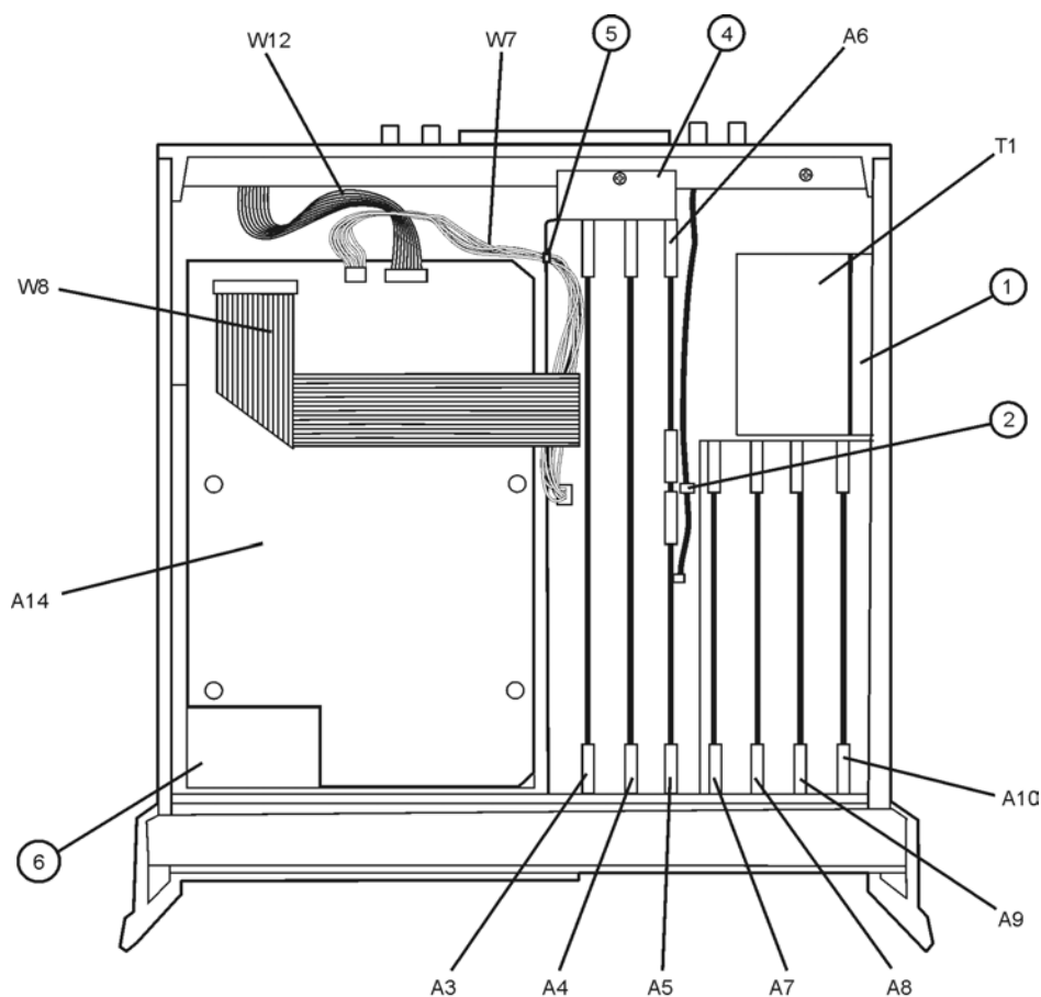
Figure 6-5. Top View
