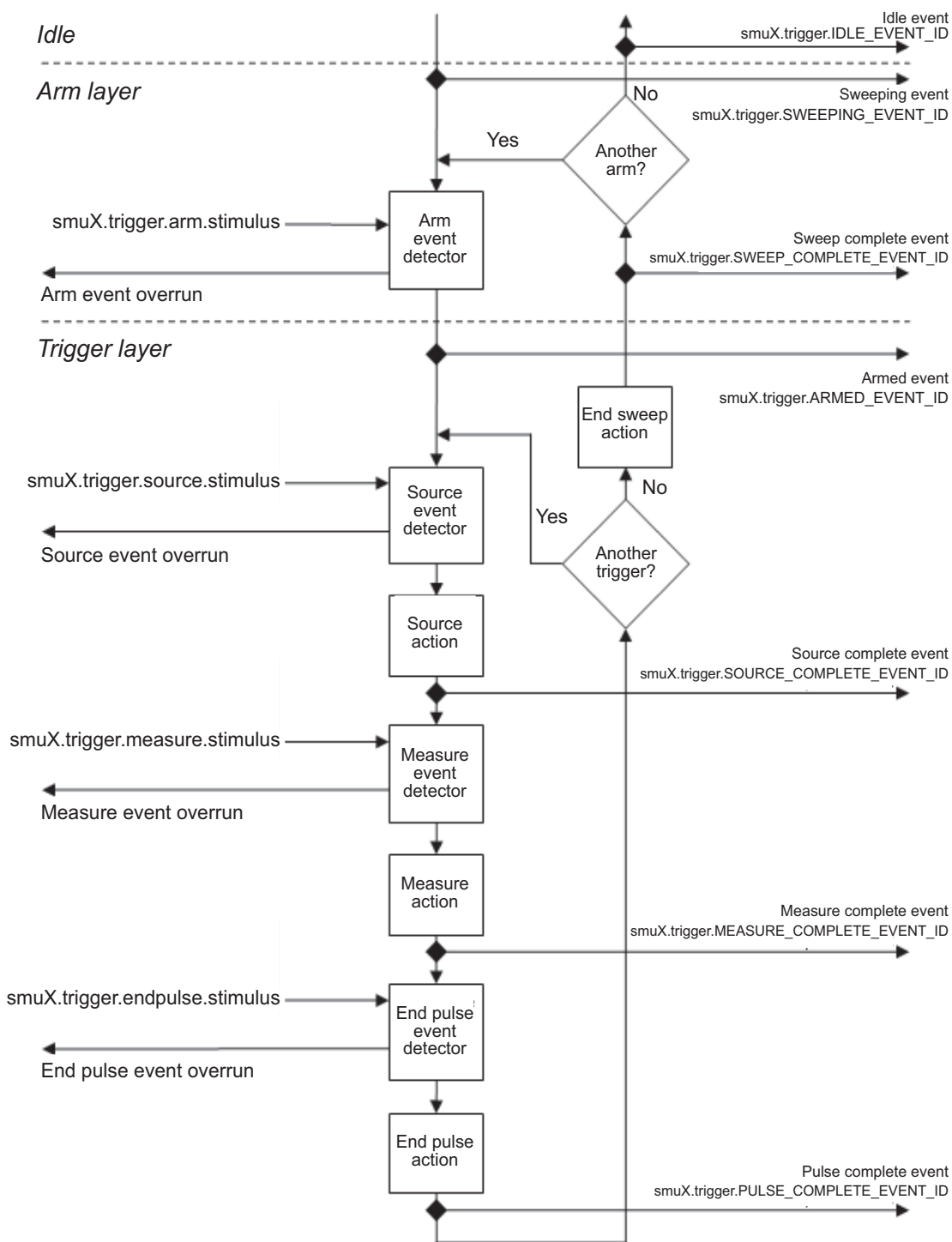
Figure 10-2 Remote trigger model
