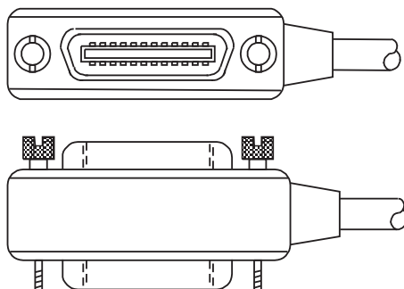
Figure 15-1 IEEE-488 connector
