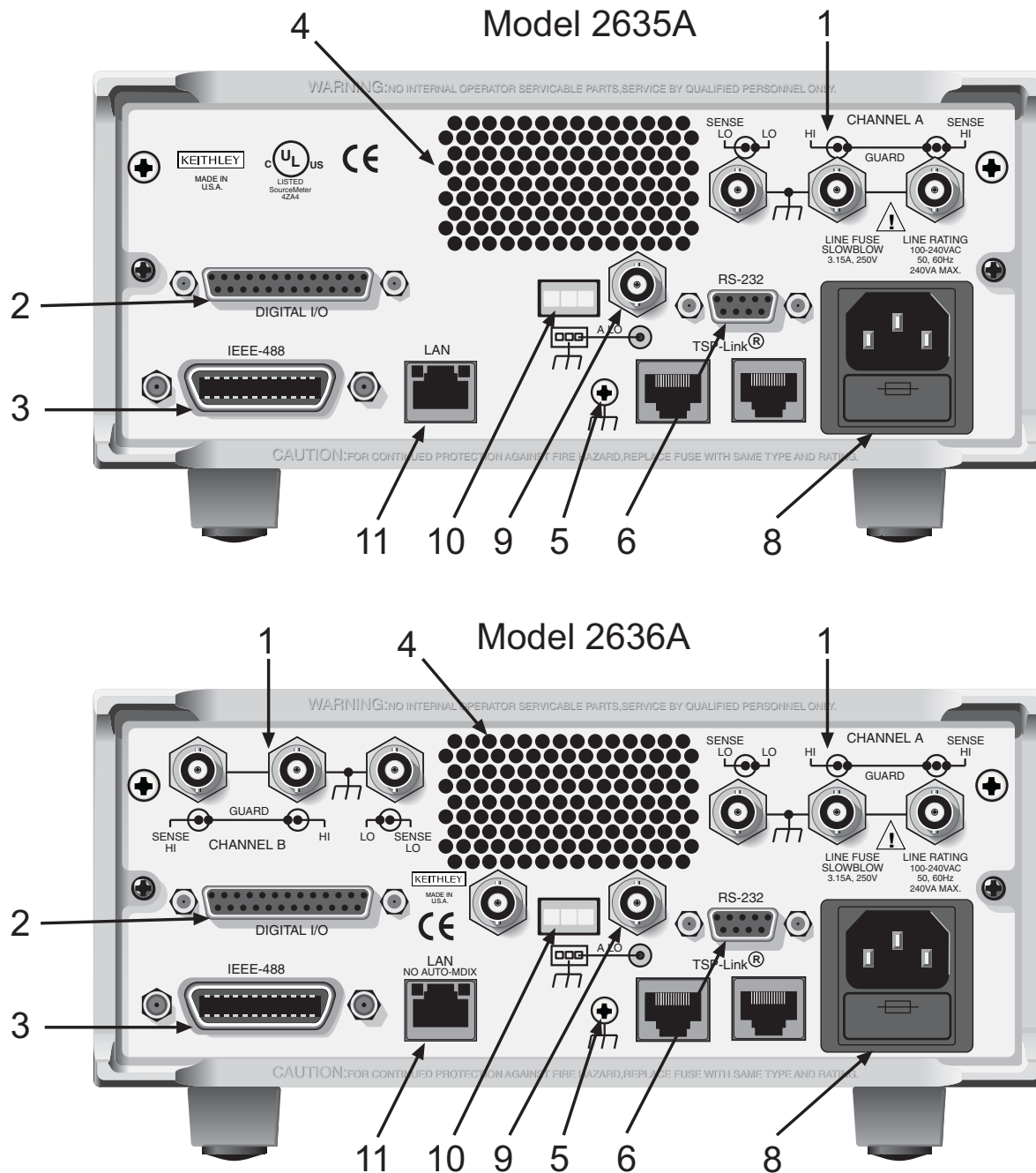
Figure 1-3 Models 2635A/2636A rear panels (see definitions below figure)
