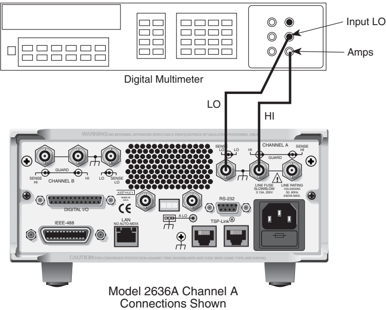
Current verification connections (1uA to 1A ranges)
