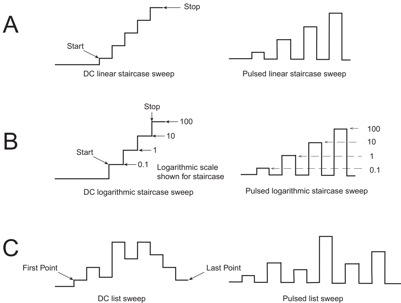
Figure 9-1 Sweep types
