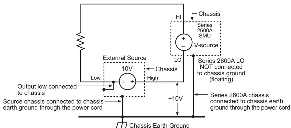
Figure 2-31 Floating the Series 2600A
