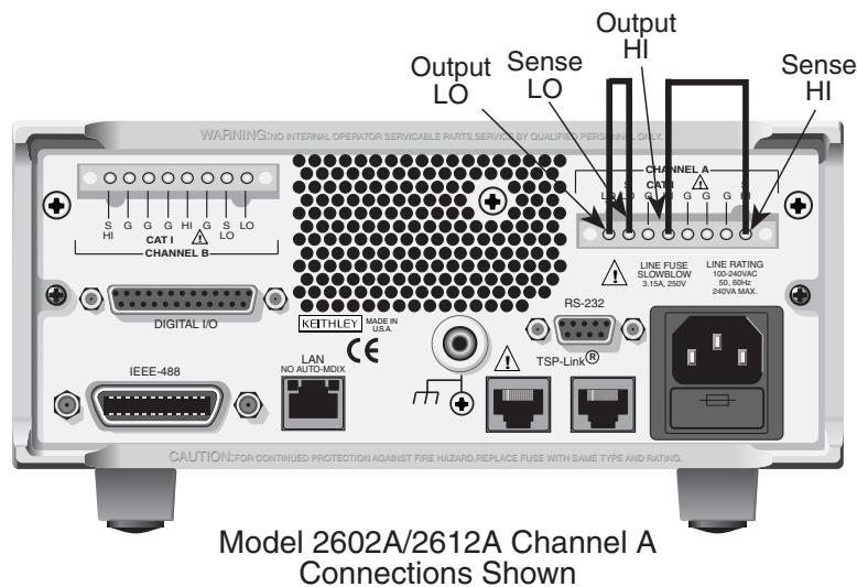
Figure 20-4 Connections for contact check 0Ω calibration
