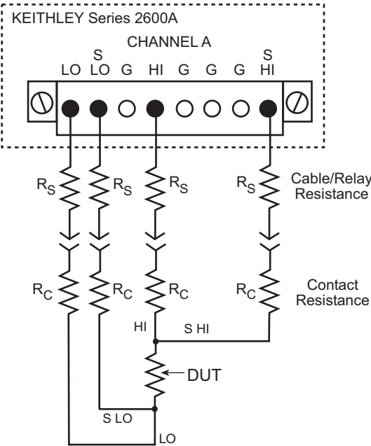
Figure 3-5 Contact check measurements
