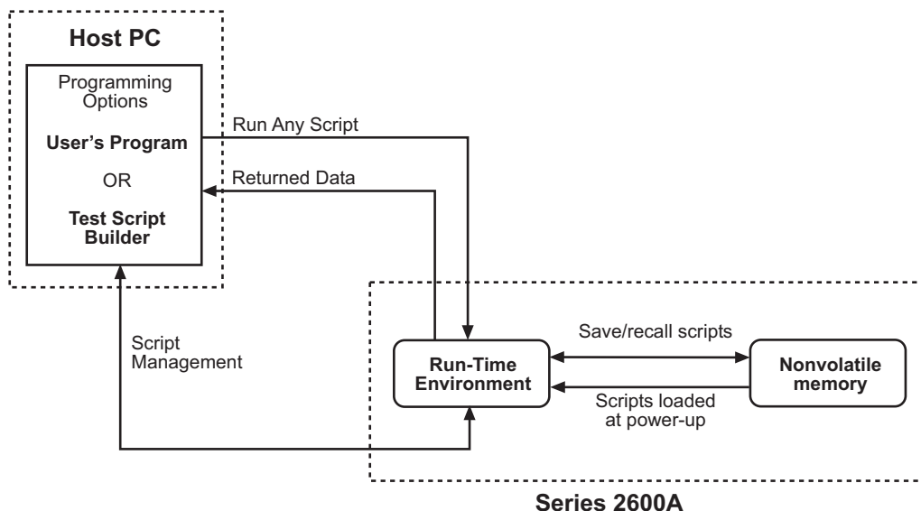
Programming model for scripts
