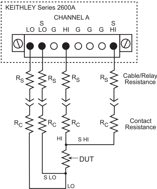
Figure 2-12 Contact check connections
