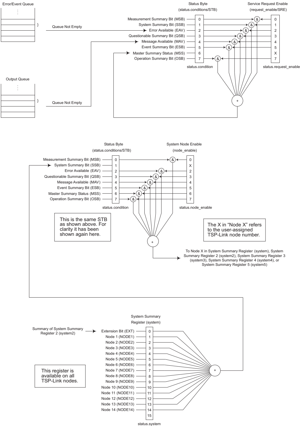
Figure C-1 Status model overview
