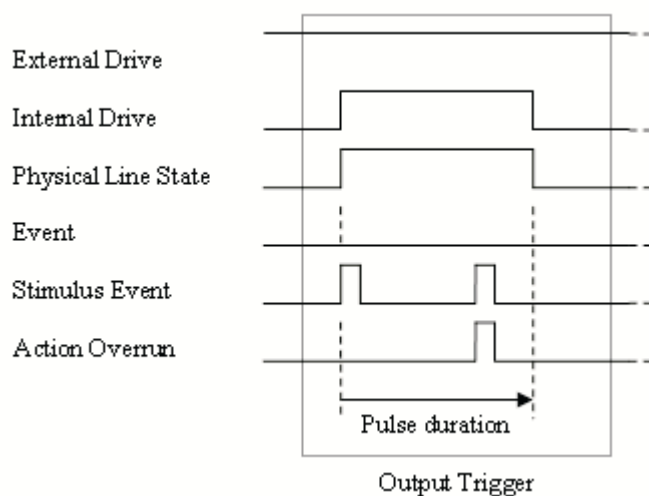
Figure 10-13 RisingM output trigger
