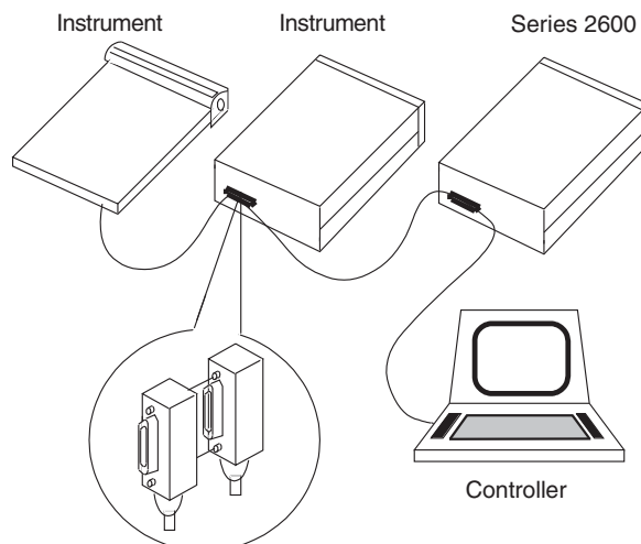
Figure 15-2 IEEE-488 connections
