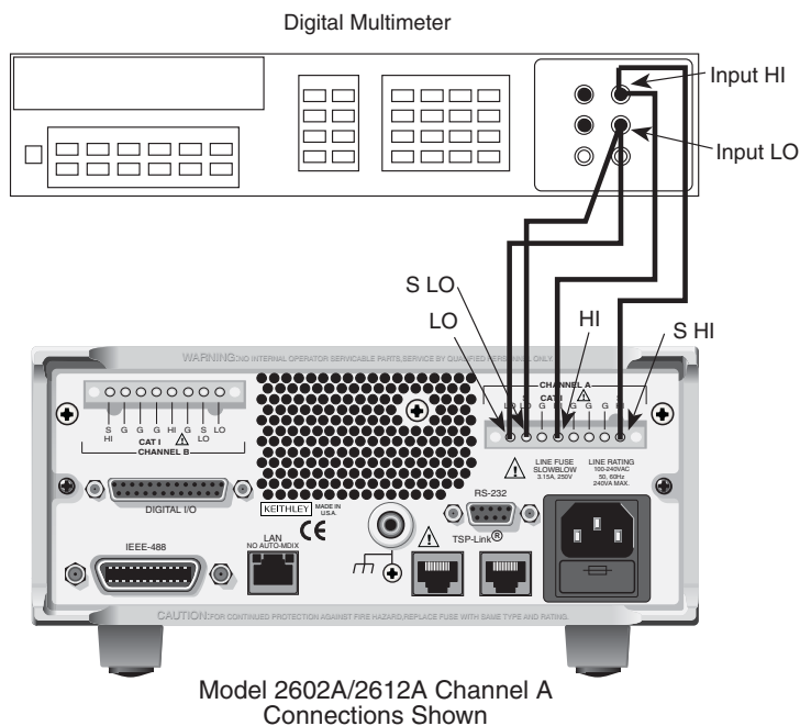
Figure 22-1 Connections for voltage verification
