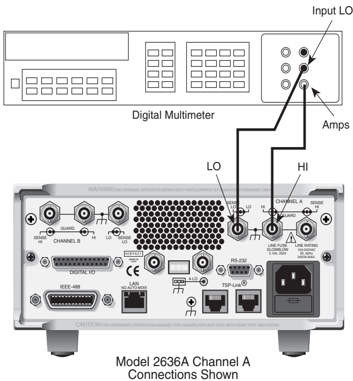
Connections for current calibration (1uA to 1A ranges)
