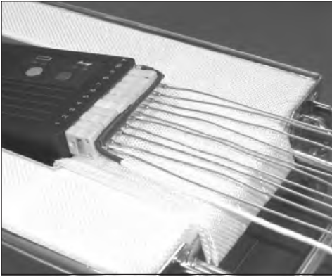
Trpaq21 logger with TX2040A antenna correctly routed across thermocouple plugs.
