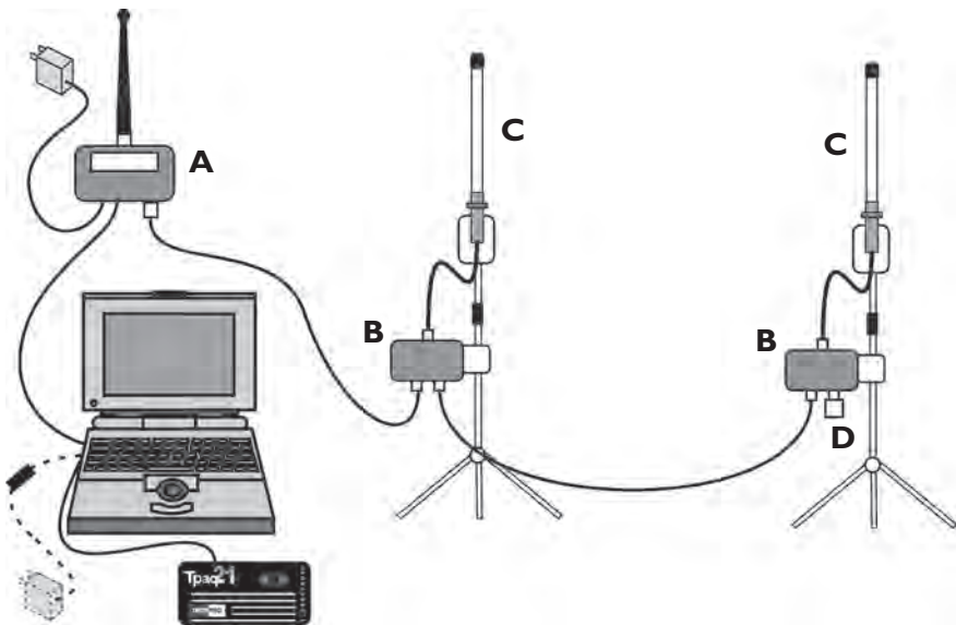
The setup for a TM21 radio-telemetry system with multiple receivers : primary receiver (A) with whip antenna, and two secondary receivers (B) attached to unity-gain end-feed antennas (C). Further secondary receivers may be added. The receiver at the end of the chain is fitted with a terminator (D). Such a system may be suitable for, e.g., a long continuous furnace.
