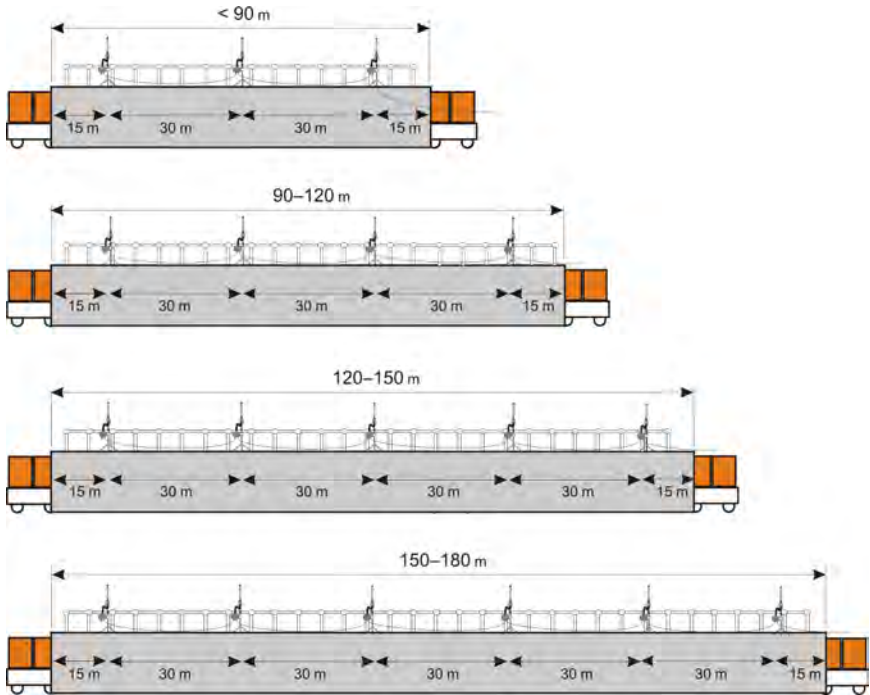
Recommended numbers of antennas, and antenna spacing, for steel-clad kilns of different lengths.
