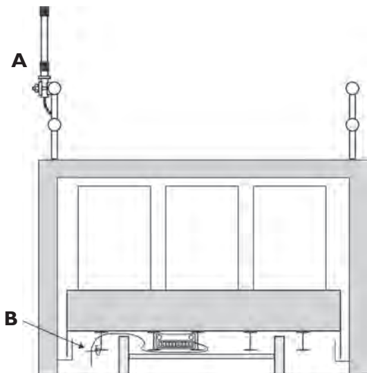
Vertical section through a kiln and kiln car, showing a typical installation of receiver antennas (A, one shown) on the kiln's handrail, and transmitter antenna (B) below the kiln car. Receiver and transmitter antennas must be on the same side of the kiln.
