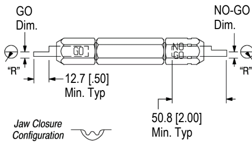
Suggested Plug Gage Design for Wire Barrel Section of Crimping Chamber
