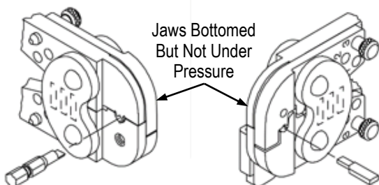
Inspection of Wire Barrel Section of Crimping Chamber
