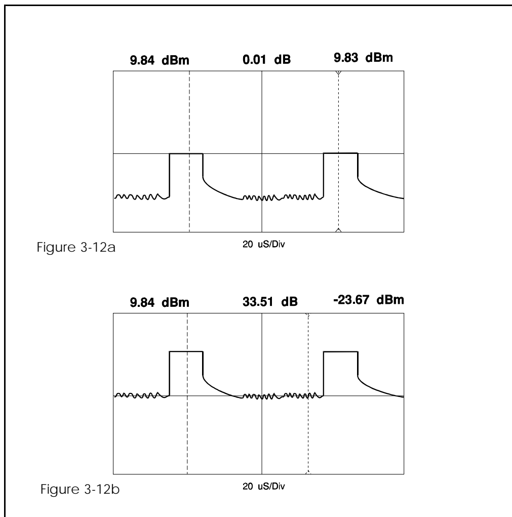
Figure 3-12. Using Mark >Set Vertical Center
