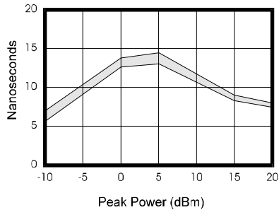
*Typical Risetime in High Bandwidth Mode
