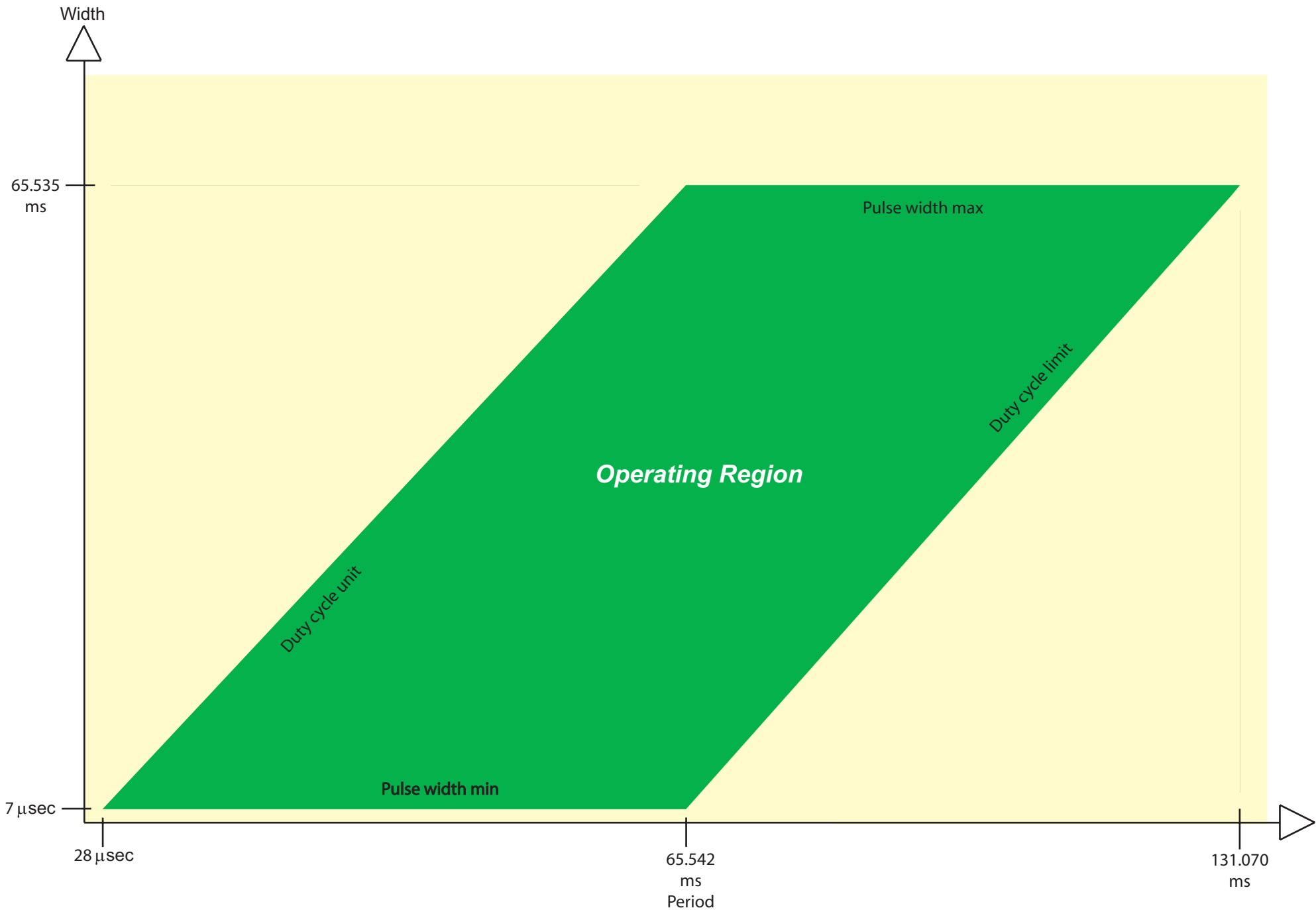
1GHz Calibrator Pulse Generator Range (Variable Mode)
