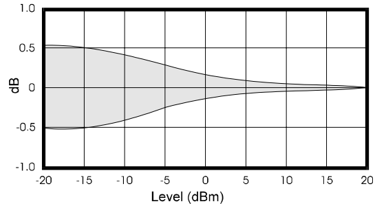
Temperature Influence (±4° from calibration)
