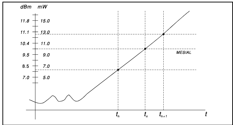
Figure 6-6. Time Interpolation
