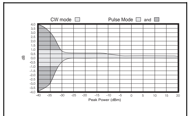
Temperature Influence (±4° from calibration)
