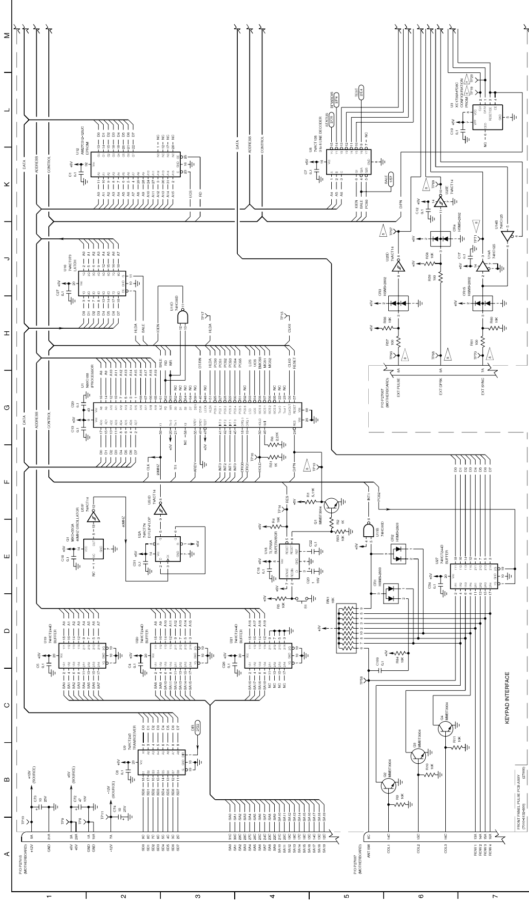
Figure 41 Front Panel Pulse PCB Assy (Sheet 8 of 11) (Circuit Schematic - Sheet 5 of 8)
