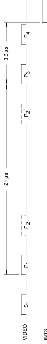
MODE C ALL CALL with S 1 PULSE (with or without SLS)
