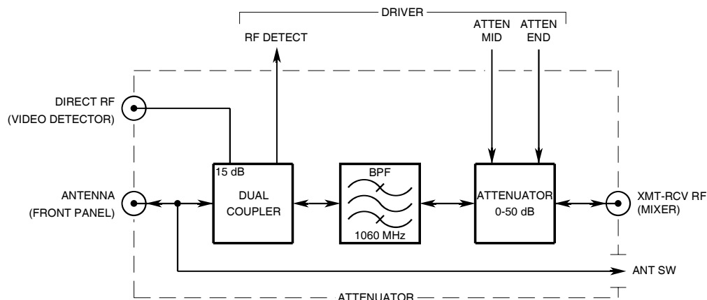
Attenuator PCB Assy Block Diagram Figure 9
