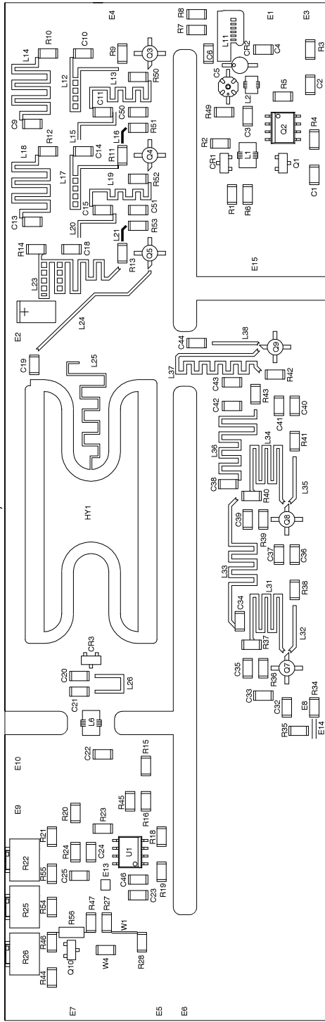
TOP VIEW
