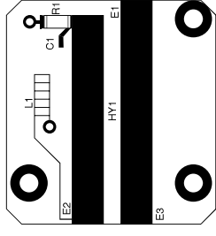
POWER TERMINATION PCB ASSY DETAIL A
