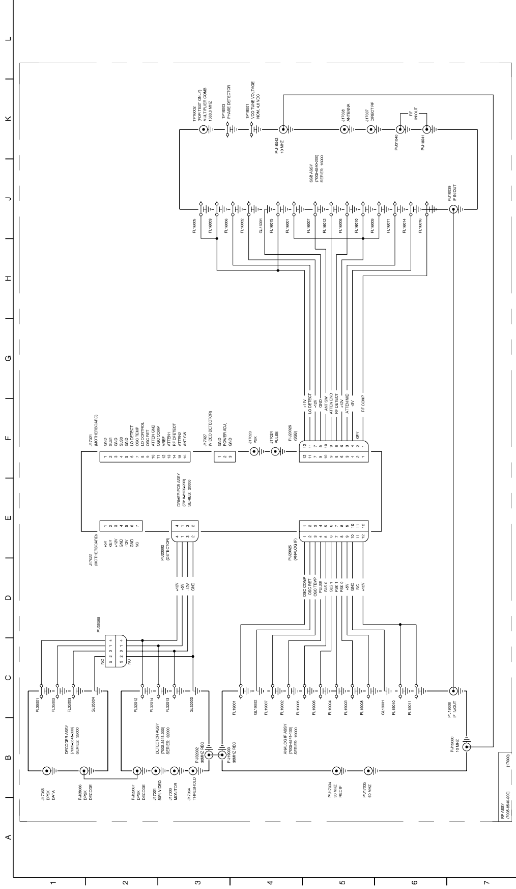
Figure 42 RF Assy (Sheet 2 of 23) (Interconnect Diagram)
