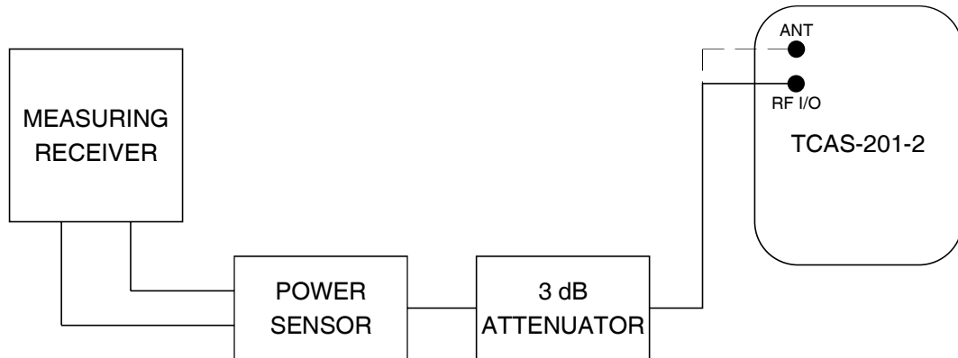
Level and Attenuation Test Setup Diagram Figure 19
