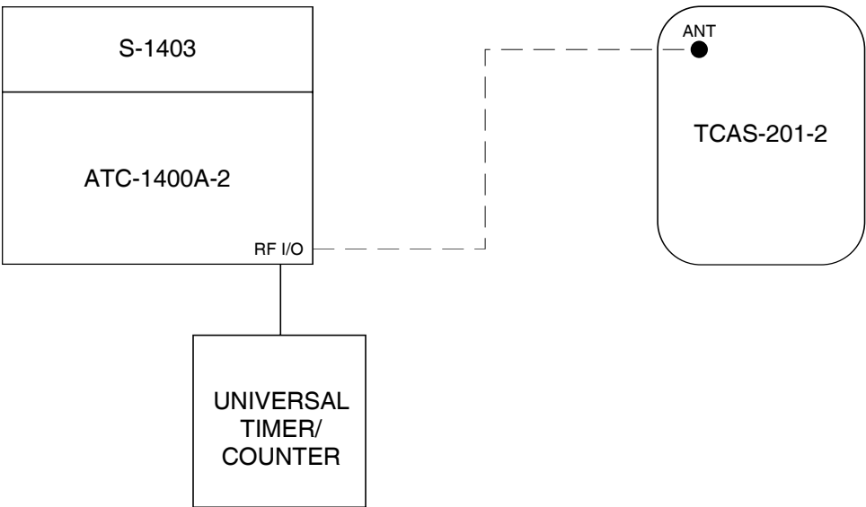
Frequency Measurement Test Setup Diagram Figure 23
