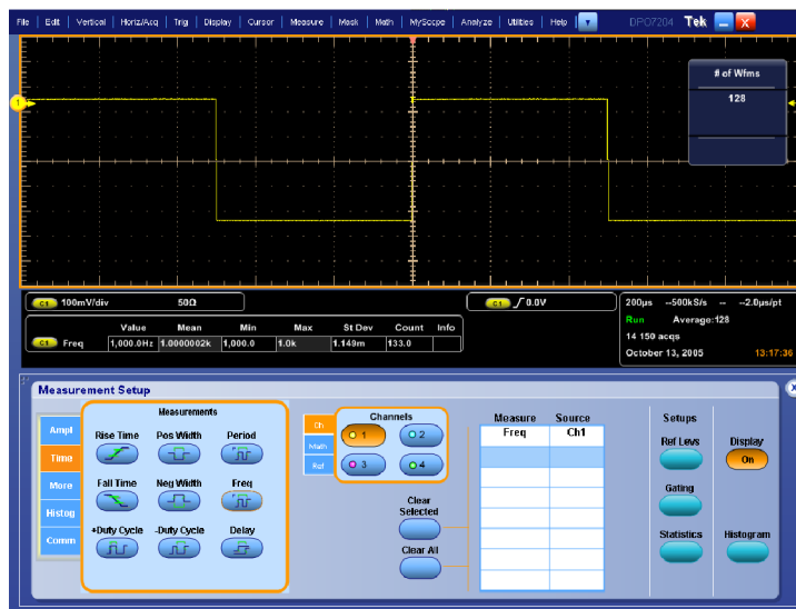
Figure 2-30: Measurement of probe compensator frequency
