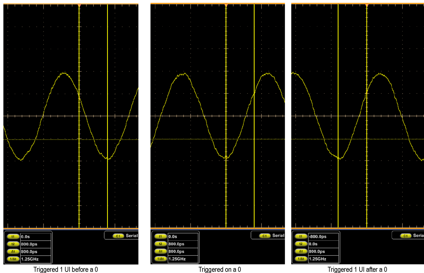
Figure 2-34: Isolated 0 triggering
