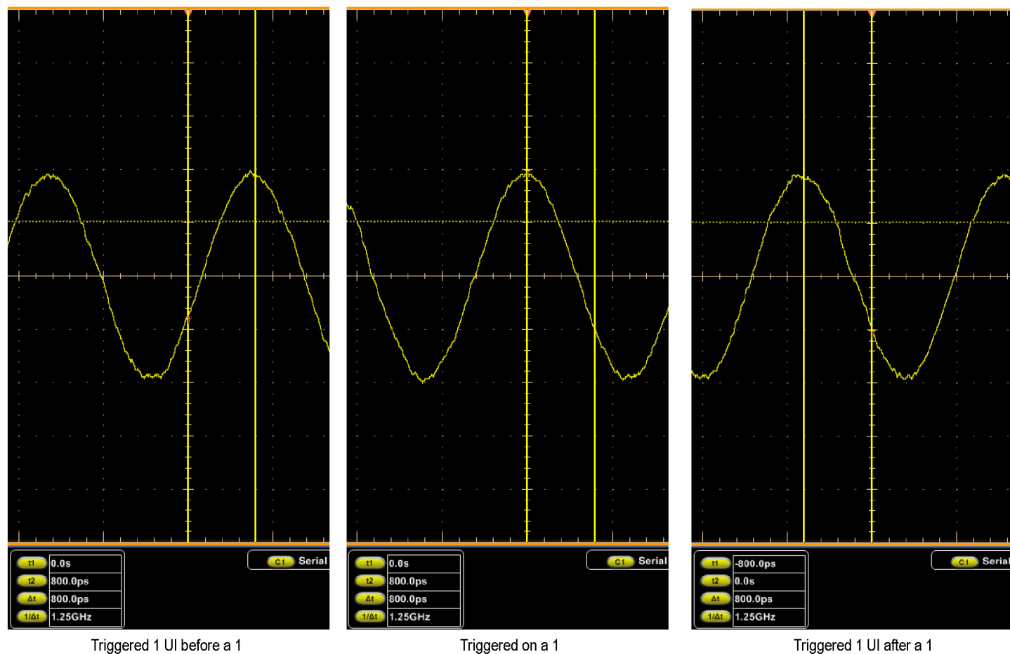
Figure 2-35: Isolated 1 triggering
