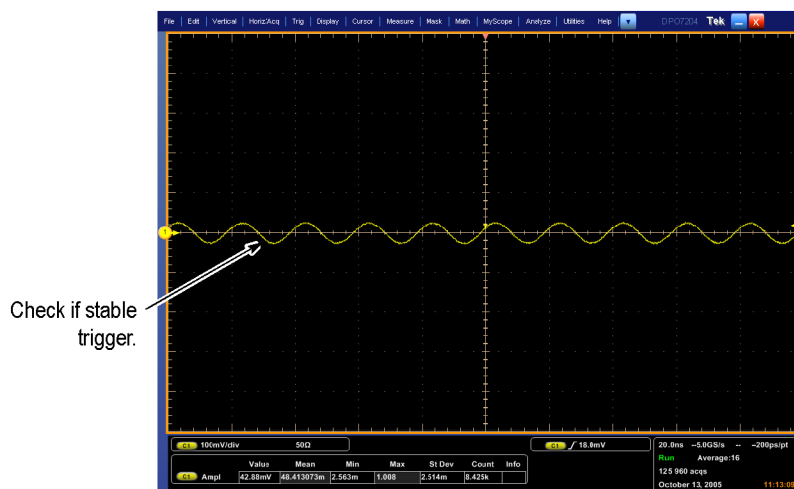
Figure 2-26: Measurement of trigger sensitivity - 50 MHz results shown
