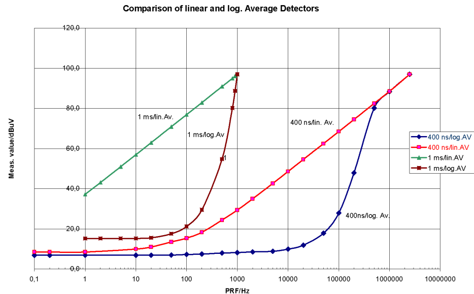
Fig. 4.2 Responses of the linear and the logarithmic average detectors as a function of pulse repetition frequency (PRF) for pulse-modulated signals with pulse durations of 400 ns and 1 ms. Resolution bandwidth is 1 MHz.
