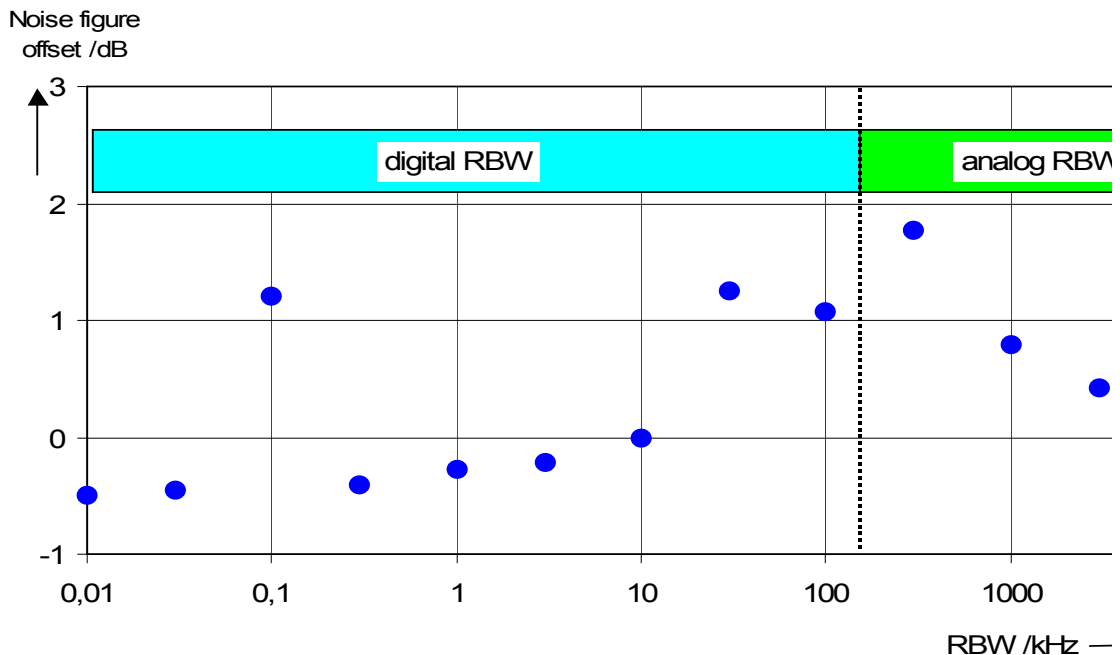
Fig. 2.8 Change in R&S FSG noise figure at various bandwidths. The reference bandwidth is 10 kHz
