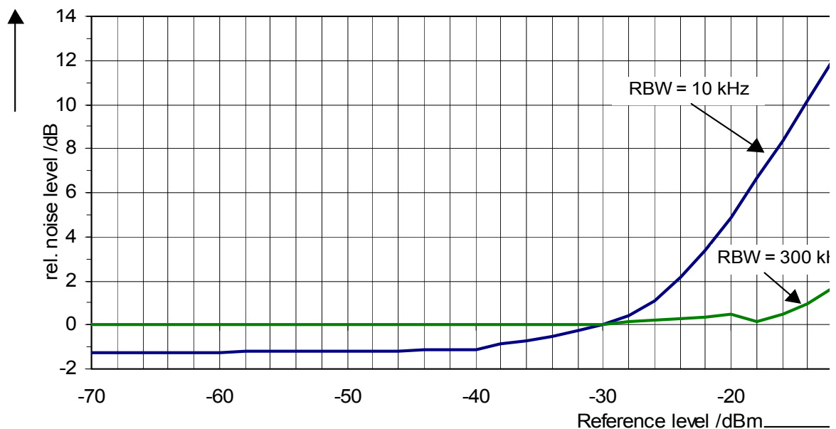
Fig. 2.7 Change in displayed noise as a function of the selected reference level at bandwidths of 10 kHz and 300 kHz (-30 dBm reference level)
