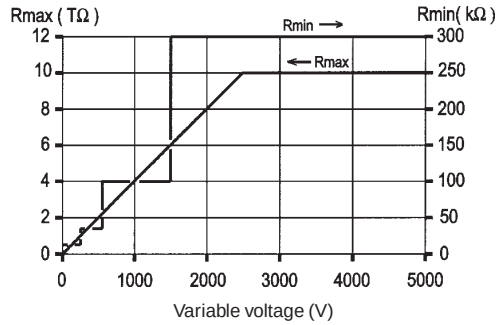
Resistance range in voltage mode
