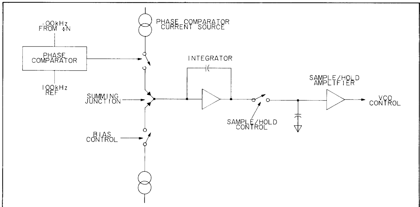
Figure 8-7. Phase Detector.
