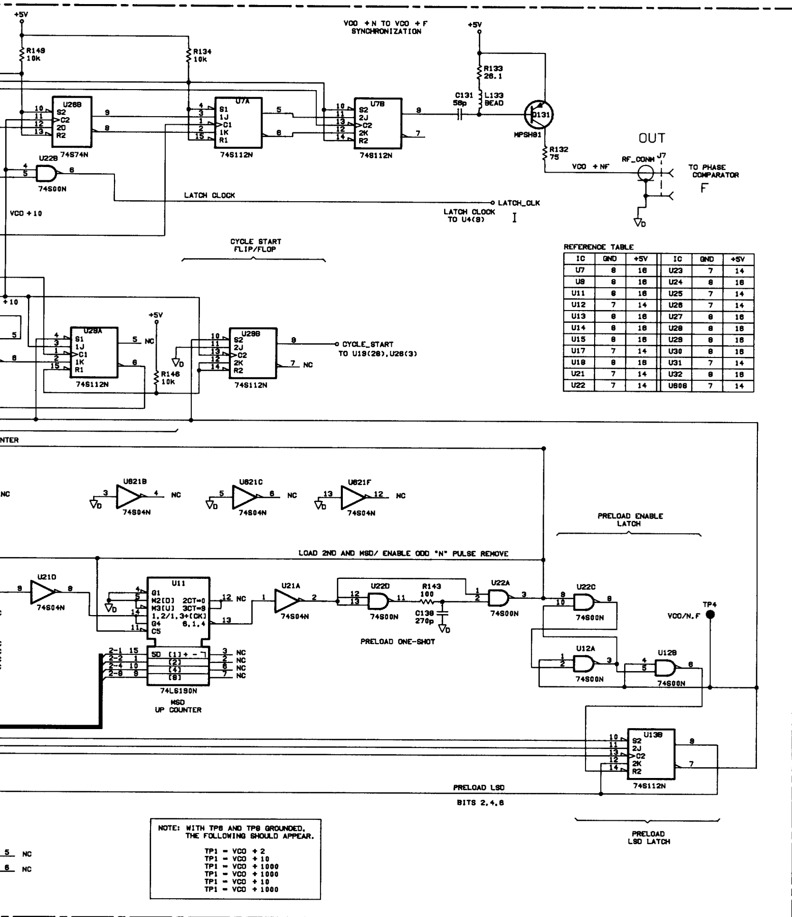
Figure 8-E-1. ÷ N.F. Counter, A21. 8-E-3/8-E-4
