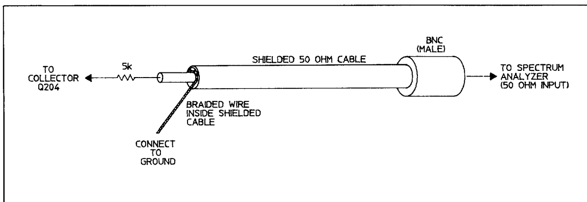
Figure 8-K-1. Gain Stage High Frequency Troubleshooting Probe.
