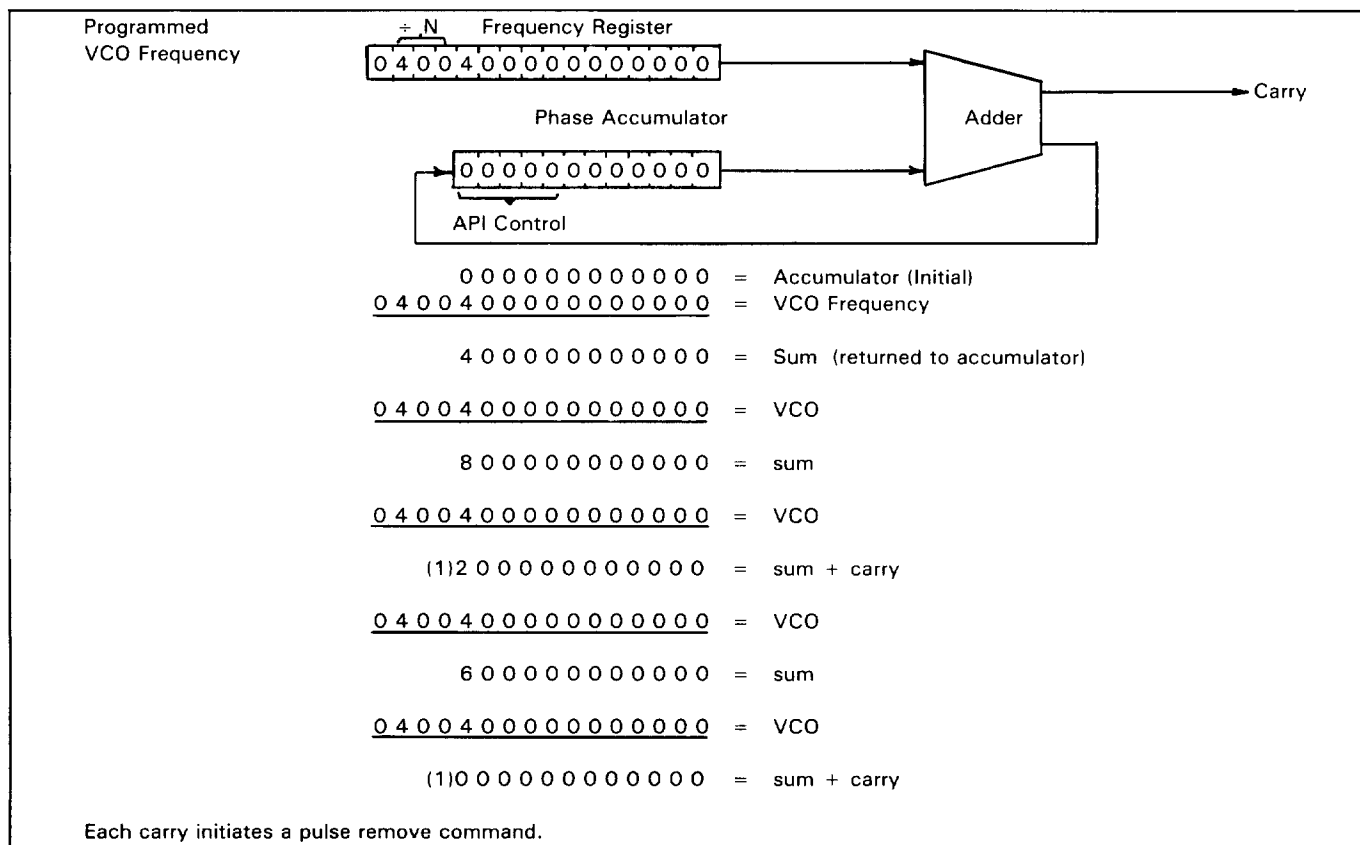
Figure 8-10. Phase Accumulation.
