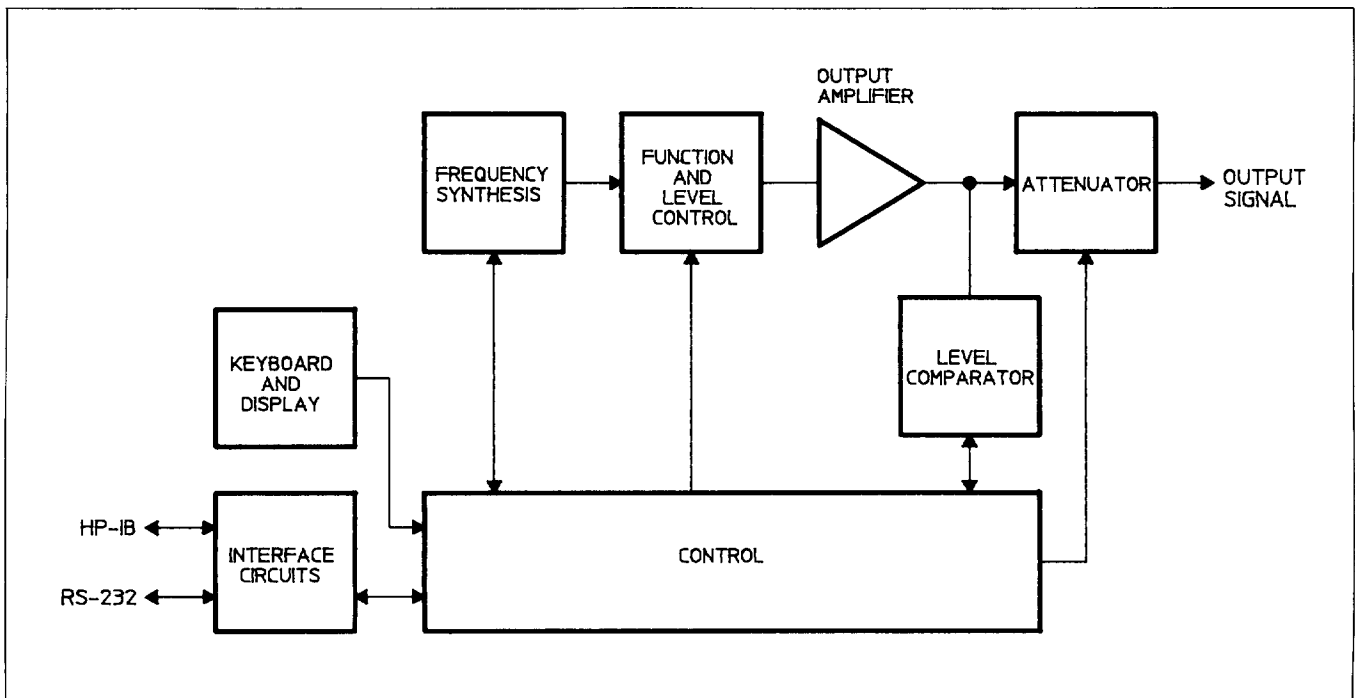
Figure 8-1. Simplified Block Diagram.
