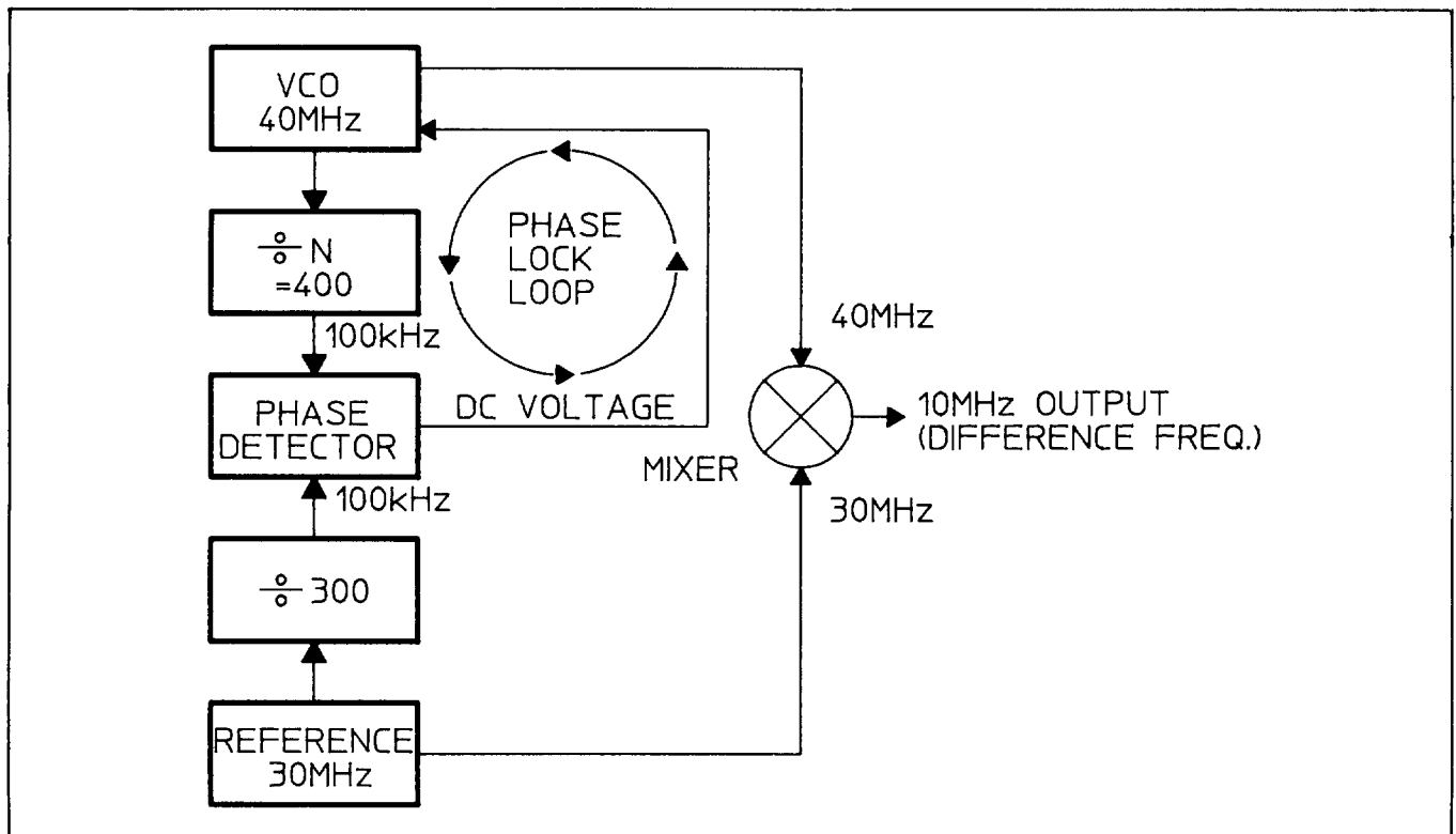
Figure 8-6. Phase Lock Loop.
