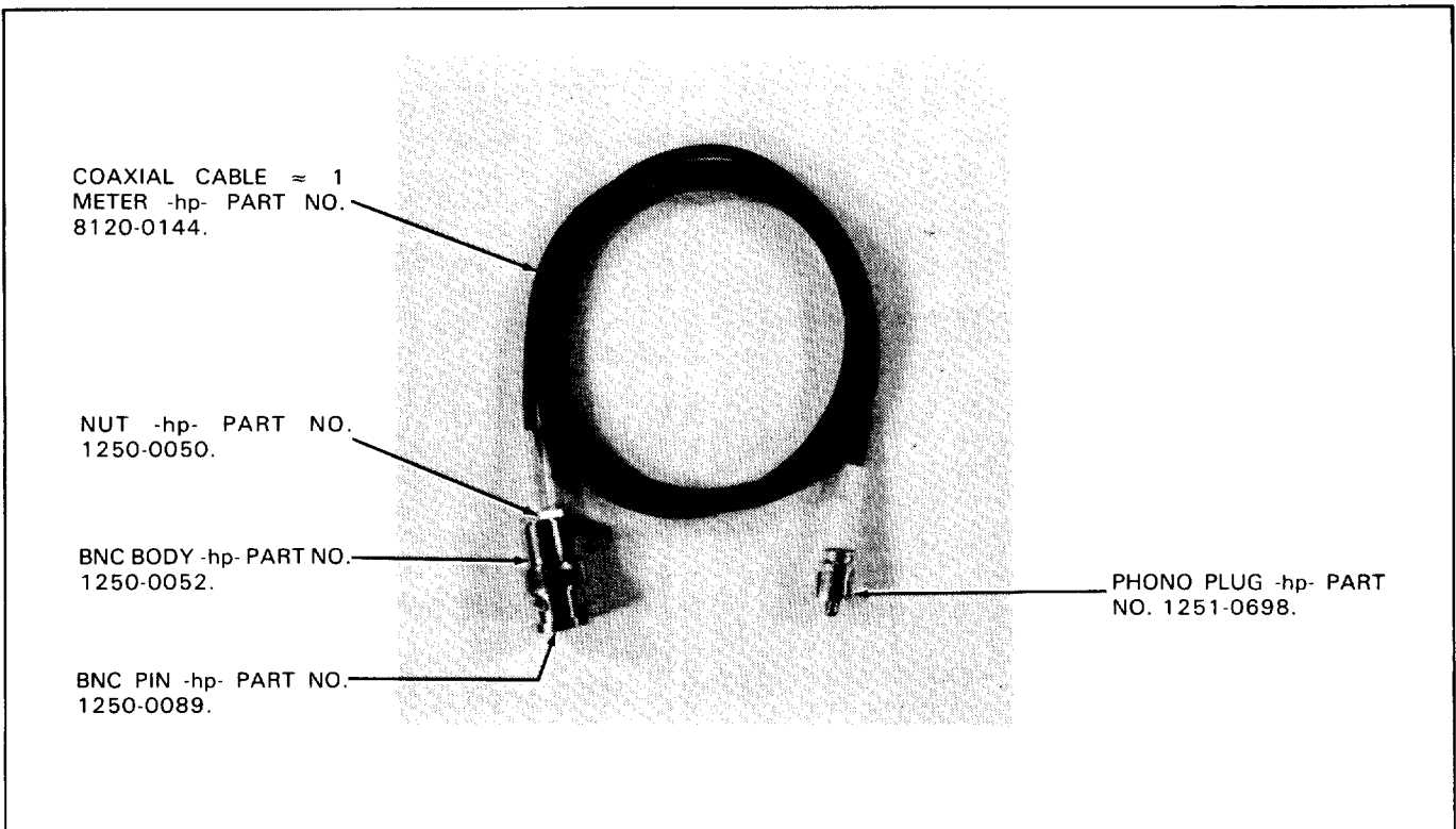
Figure 8-26. Adapter Cable.
