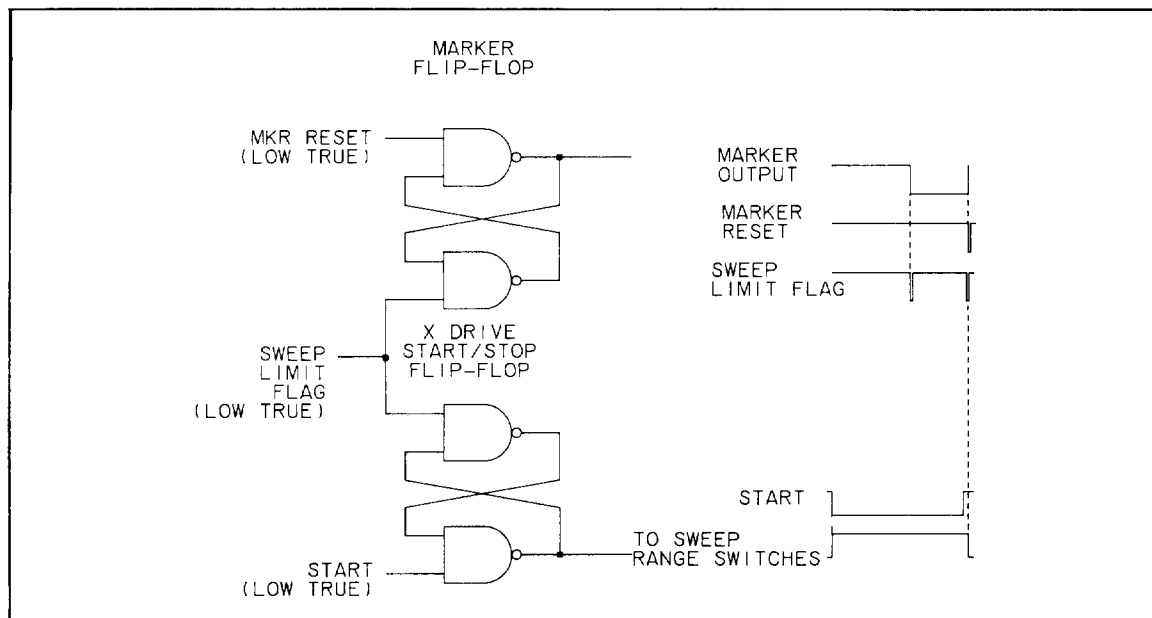
Figure 8-21. Marker and X Drive Start-Stop Flip-Flops.
