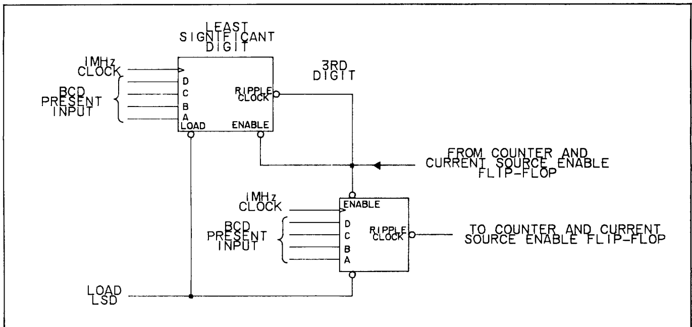
Figure 8-15. Preset Counters.
