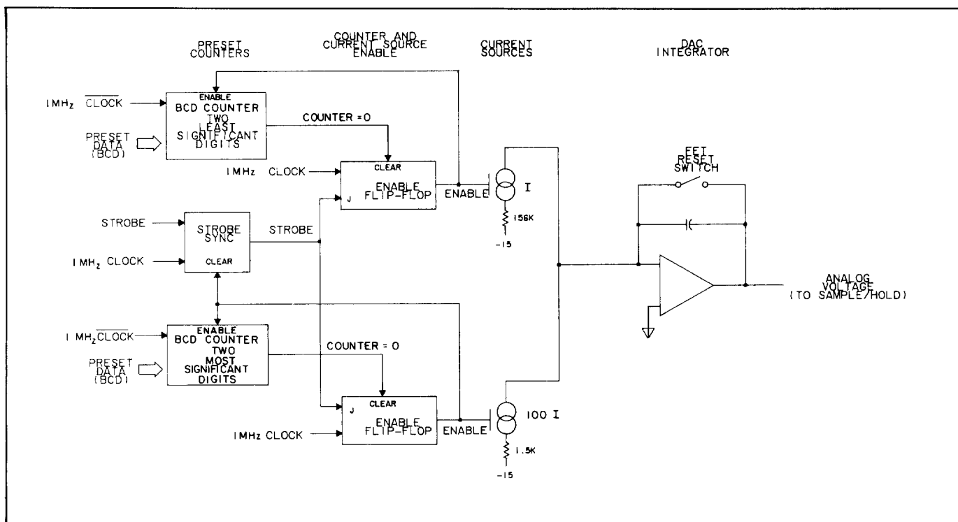
Figure 8-16. Digital-to-Analog Converter.
