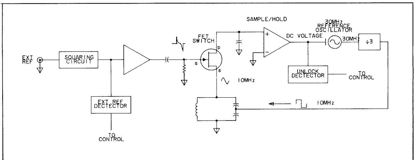
Figure 8-12. External Reference Phase Lock Loop Block Diagram.
