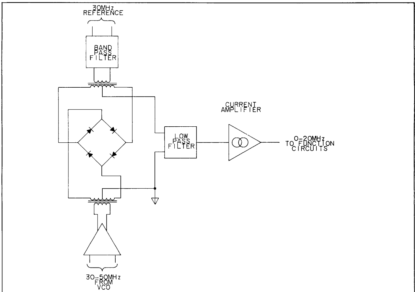
Figure 8-14. Mixer Diagram.
