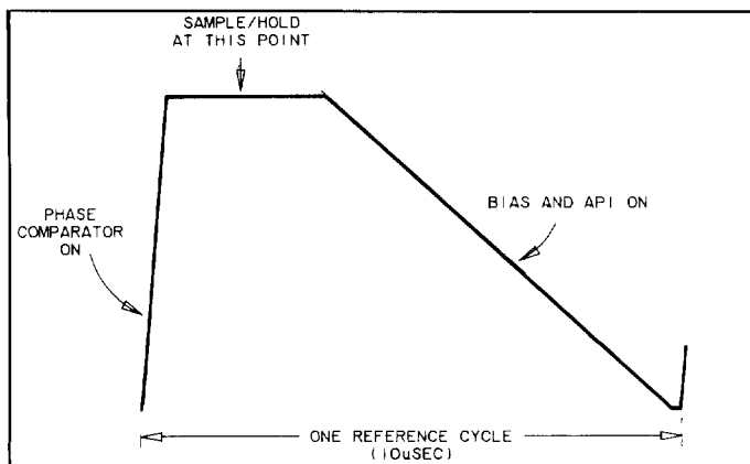
Figure 8-8. Integrator Output.
