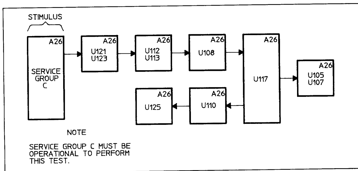
Figure 8-B-1. A26 Assembly SA0 Test Signal Flow Diagram.
