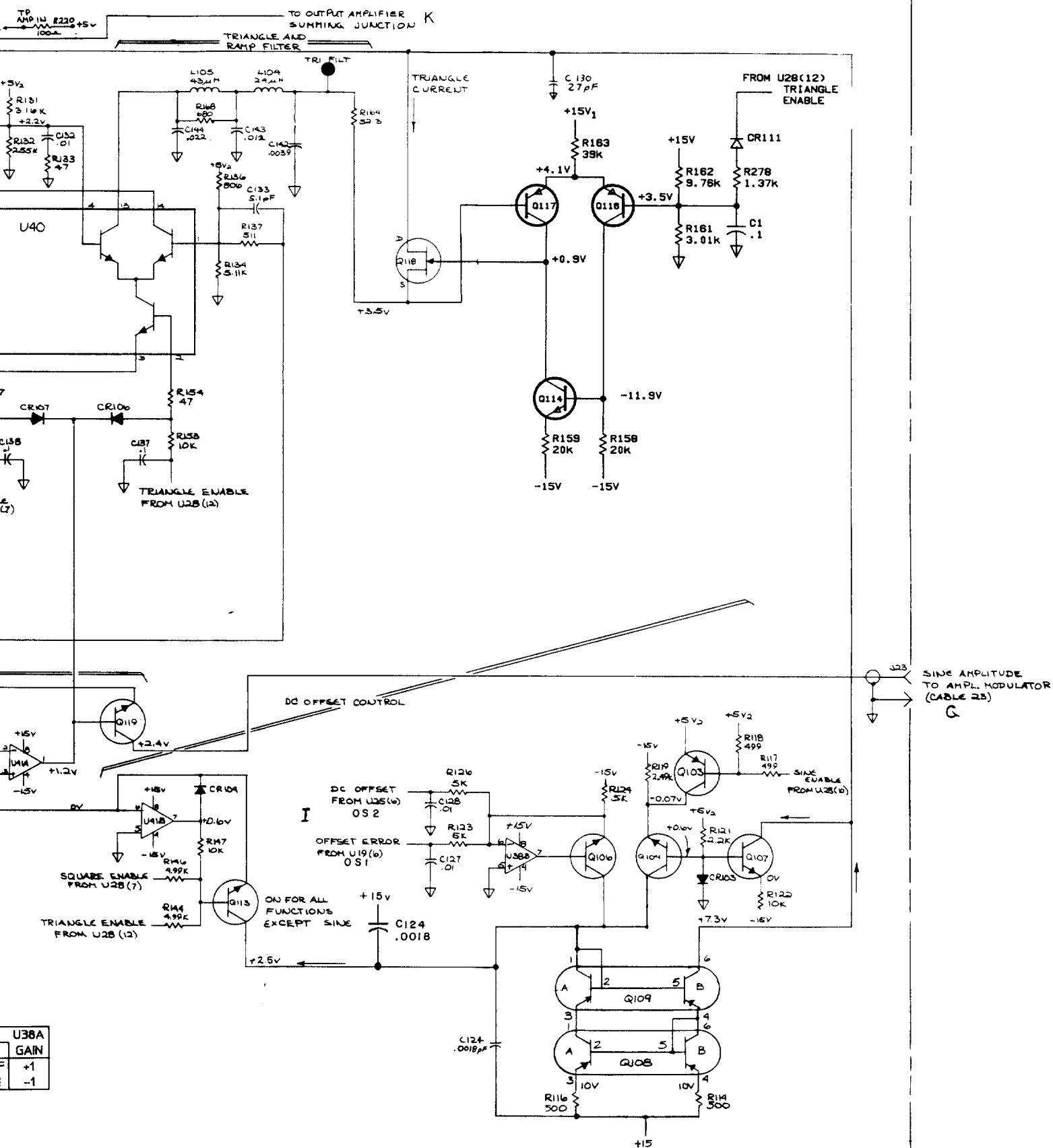
Figure 8-J-3. Function Circuits, A14. 8-J-7/8-J-8
