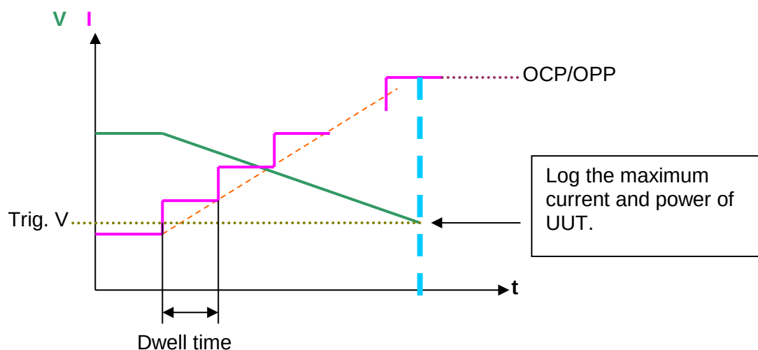
Figure 3-9 OCP/OPP Mode
