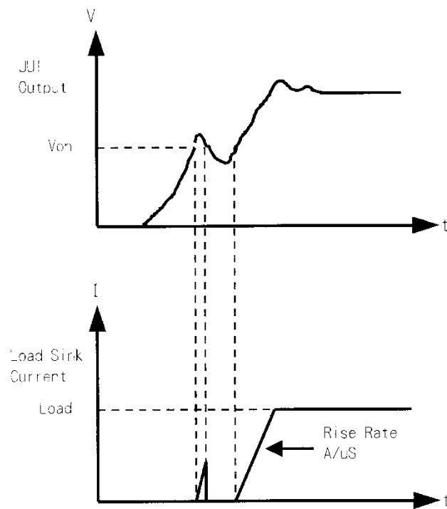
Figure 4-3 Von LATCH OFF Current Waveform
