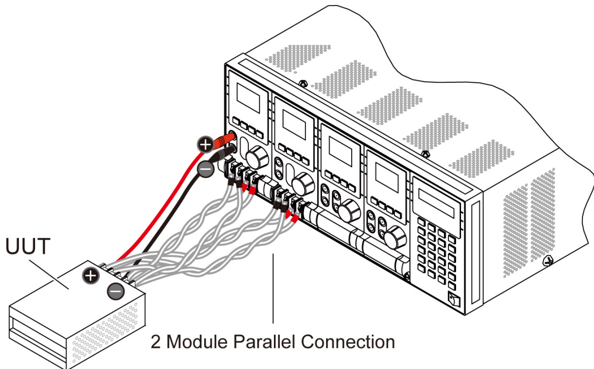
Figure 2-6 Parallel Connection
