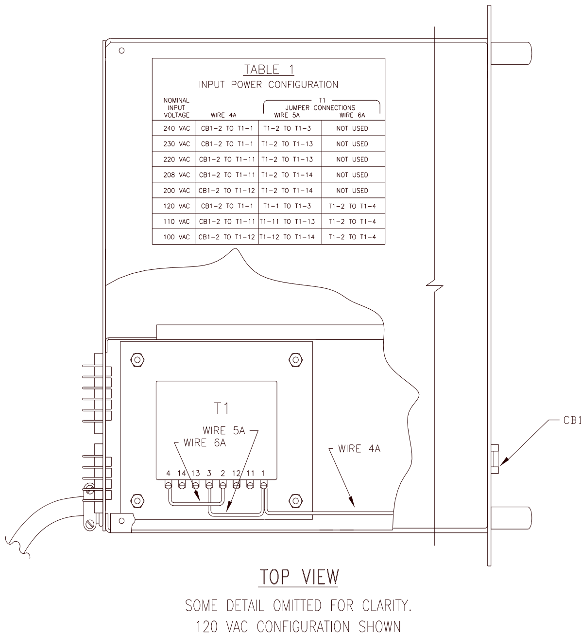
FIGURE 3.3.2 MODELS 120-ASX & 320-ASX INPUT VOLTAGE CONFIGURATION
