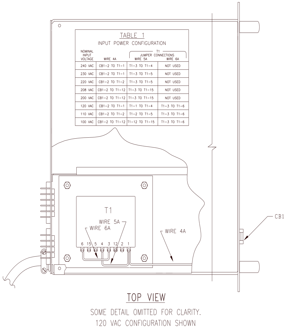
FIGURE 3.3.3 MODEL 315-ASX INPUT VOLTAGE CONFIGURATION
