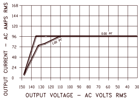
RATING CURVE 1 PHASE MODE
