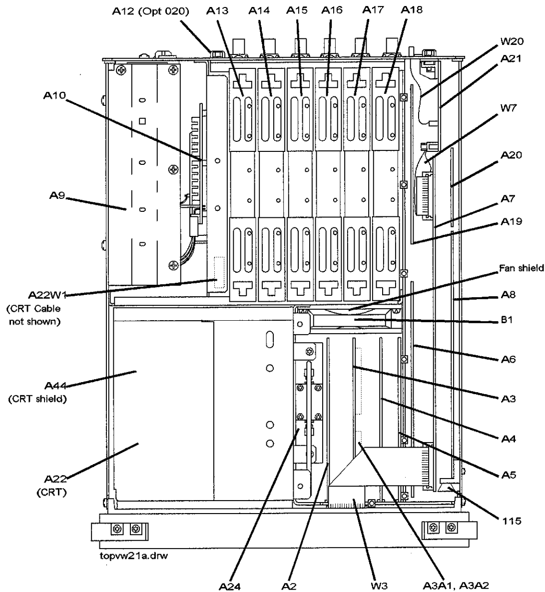
Major Assemblies and Cables, Top View
