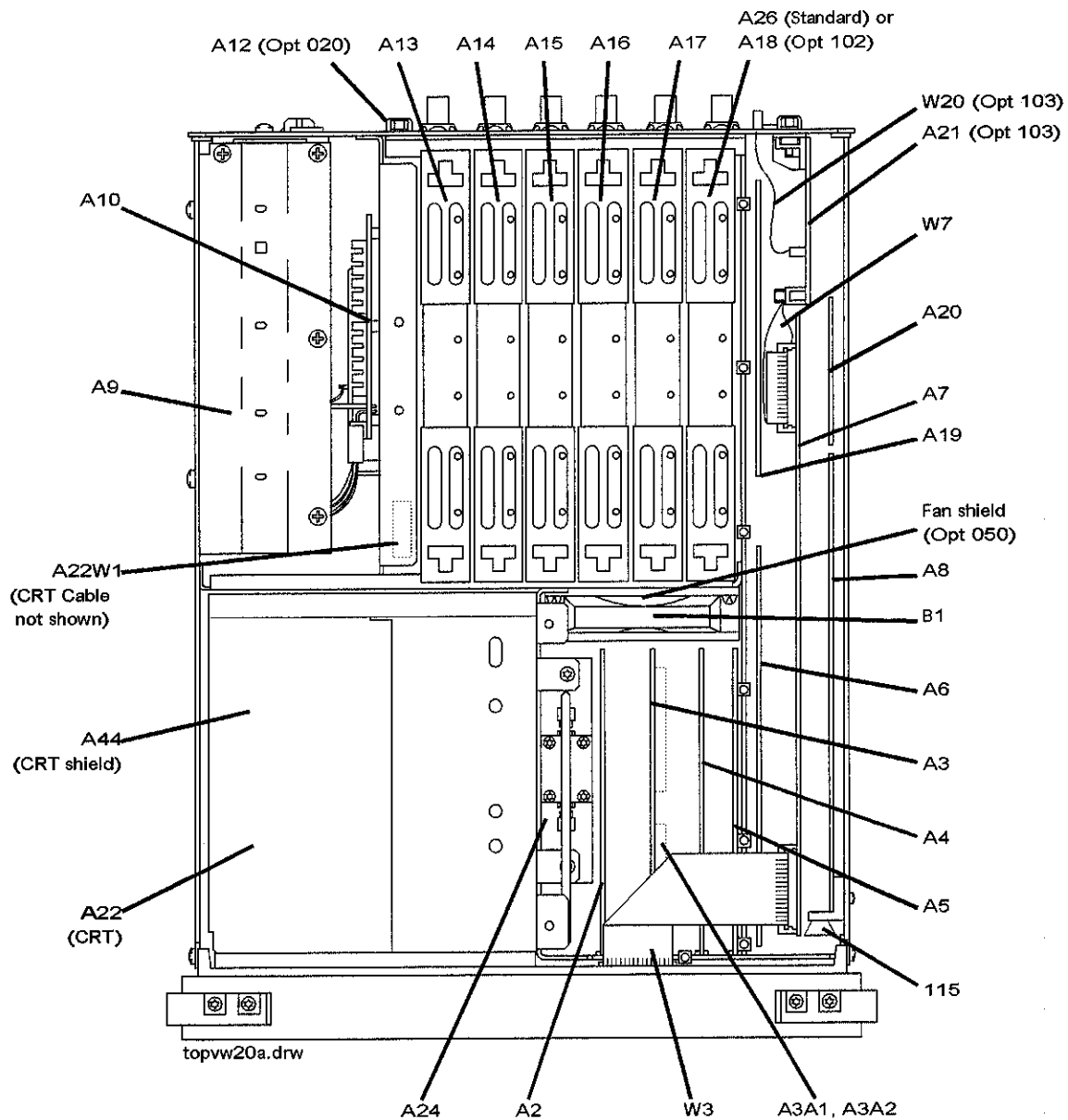
Major Assemblies and Cables, Top View
