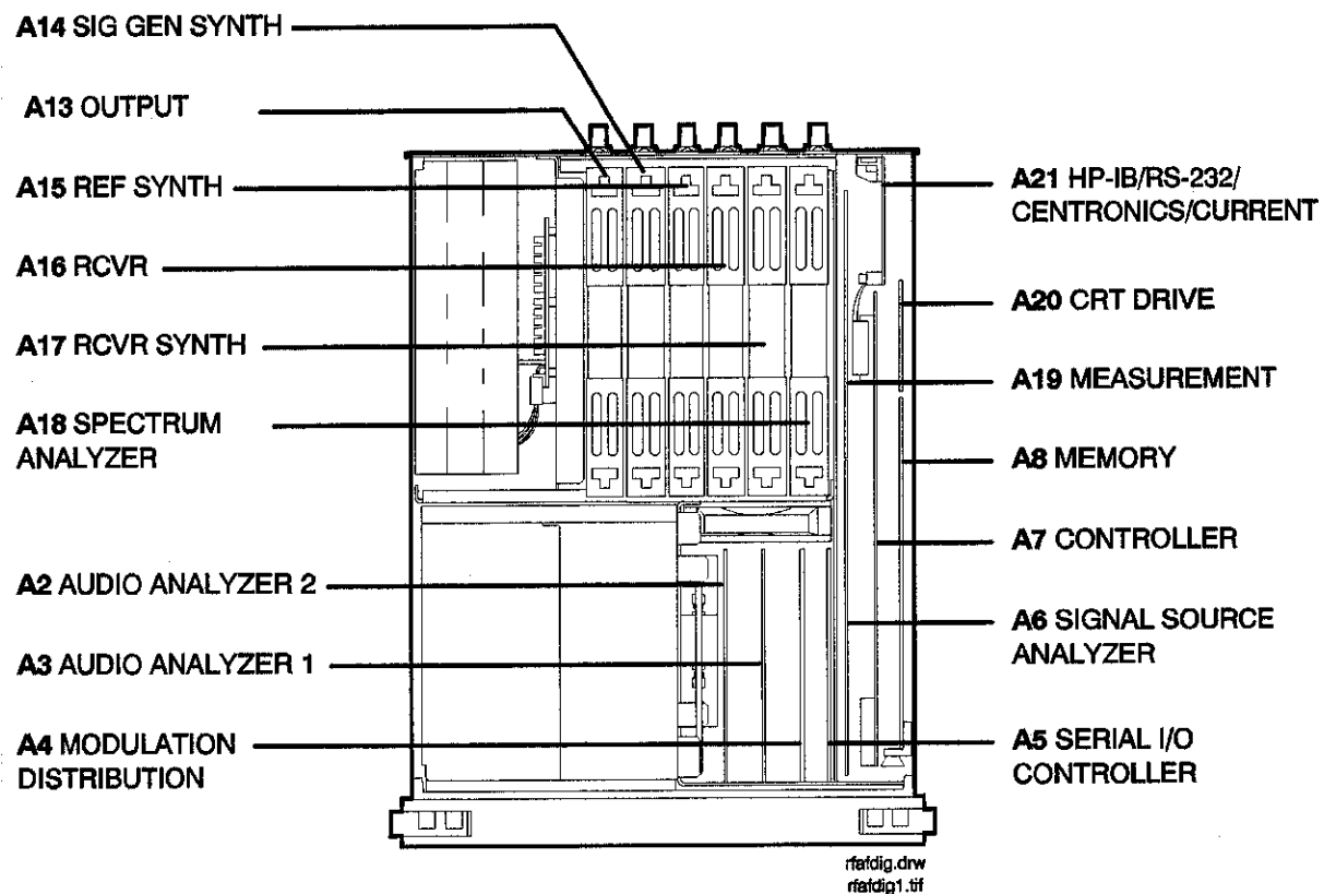
Figure 3-2. AF, Digital, And Most RF Assemblies
