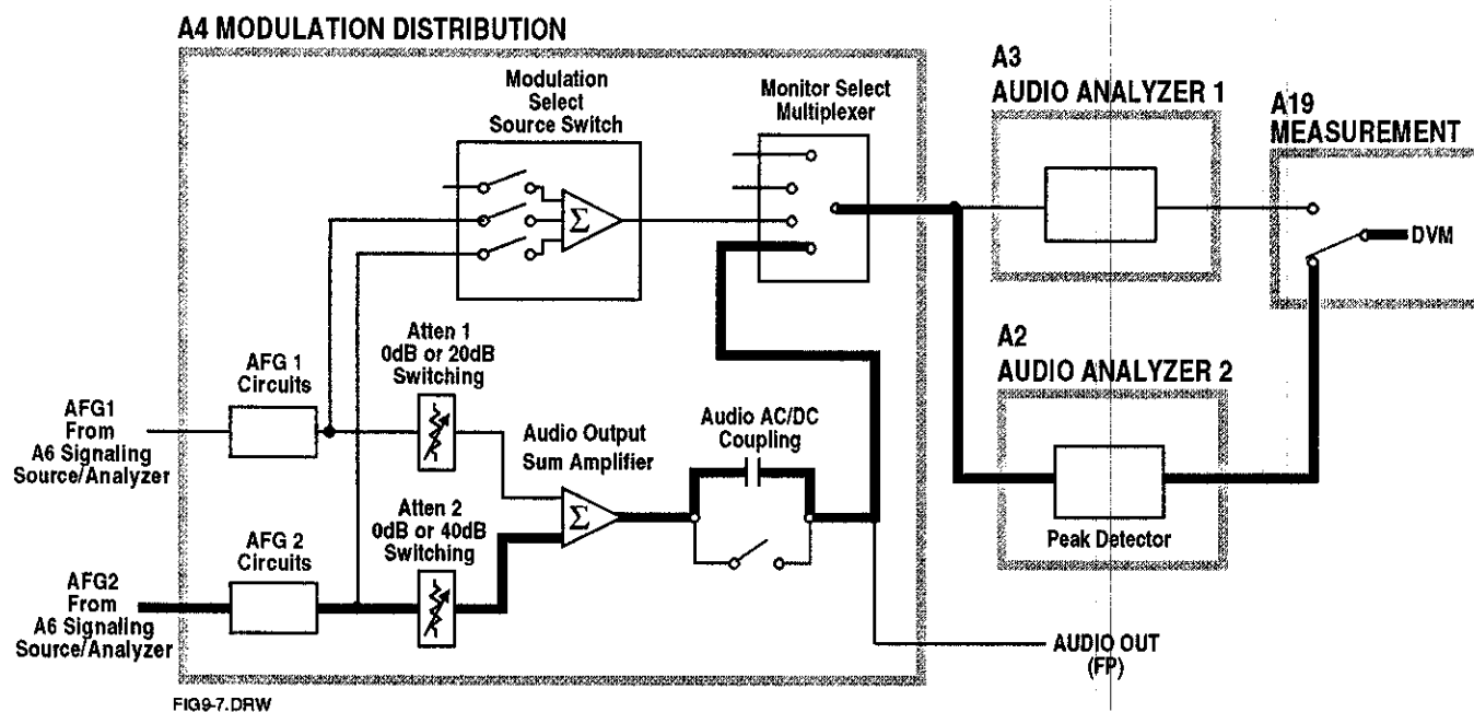
Figure 9-7. Preliminary Audio Path 9
