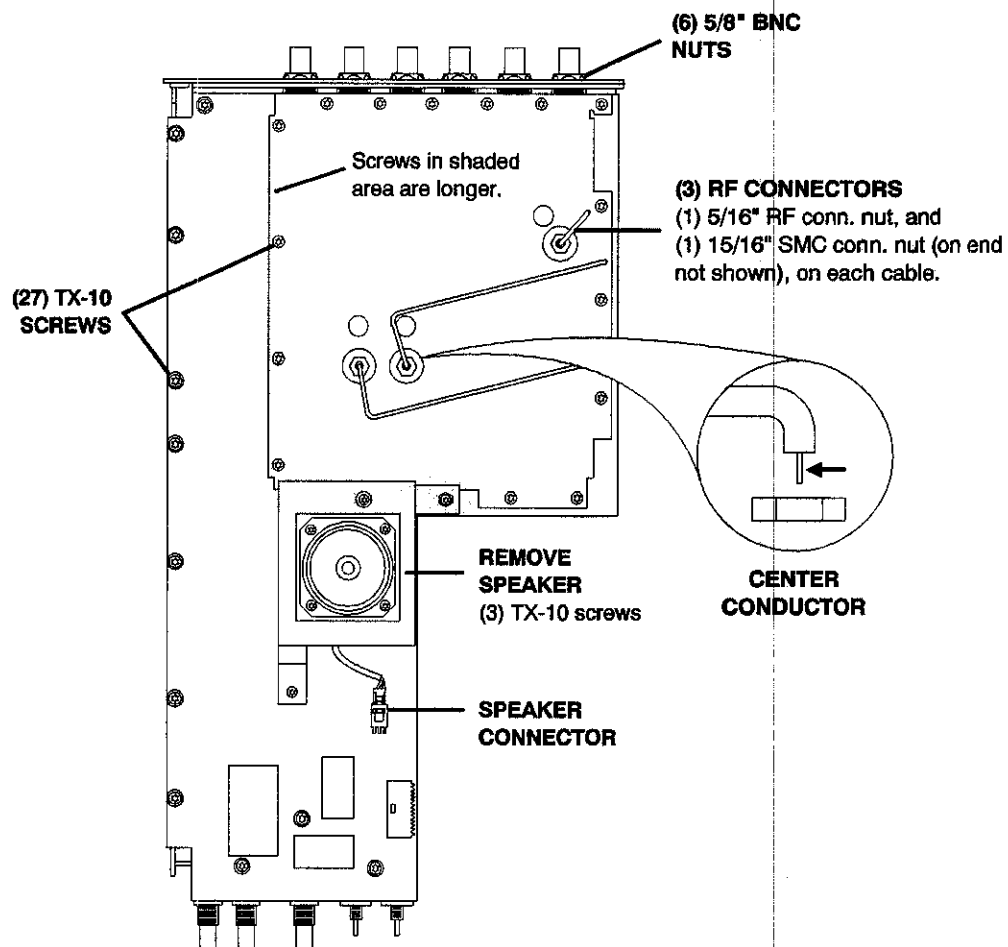
Figure 3-9. A25 Motherboard
