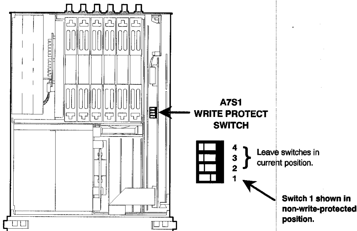
Figure 4-1. Location Of the Write-Protect Switch On the Controller Assembly.
