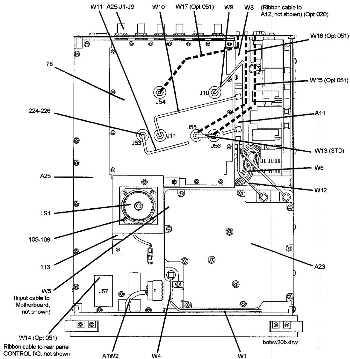
Major Assemblies and Cables, Bottom View
