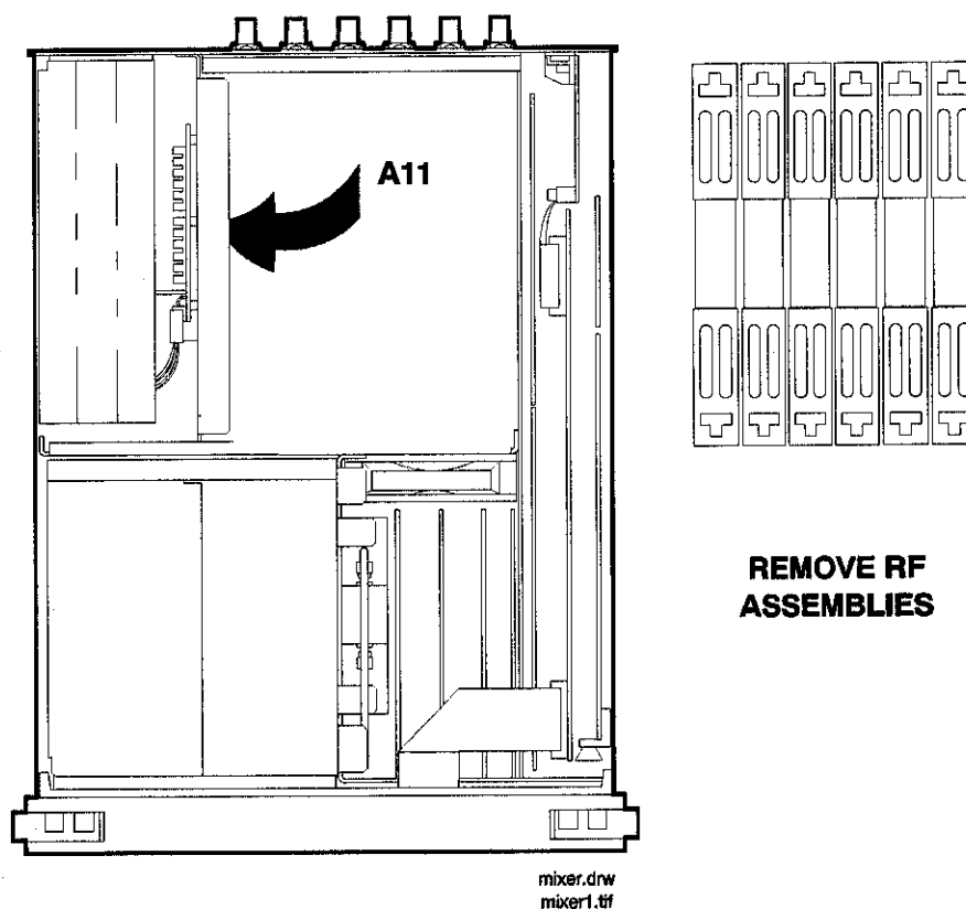
Figure 3-6. A11 Receiver Mixer
