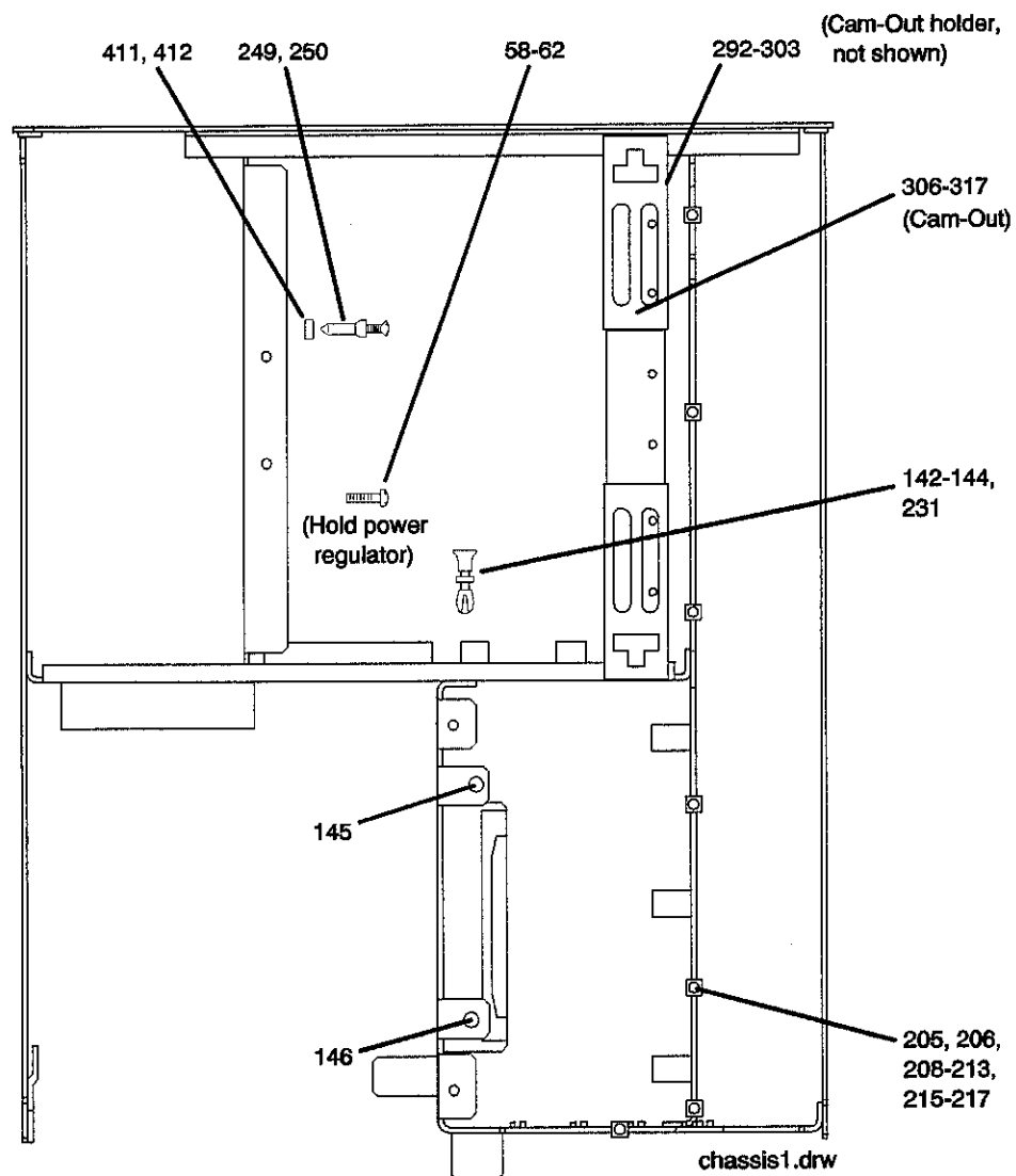
Attaching Hardware, Top View
