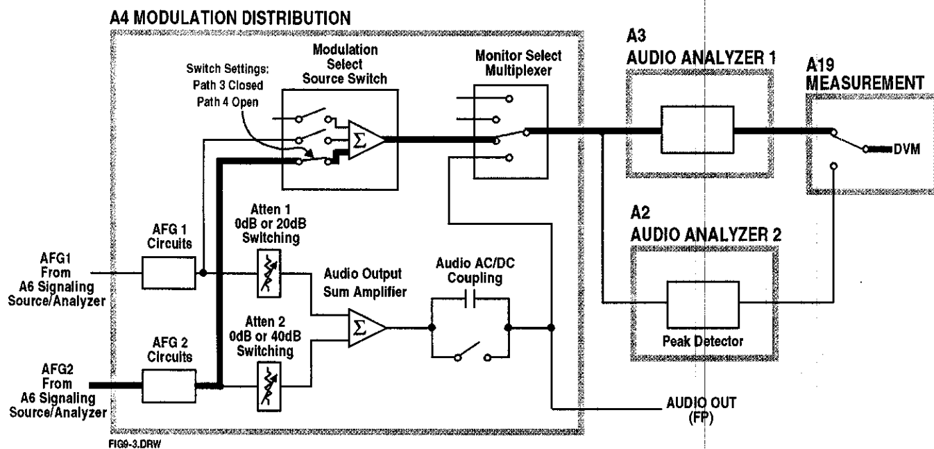
Figure 9-3. Preliminary Audio Paths 3 and 4
