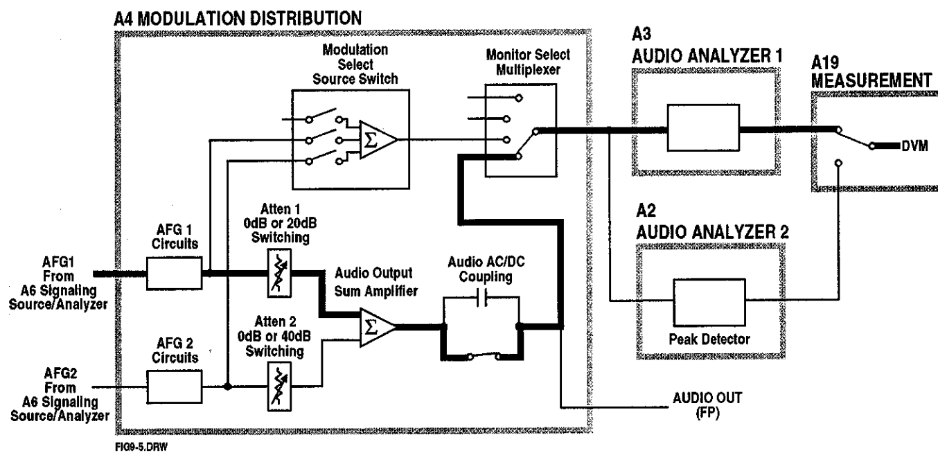
Figure 9-5. Preliminary Audio Path 6
