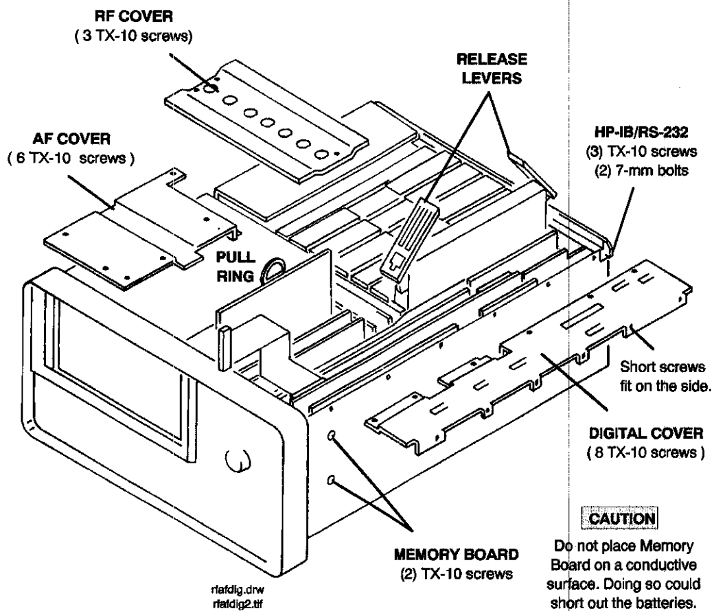
Figure 3-3. Internal Covers
