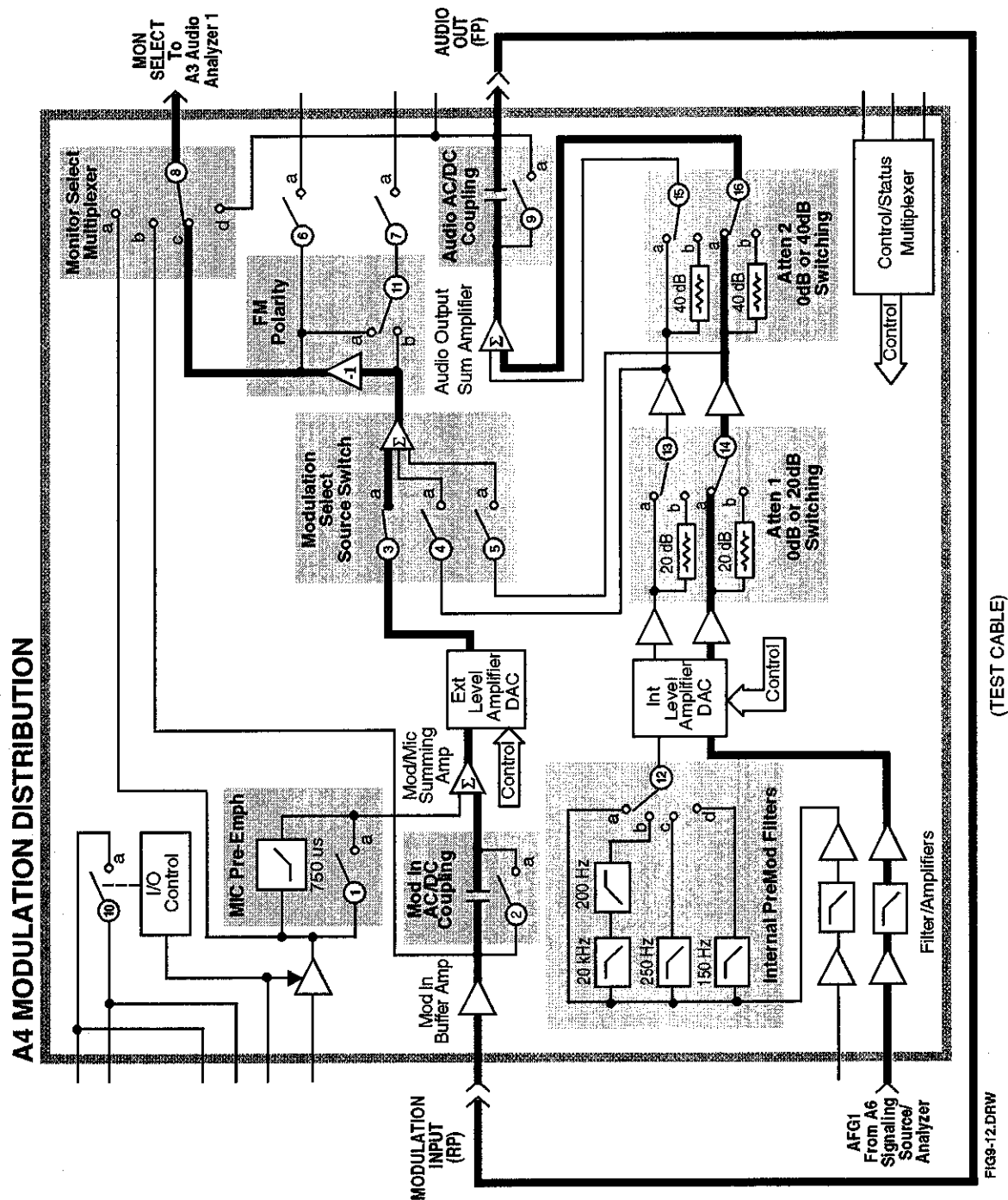
Figure 9-12. Modulation Distribution External Paths 3 to 7
