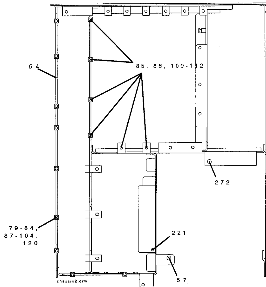
Chassis and Attaching Hardware, Bottom View
