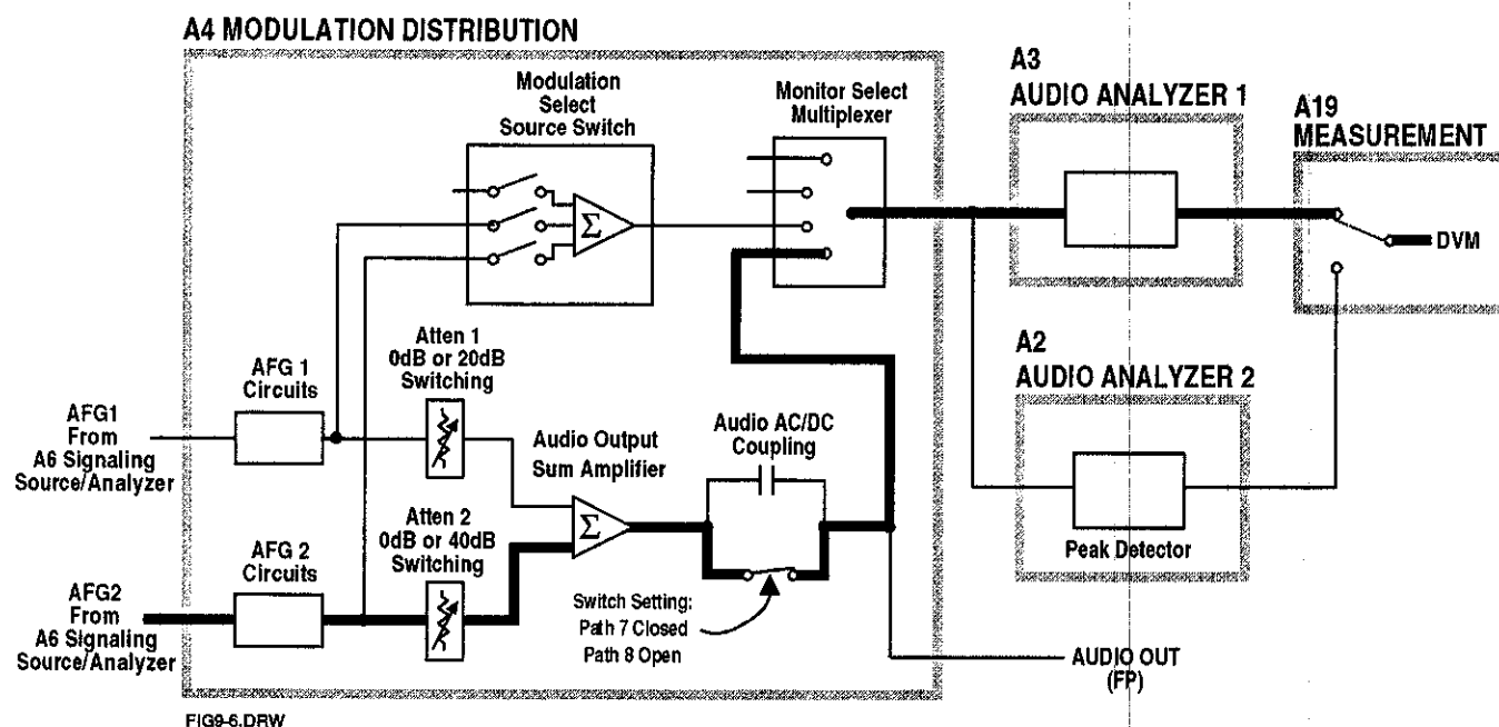
Figure 9-6. Preliminary Audio Paths 7 and 8
