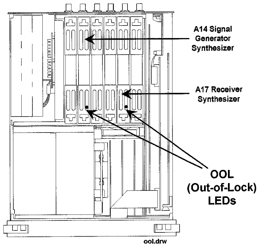
Figure 2-3. Location of the Out-of-Lock Annunciators
