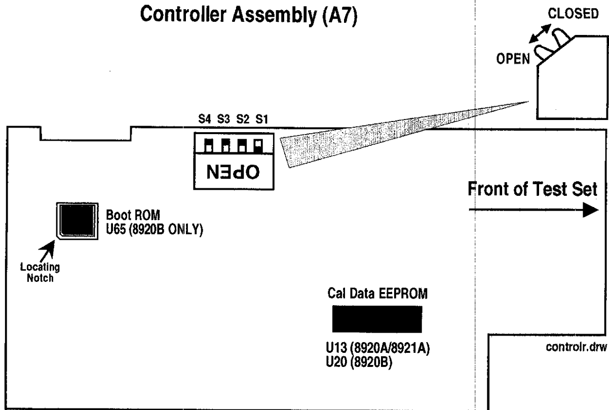
Figure 3-13. A7 Controller
