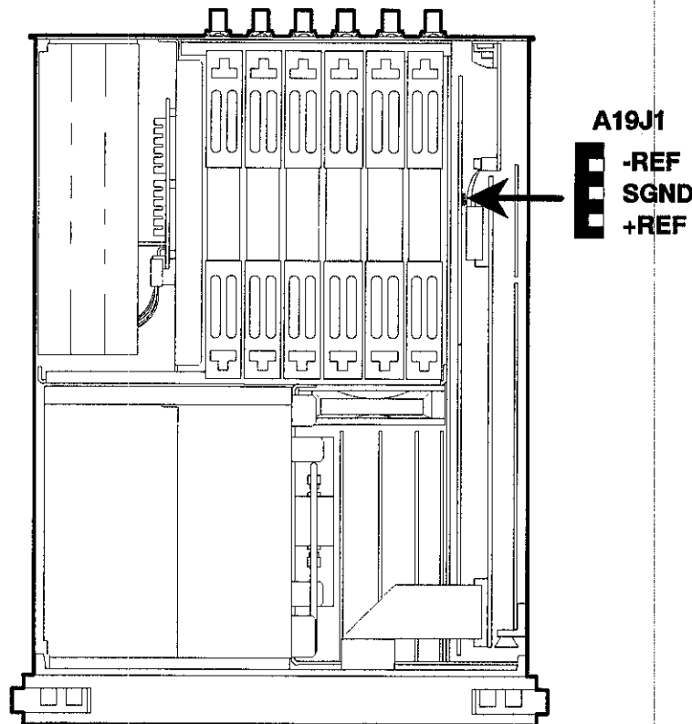
Figure 4-2. Location Of the Voltmeter Connections On the Measurement Assembly.
