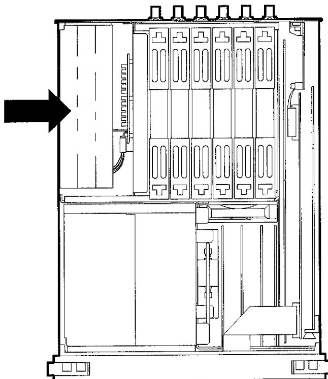
Figure 3-8. A9 Power Supply
