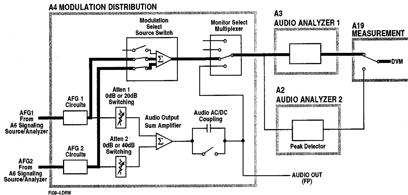
Figure 9-4. Preliminary Audio Path 5
