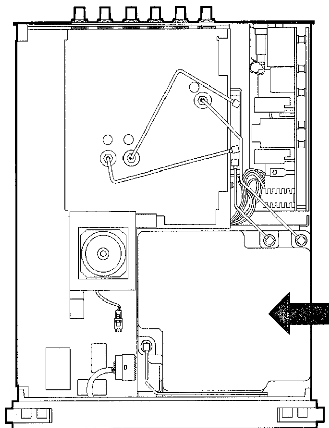
Figure 3-4. A23 RF Input Assembly
