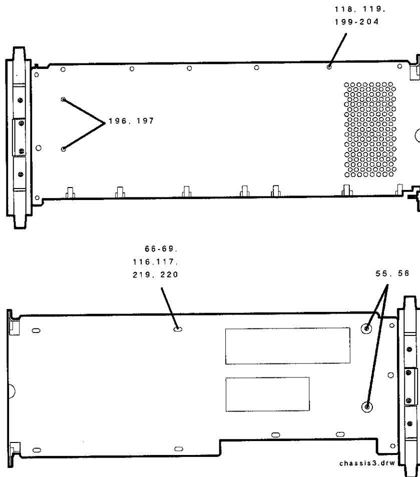
Attaching Hardware, Side View
