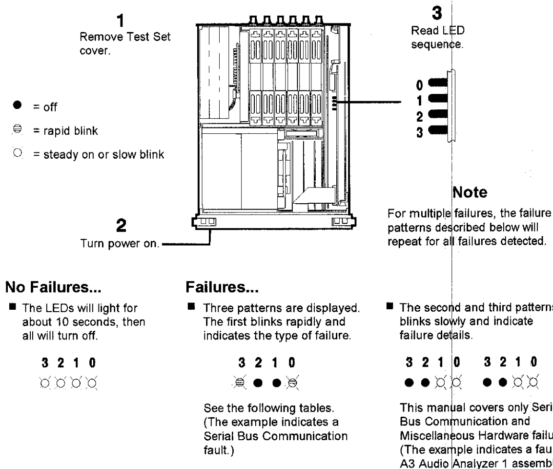
Figure 9-1. Reading the Self-Test Diagnostic Using the Internal LEDs
