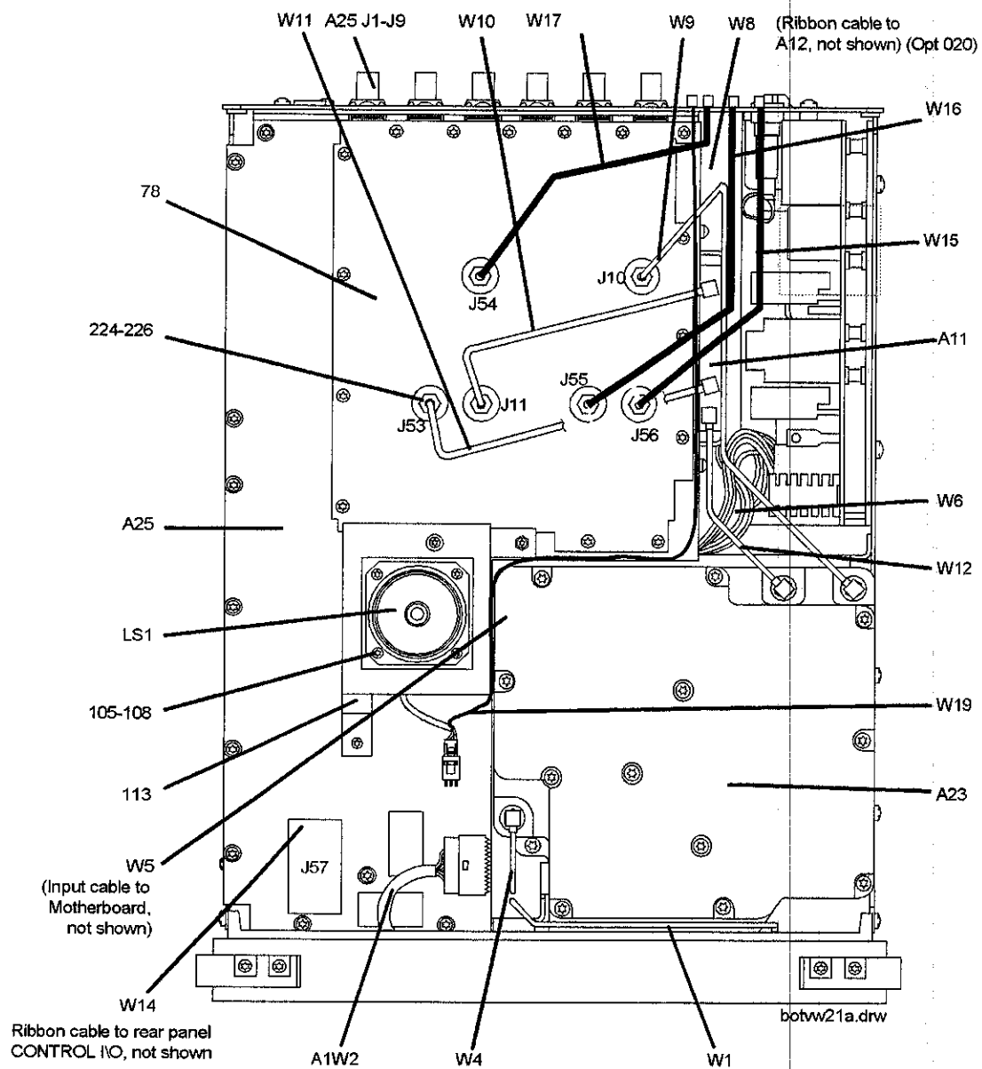
Major Assemblies and Cables, Bottom View
