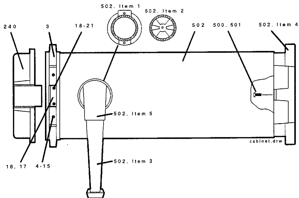
Instrument Cover, Bumpers and Attaching Hardware
