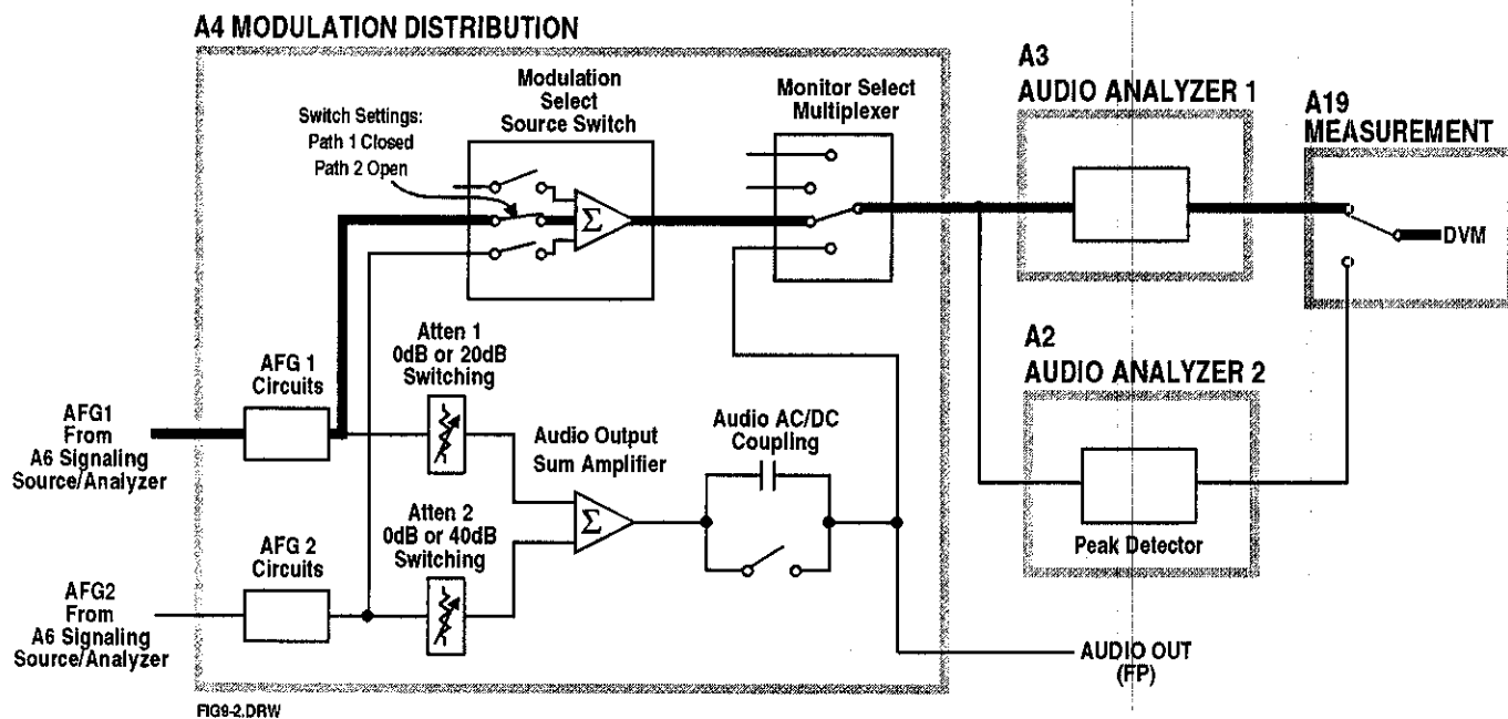
Figure 9-2. Preliminary Audio Paths 1 and 2
