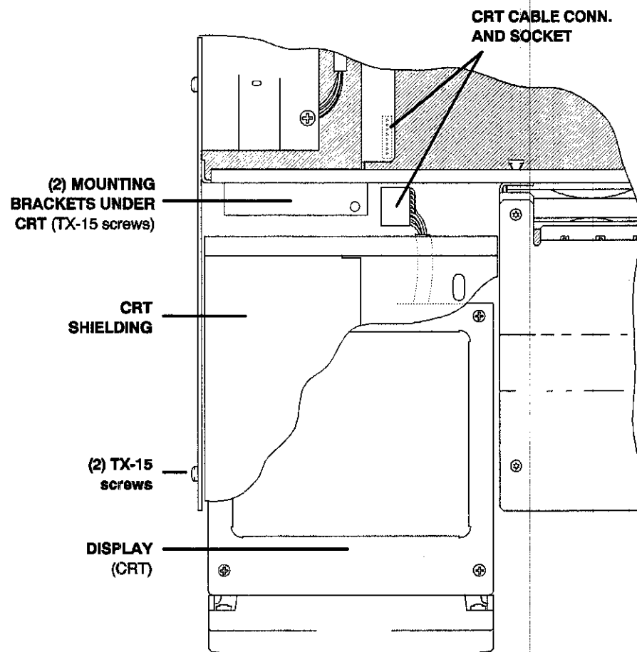
Figure 3-12. A20 Display (CRT)
