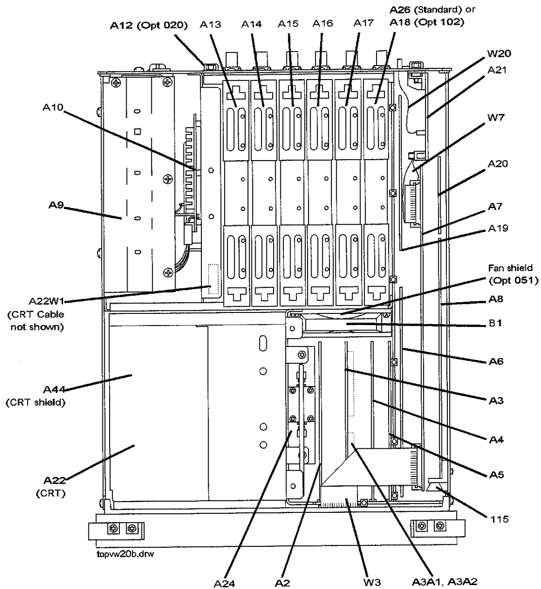
Major Assemblies and Cables, Top View
