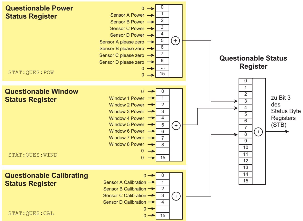
Abbildung 6-13: Questionable Status Register
