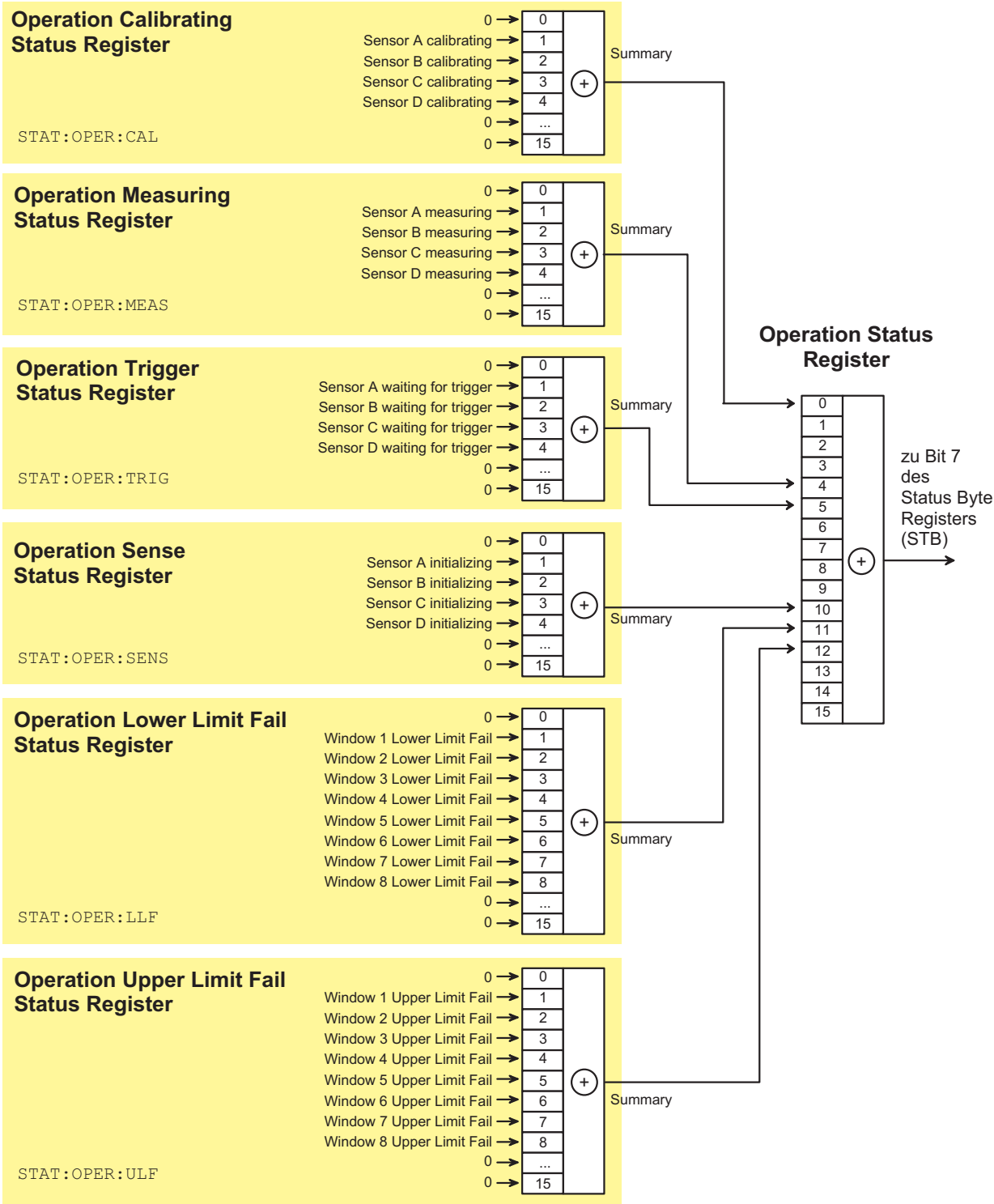
Abbildung 6-12: Operation Status Register
