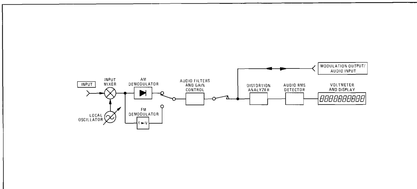
Audio Distortion and Level Block Diagram
