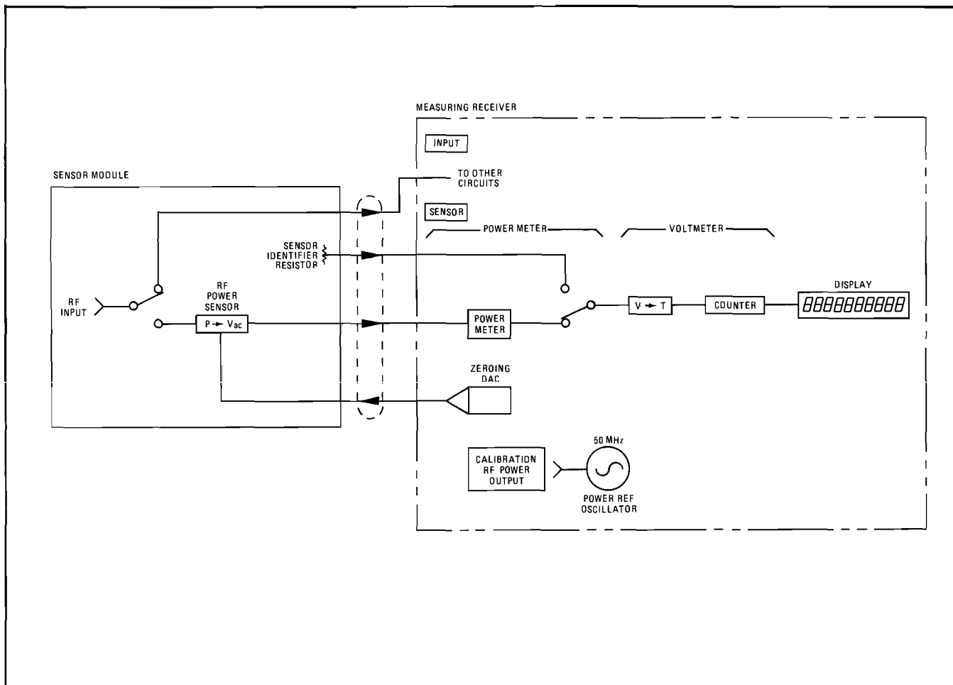
Simplified Block Diagram of RF Power Calibration
