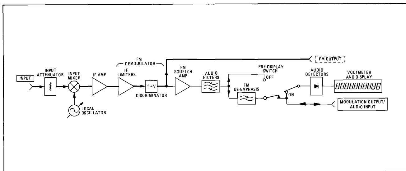
FM OUTPUT Block Diagram
