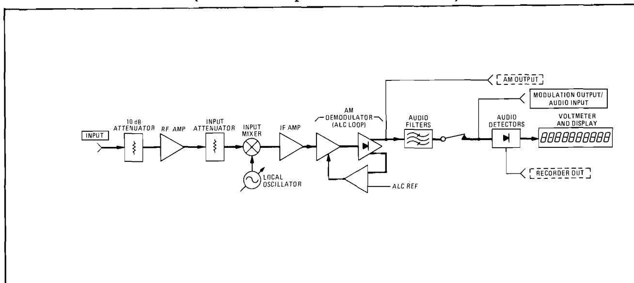
AM Measurement Block Diagram
