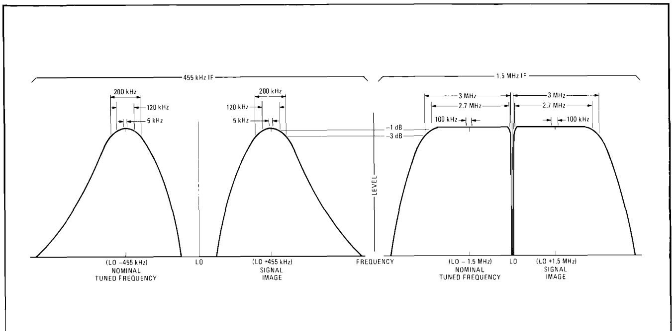
Spectrum Diagram of the 455 kHz and 1.5 MHz Passbands
