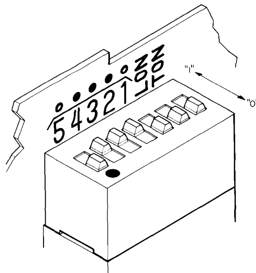
Figure 2-2. The HP-IB Address Switch Shown as Set by the Factory. The Address Shown is 01110 in Binary With Both Talk Only and Listen Only Off
