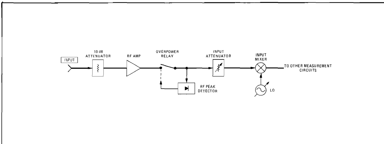
Block Diagram of RF Input Attenuation and Gain
