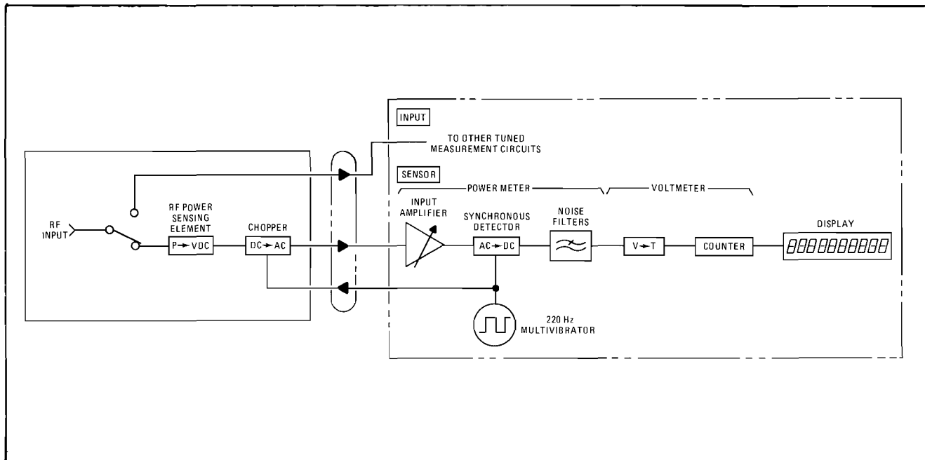
RF Power Block Diagram
