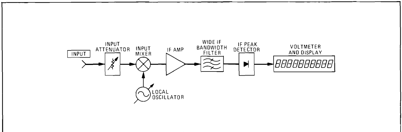
Peak Tuned RF Level Measurement Block Diagram
