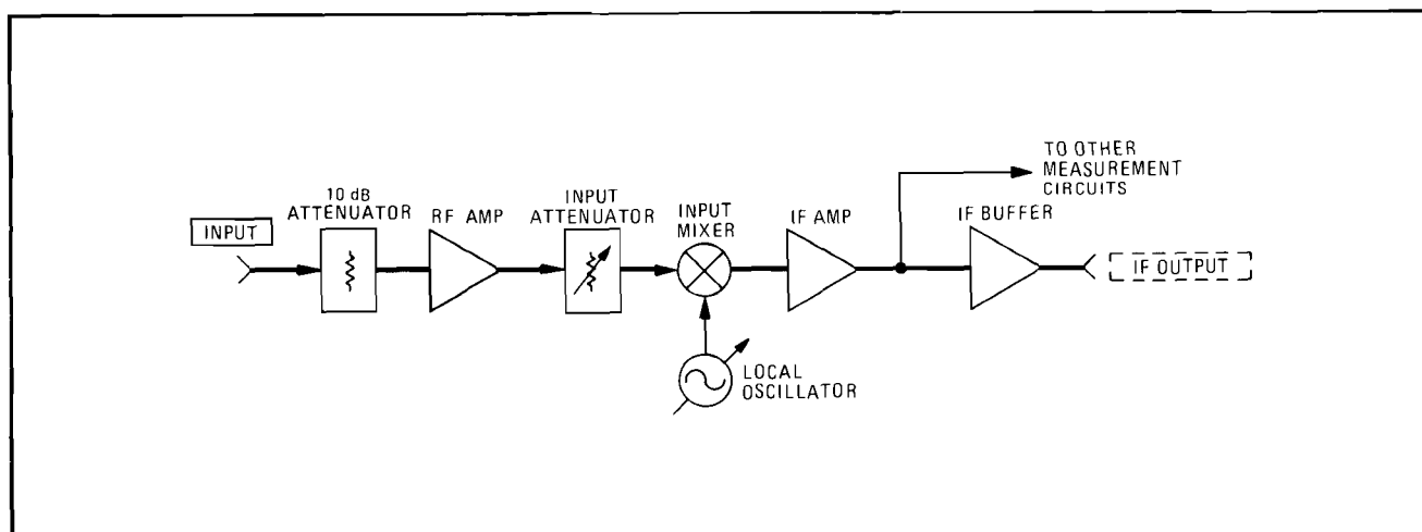
IF Output Block Diagram
