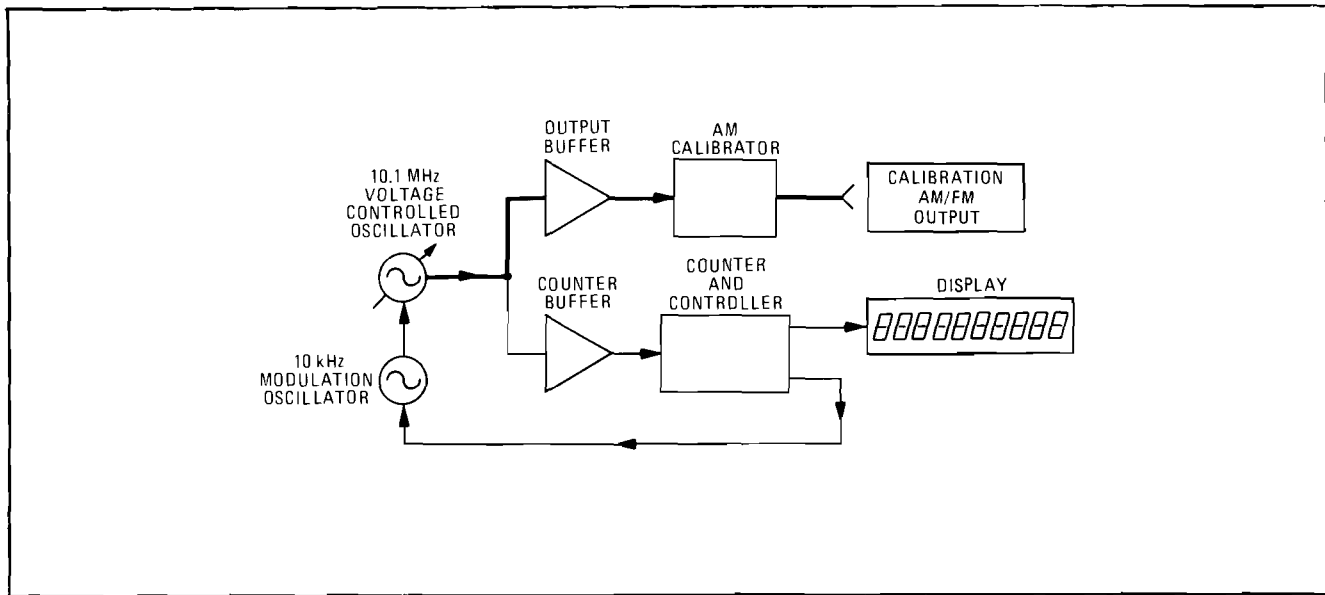
Simplified Block Diagram of the FM Calibrator
