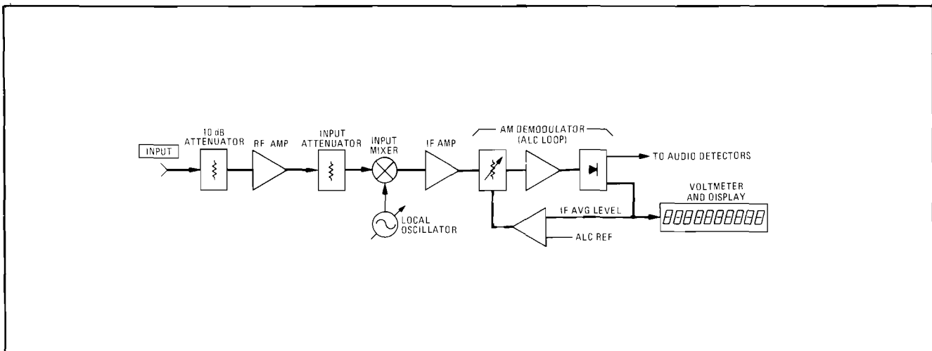
IF Level Measurement Block Diagram
