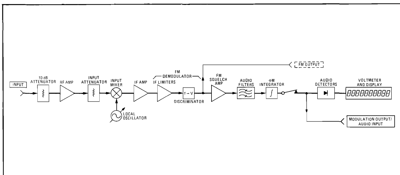
\phi M Measurement Block Diagram
