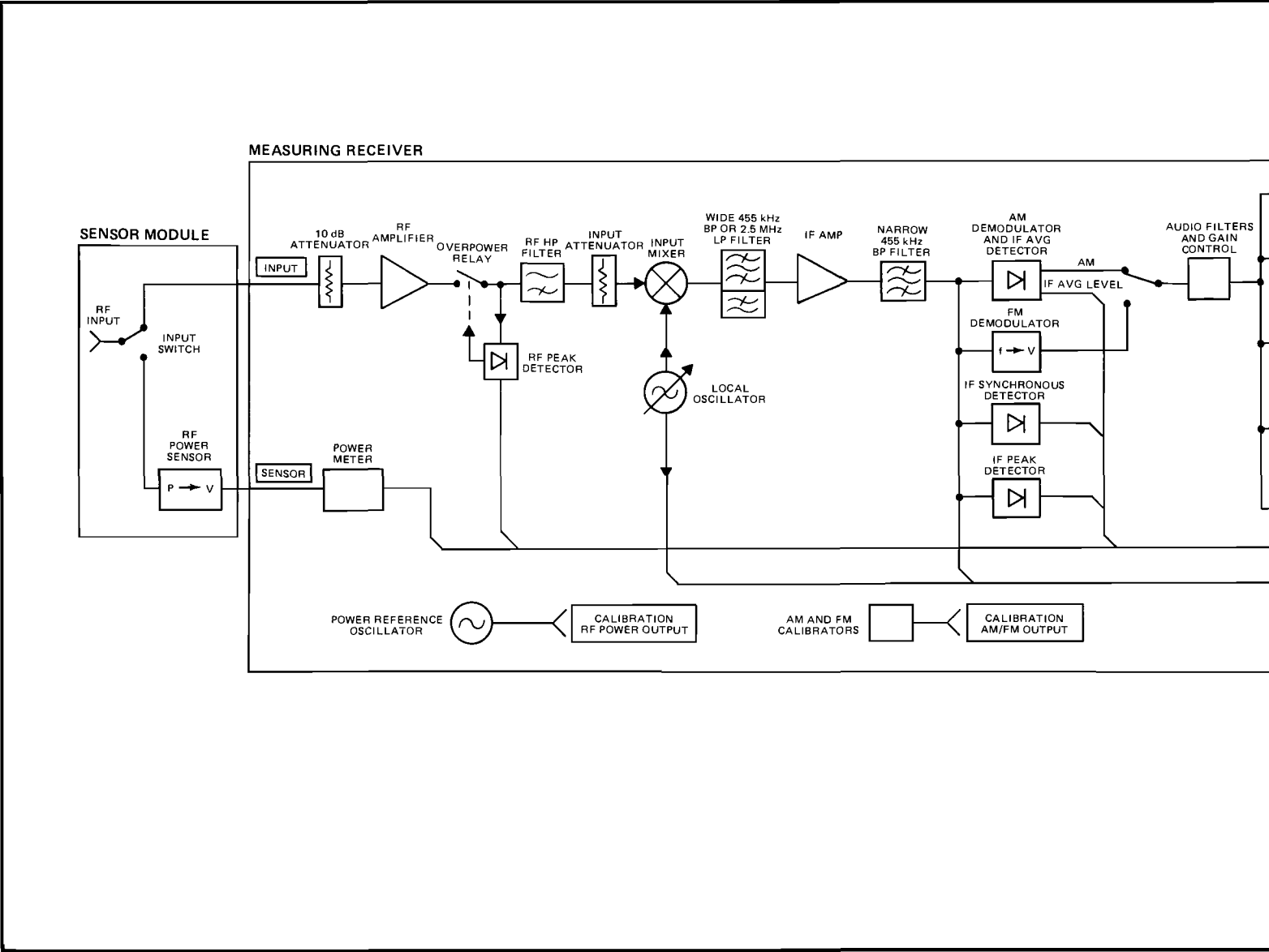
Figure 1-2. HP 8902A Measuring Receiver Simplified Block Diagram
