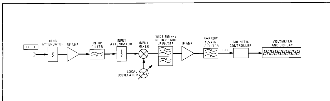
Block Diagram of RF and IF Filters
