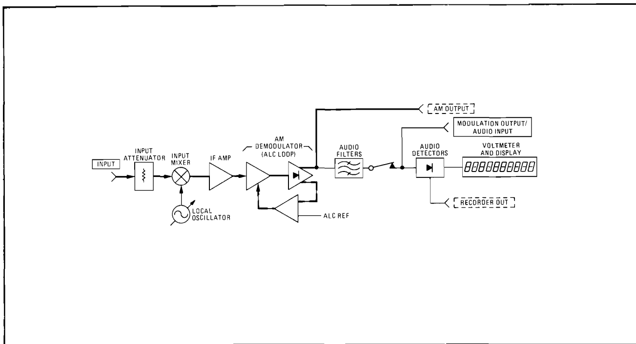
AM Output Block Diagram
