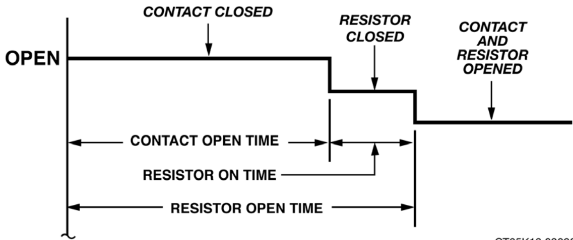
Figure 29. Graphical Interpretation of an OPEN Timing Shot
