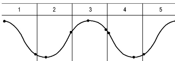
Peak Detect acquisition intervals (1250)
