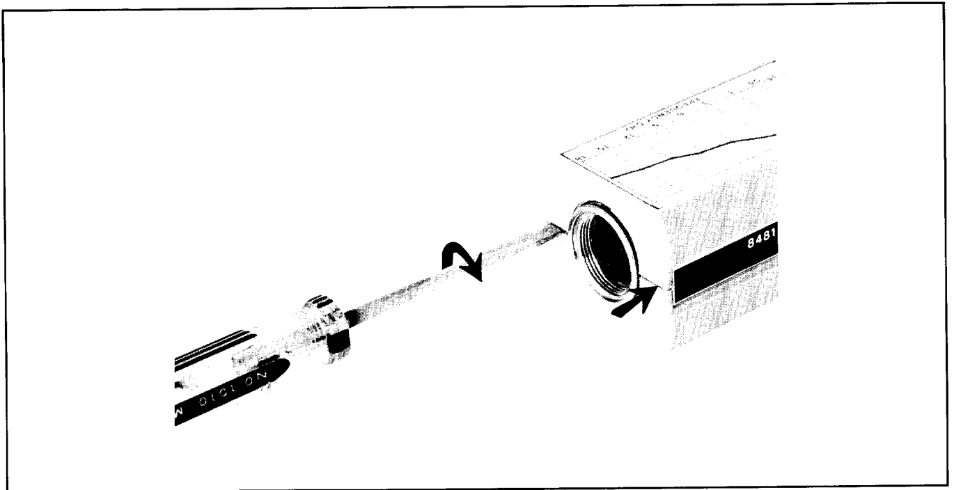
Figure 6. Removing the Power Sensor's Cover
