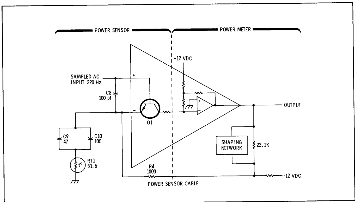
Figure 5. Operational Amplifier
