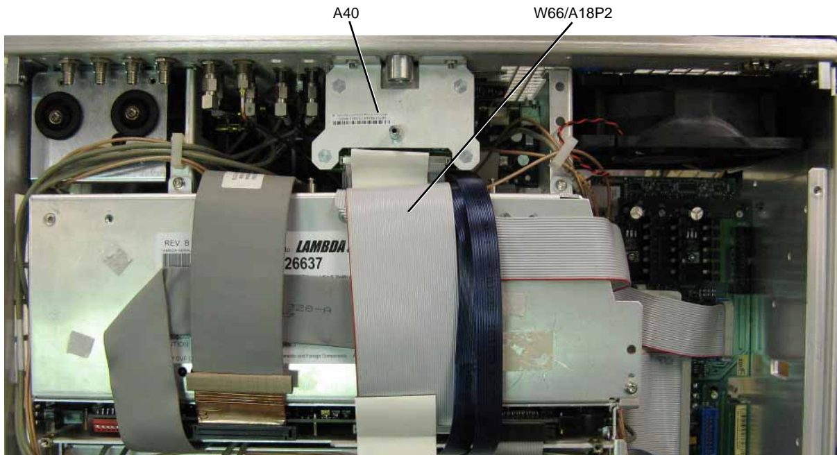
Figure 3-66 A40 Flash Drive Assembly
