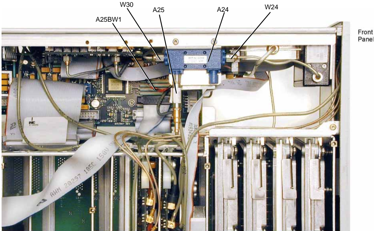
Figure 3-33 A24 40 GHz Highband Coupler (Option 540 – Standard)
