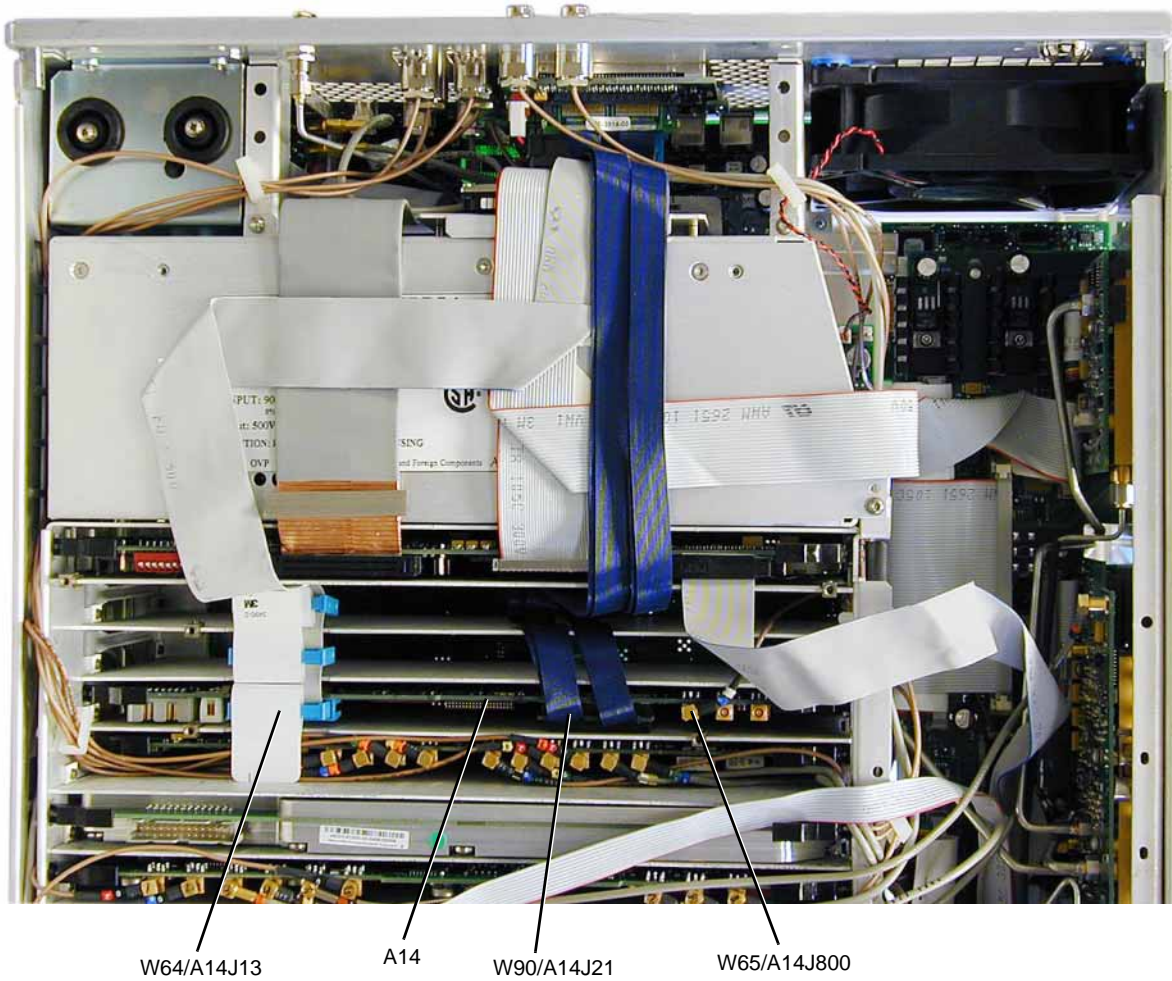
Figure 3-20 A14 Baseband Generator
