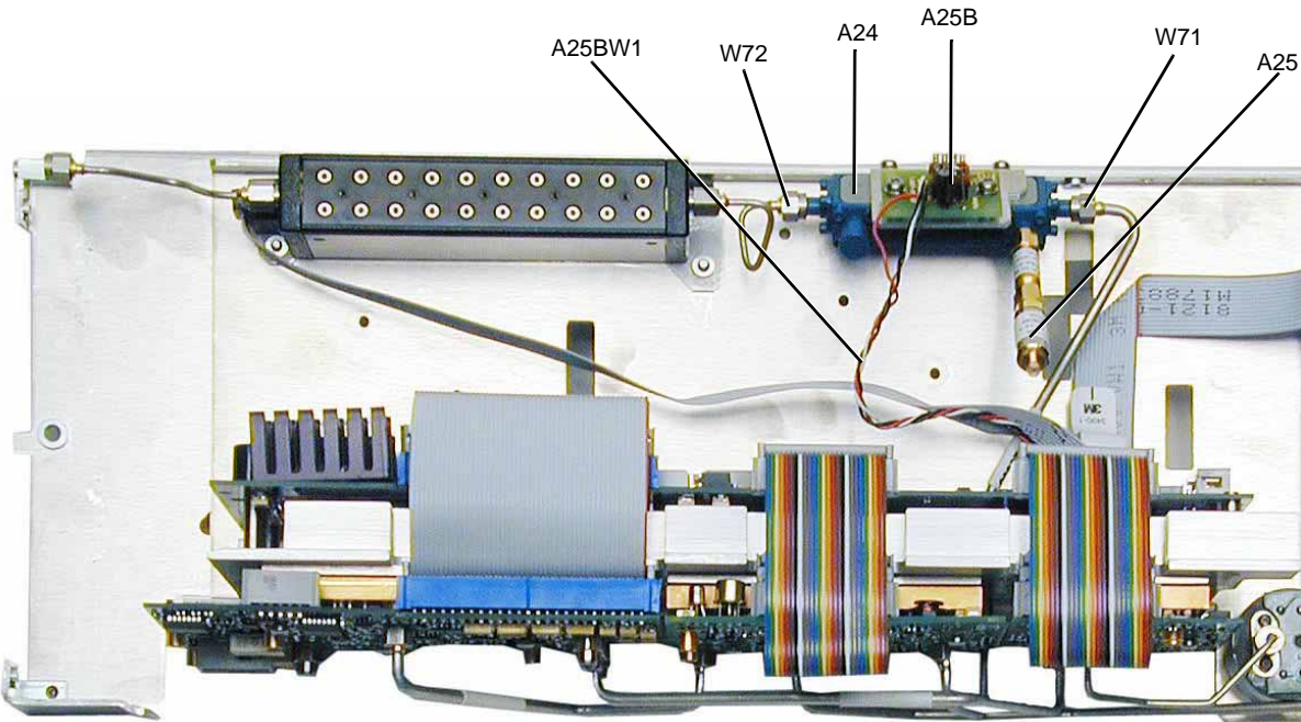
Figure 3-34 A24 40 GHz Highband Coupler (Option 540 – Option 1EM)
