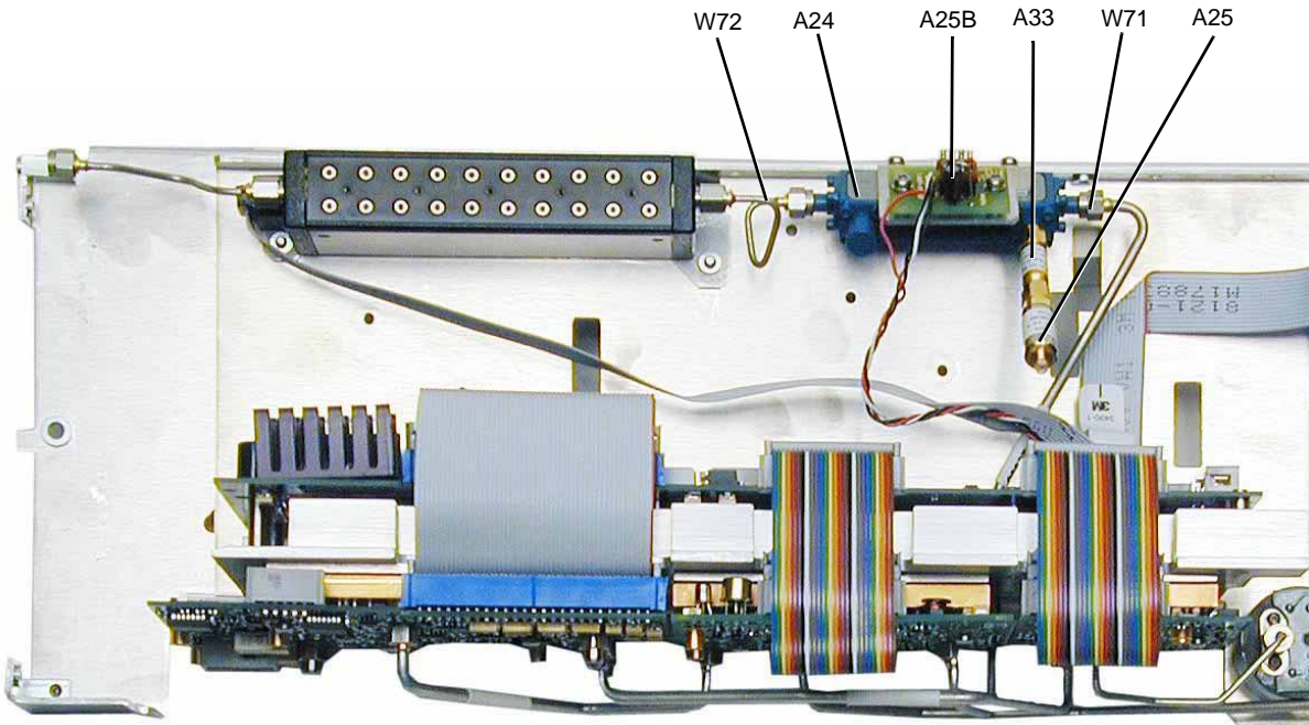
Figure 3-30 A24 20 GHz Highband Coupler (Options 503, 509 and 520 – Option 1EM)
