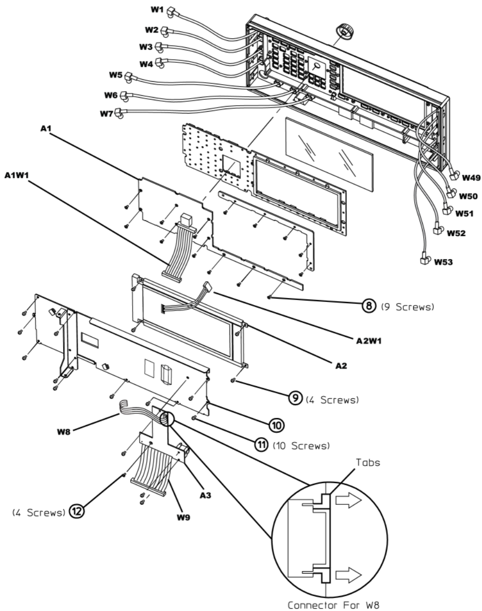
A2 Display Removal with serial prefixes > US/MY5XXX3XXX
