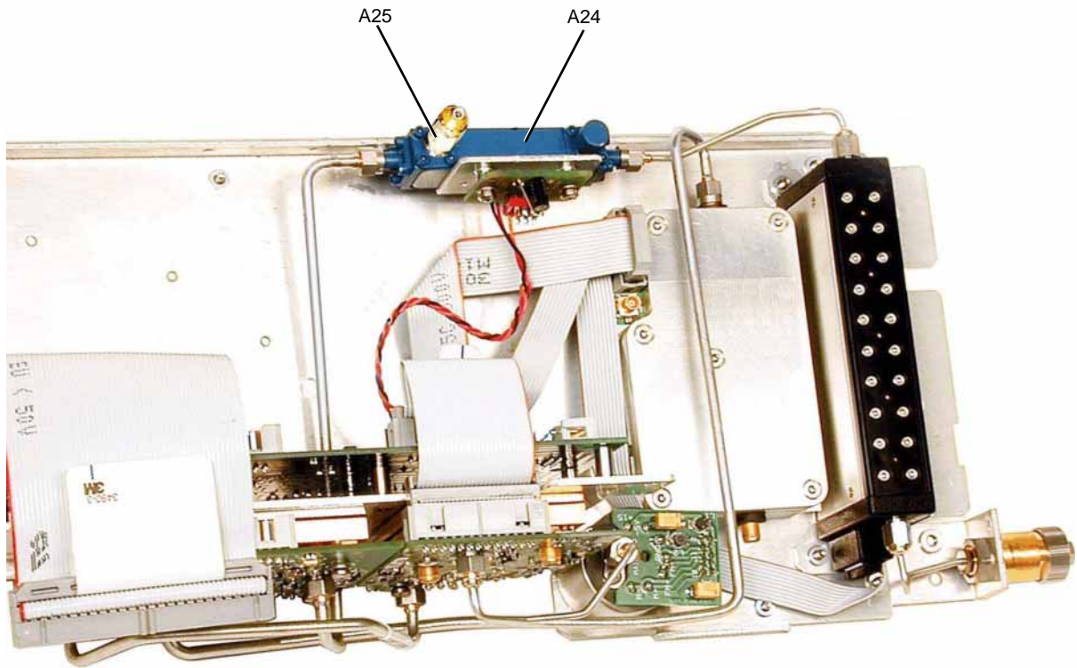
Figure 3-41 A25 40 GHz Highband Detector (Option 540)
