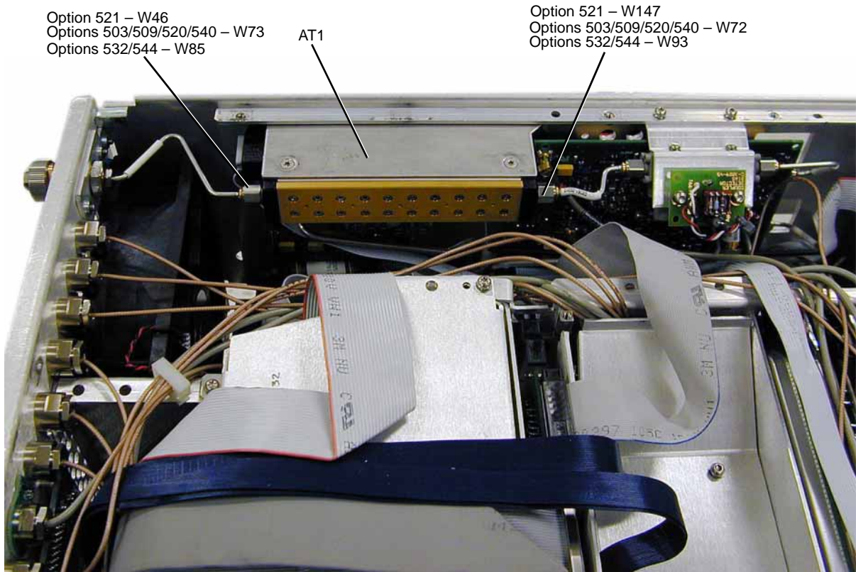
Figure 3-75 AT1 115dB Attenuator (Option 1EM)
