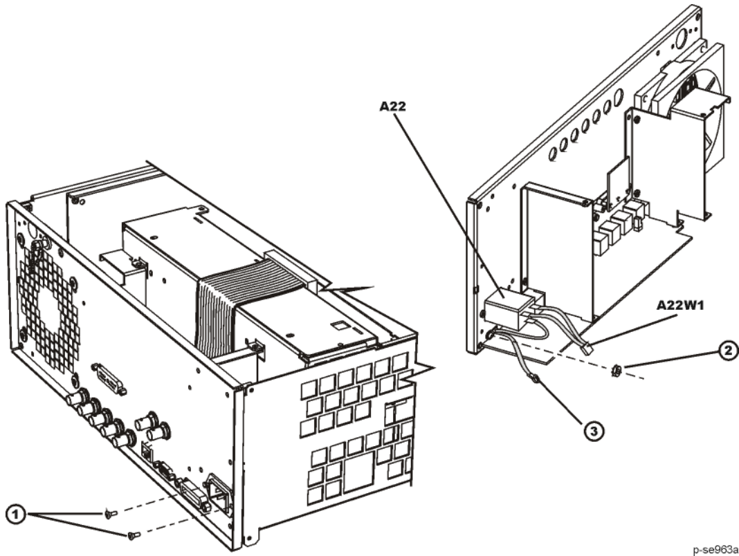
Figure 3-27 A22 Line Module Removal
