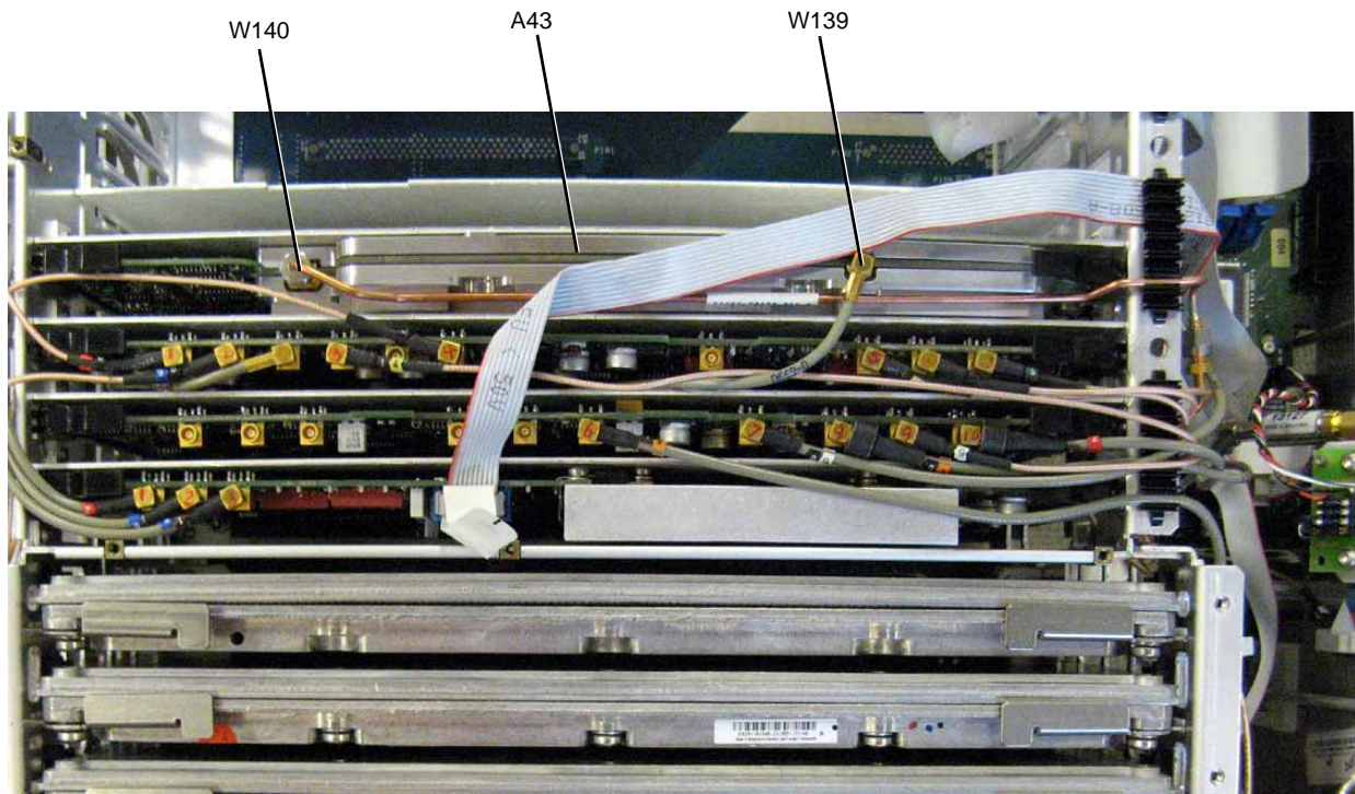
Figure 3-70 A43 Lowband Amp Filter
