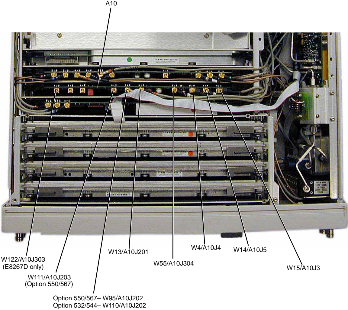
Figure 3-15 A10 ALC
