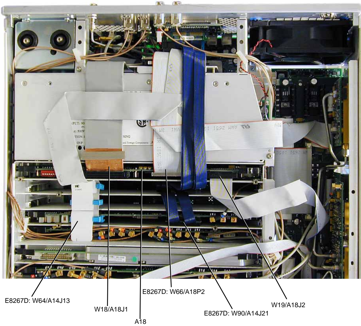
Figure 3-22 A18 CPU
