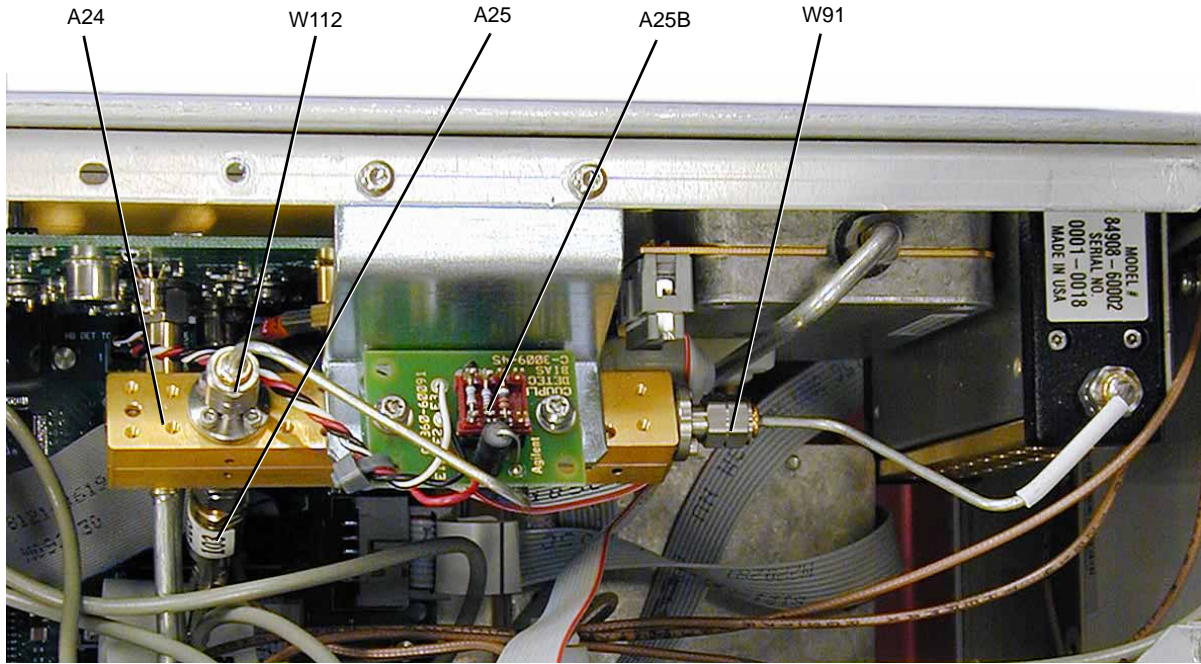
Figure 3-38 A24 67 GHz Highband Coupler (Options 550 & 567 and Option 1EM)
