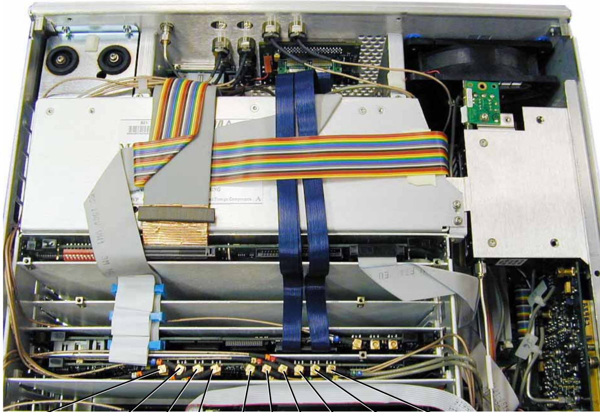
Figure 3-18 A13 I/Q MUX (E8267D Standard or with Option 015) (Serial Prefixes <US4722/MY4722)
