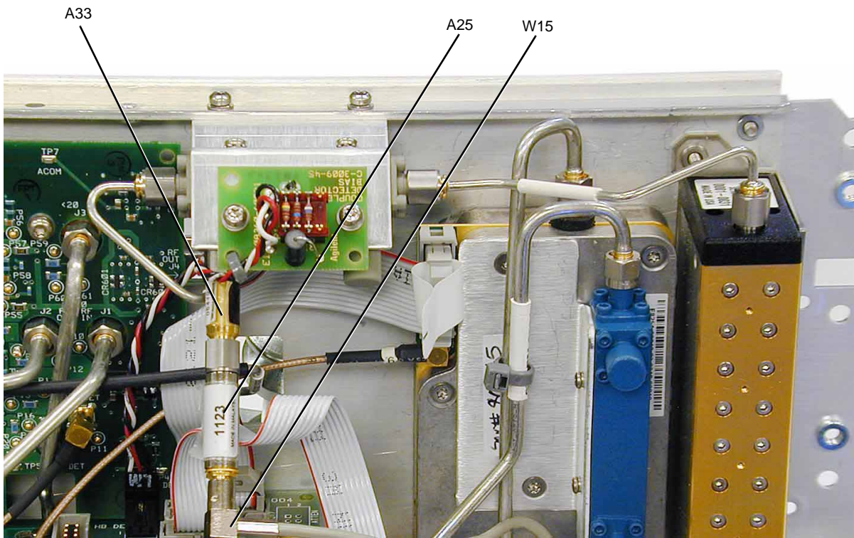
Figure 3-42 A25 50 GHz Highband Detector (Options 532 and 544)
