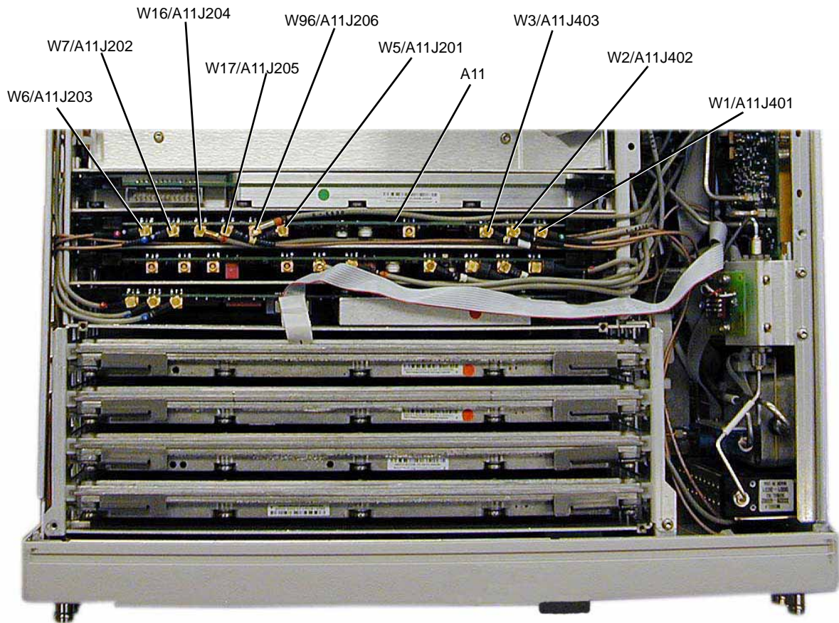
Figure 3-16 A11 Pulse/Analog Modulation Generator
