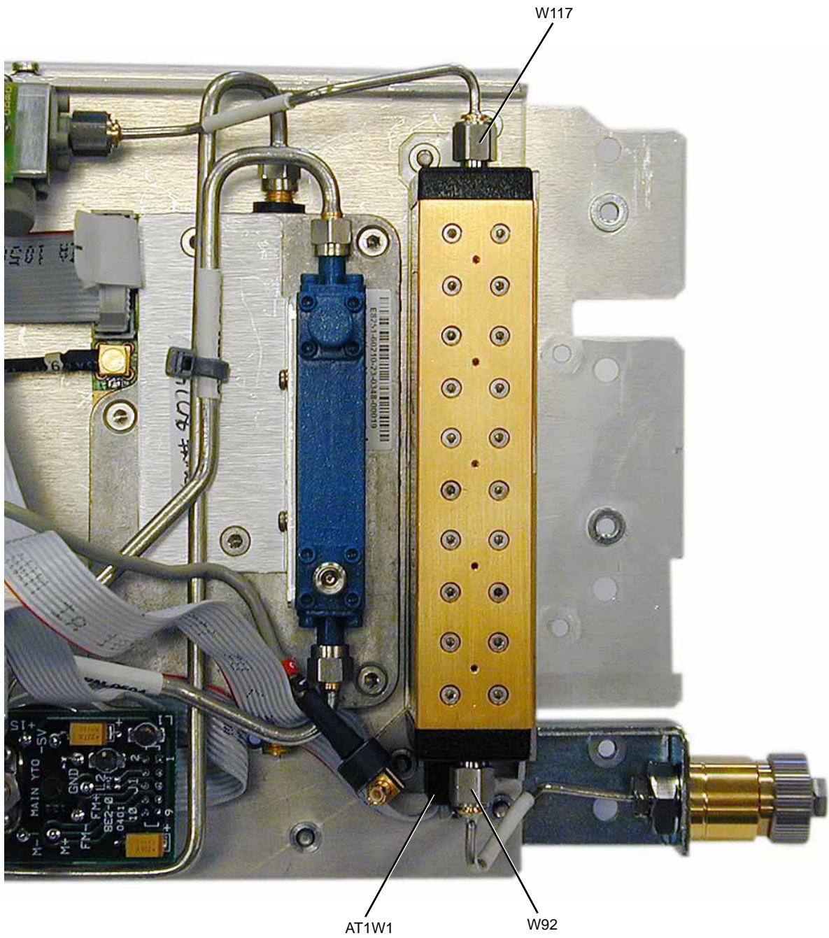
Figure 3-72 AT1 90 dB Attenuator
