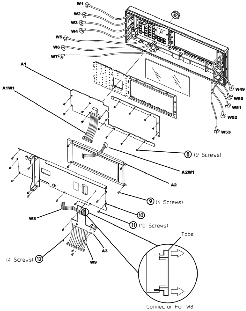
A1 Keyboard Removal with serial prefixes > US/MY5XXX3XXX
