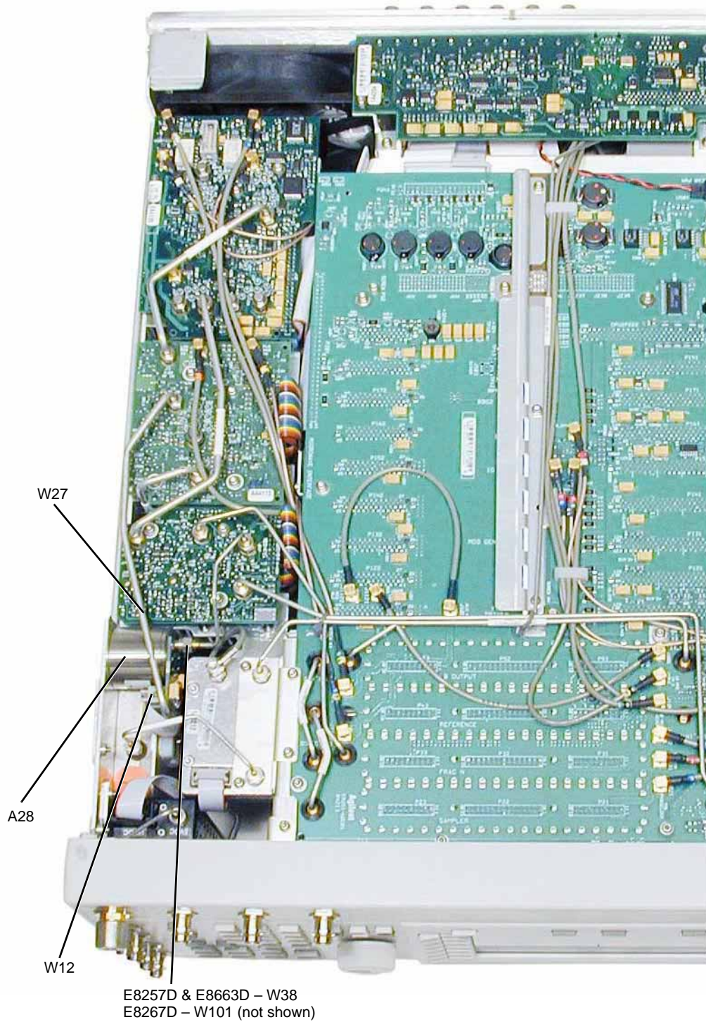
Figure 3-49 A28 YIG Oscillator
