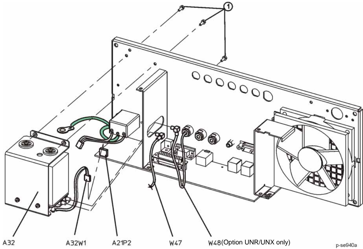
Figure 3-54 A32 Crystal Oscillator
