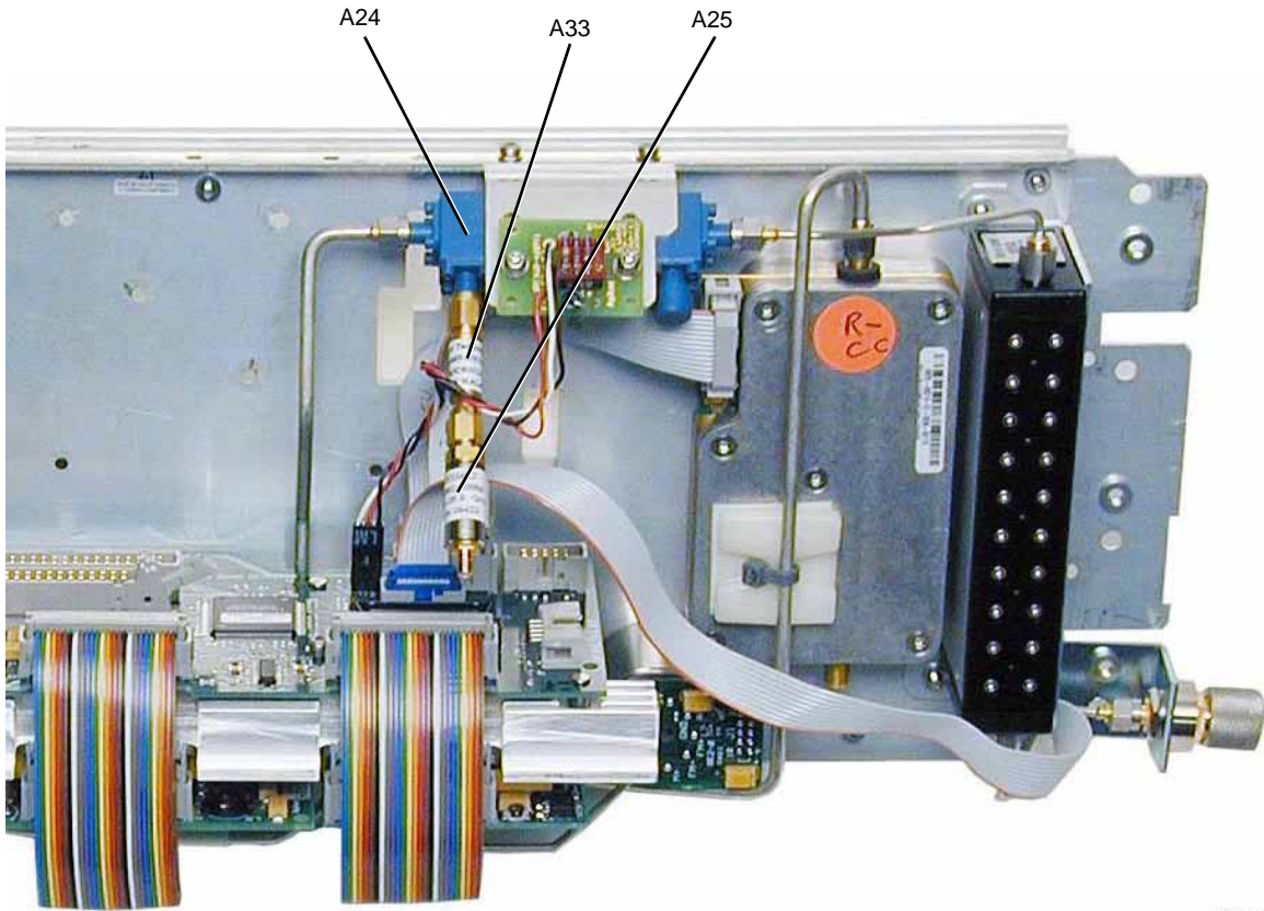
Figure 3-55 A33 6dB PAD (Options 503, 509, 520, and 521)
