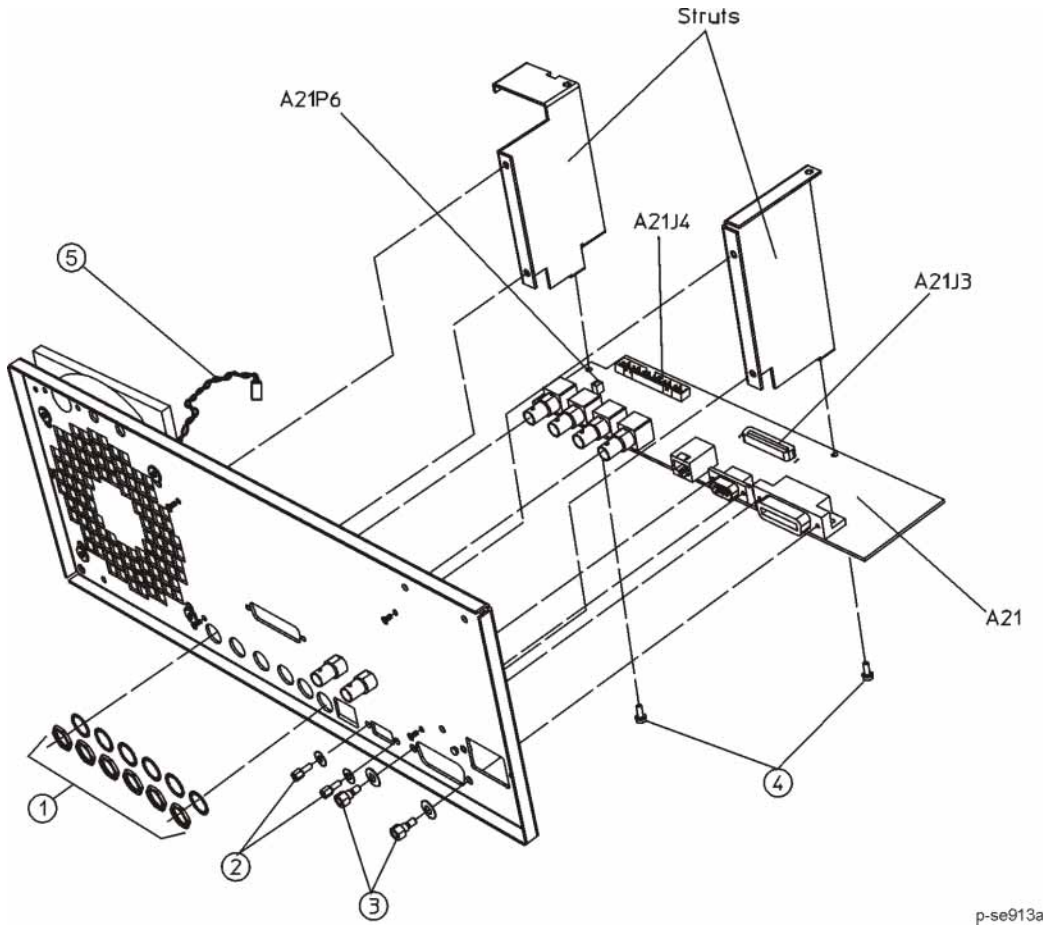
Figure 3-26 A21 Rear Panel Interface
