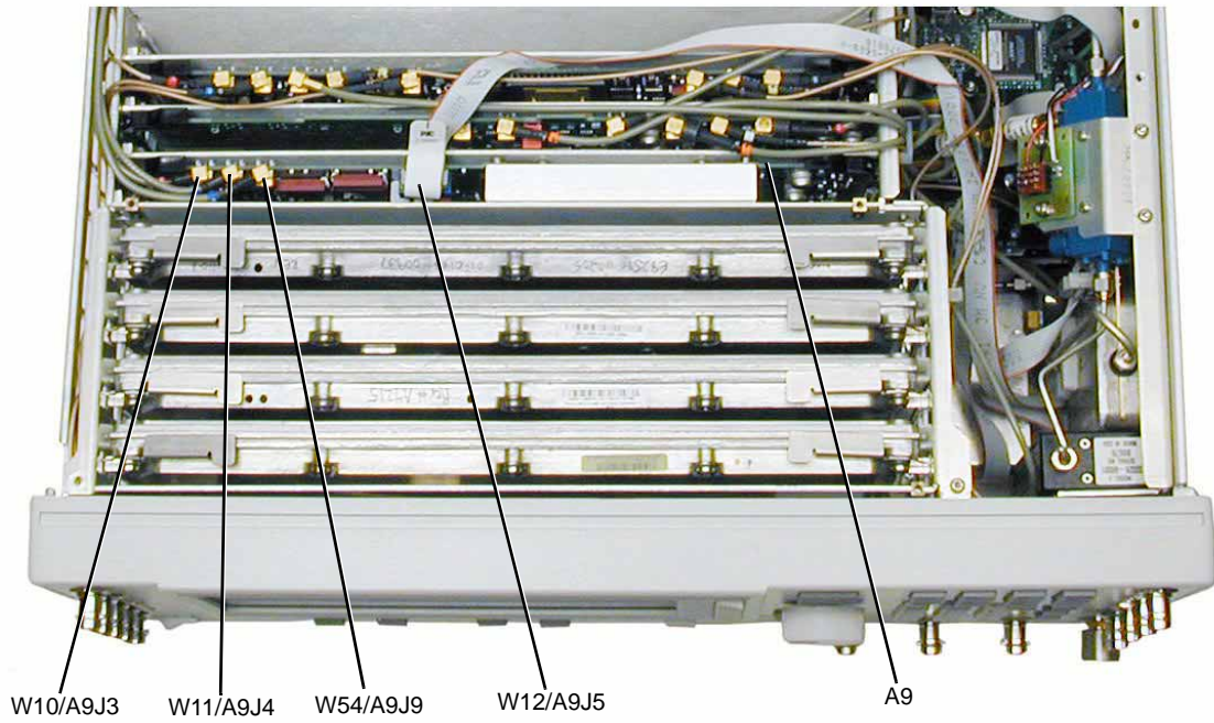
Figure 3-14 A9 YIG Driver
