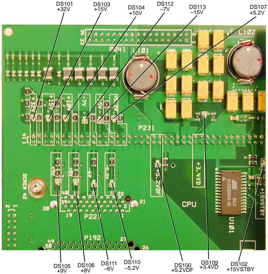
E8257D Motherboard Power Supply LEDs
