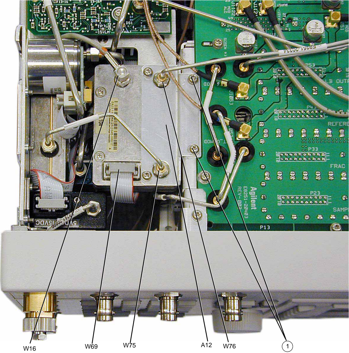
Figure 3-17 A12 Pulse Modulator Board
