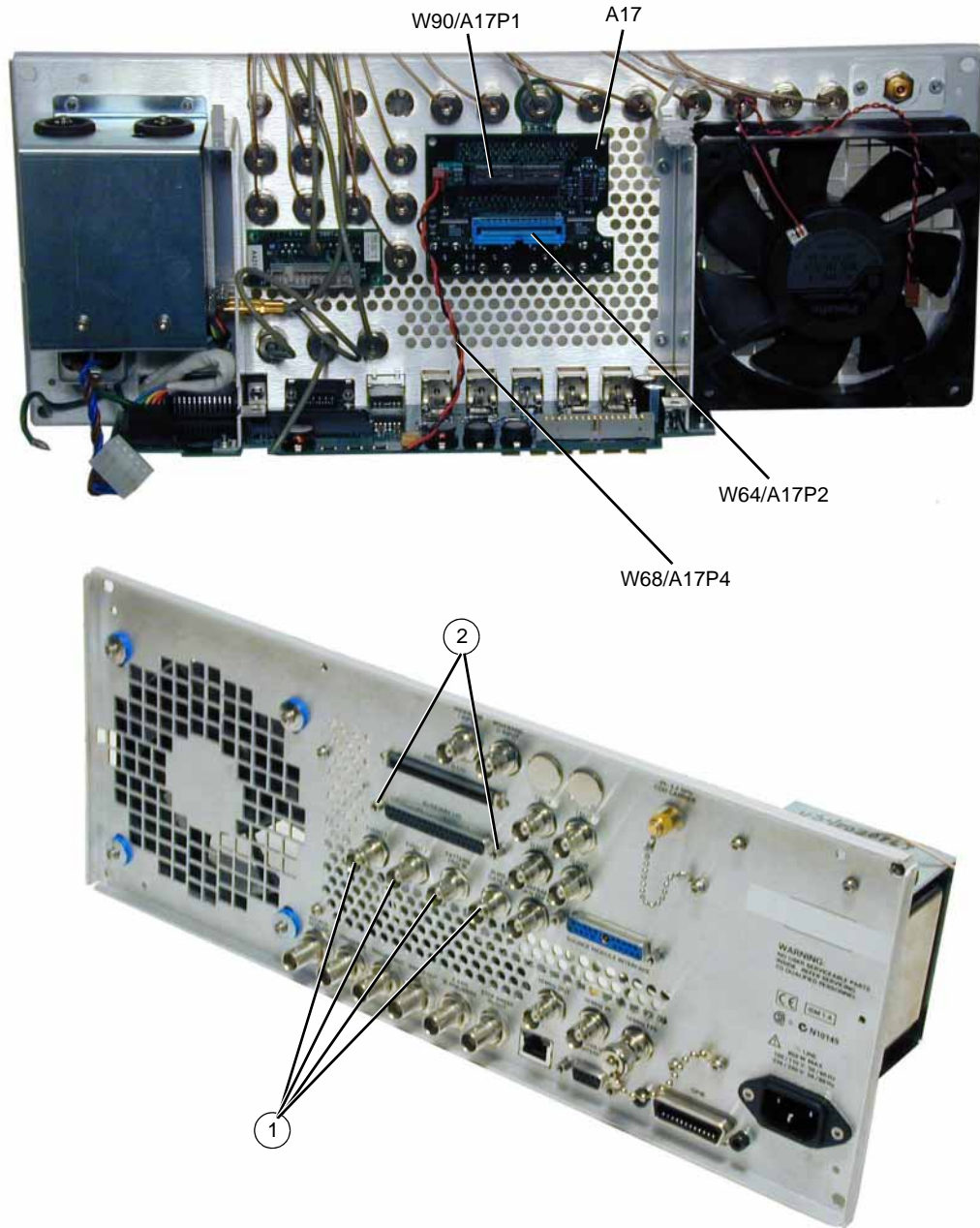
Figure 3-21 A17 Rear Panel Interface Board
