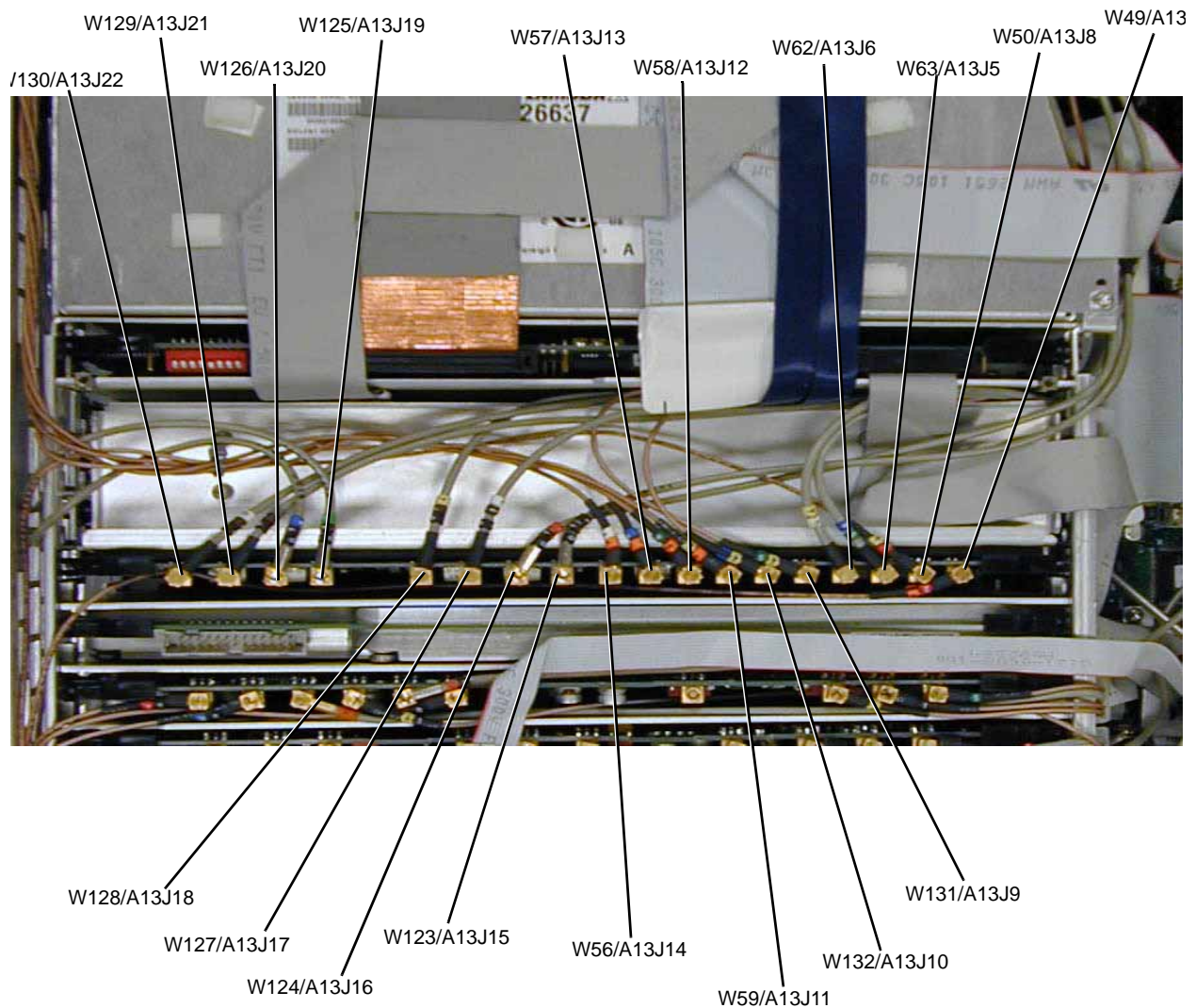
Figure 3-19 A13 I/Q MUX (E8267D Standard or with Option 016) (Serial Prefixes >US4722/MY4722)
