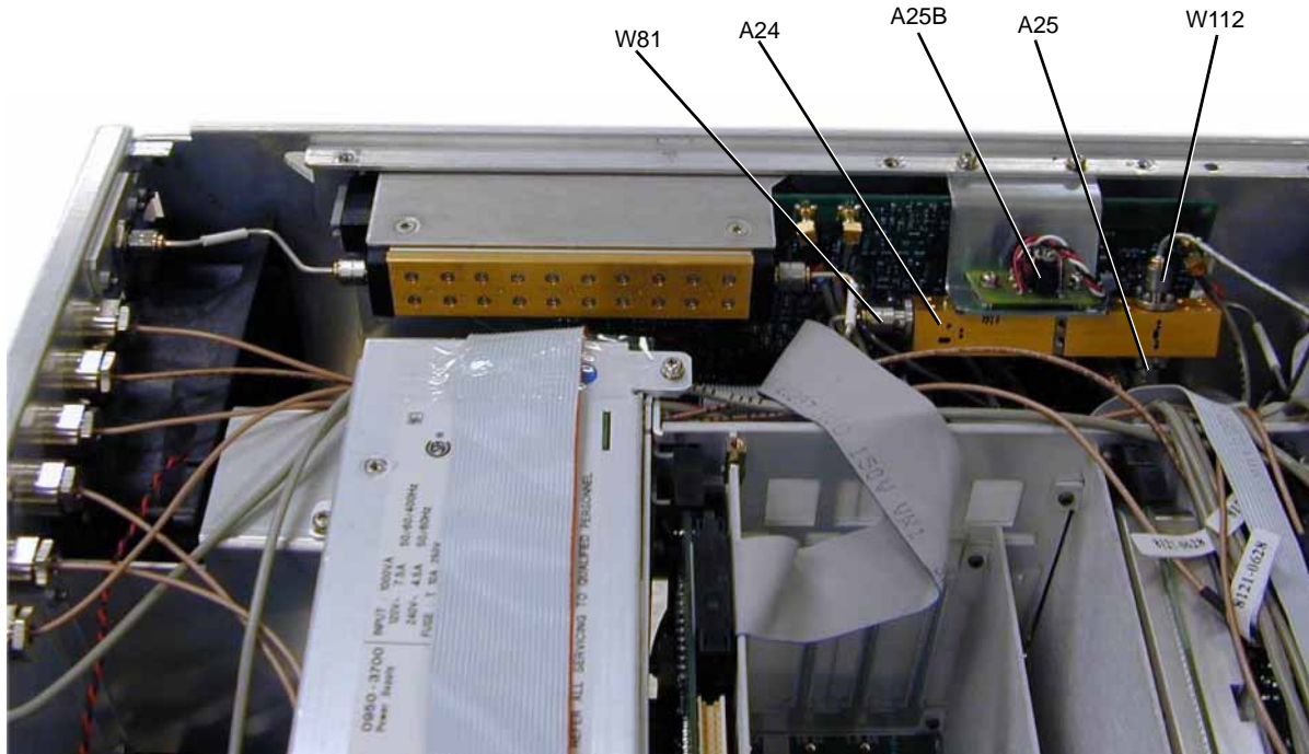
Figure 3-38 A24 67 GHz Highband Coupler (Options 550 & 567 and Option 1EM)
