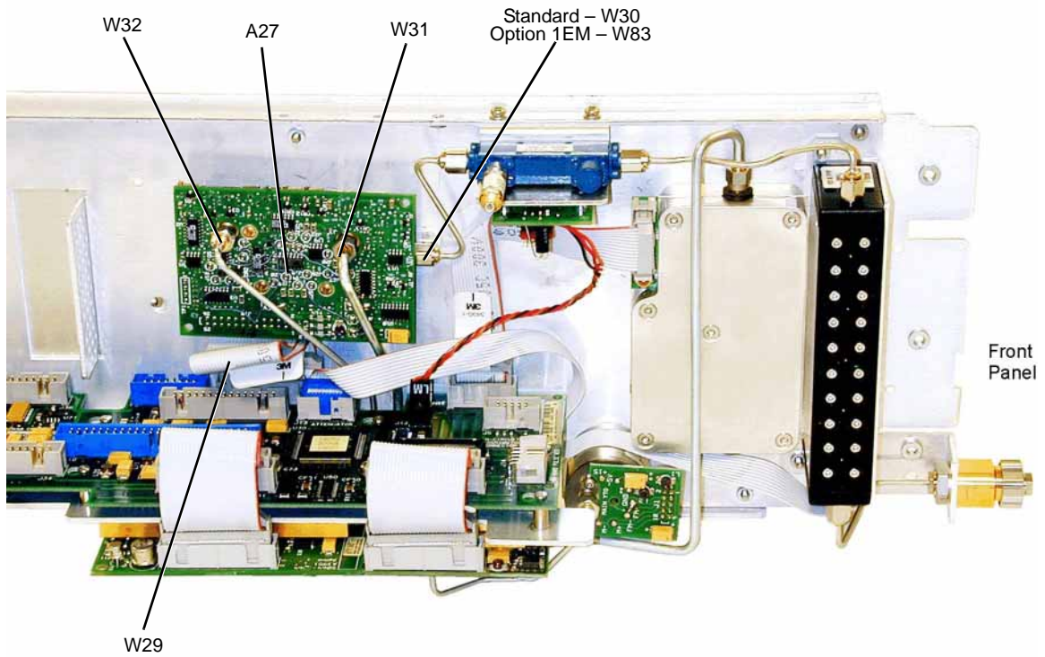
Figure 3-47 A27 40 GHz Doubler (Option 540)
