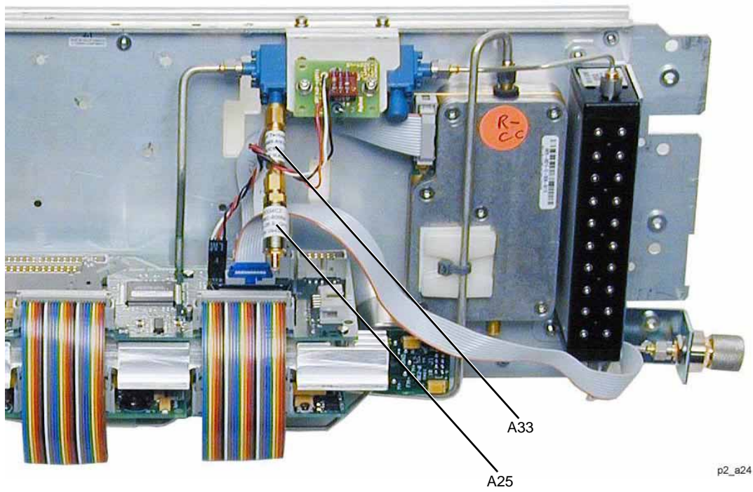
Figure 3-39 A25 20 GHz Highband Detector (Options 503, 509, & 520)
