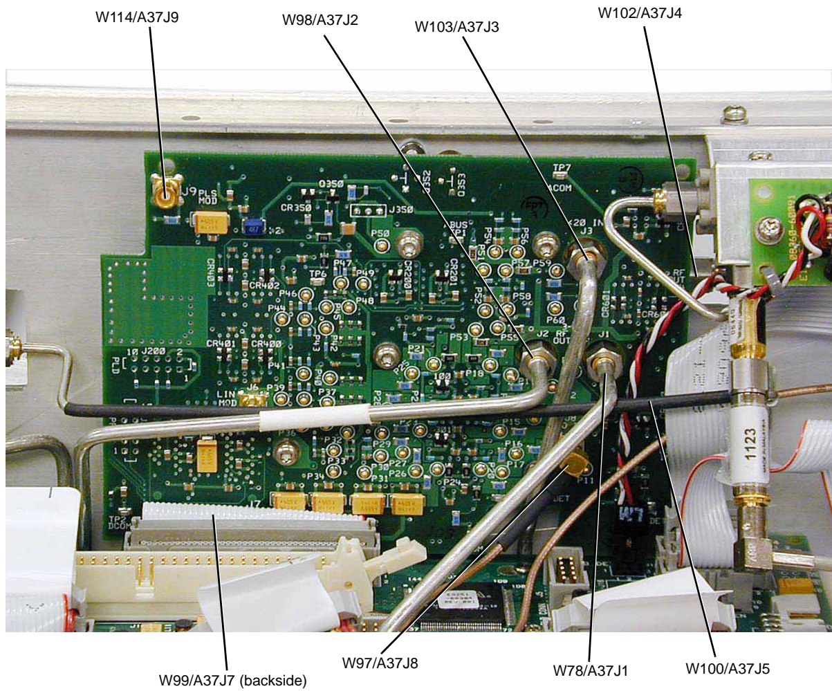
Figure 3-63 A37 Upconverter
