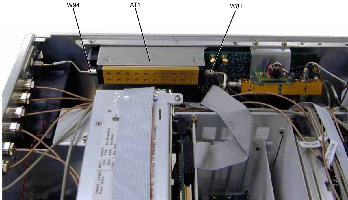
Figure 3-74 AT1 90 dB Attenuator (Options 1EM)
