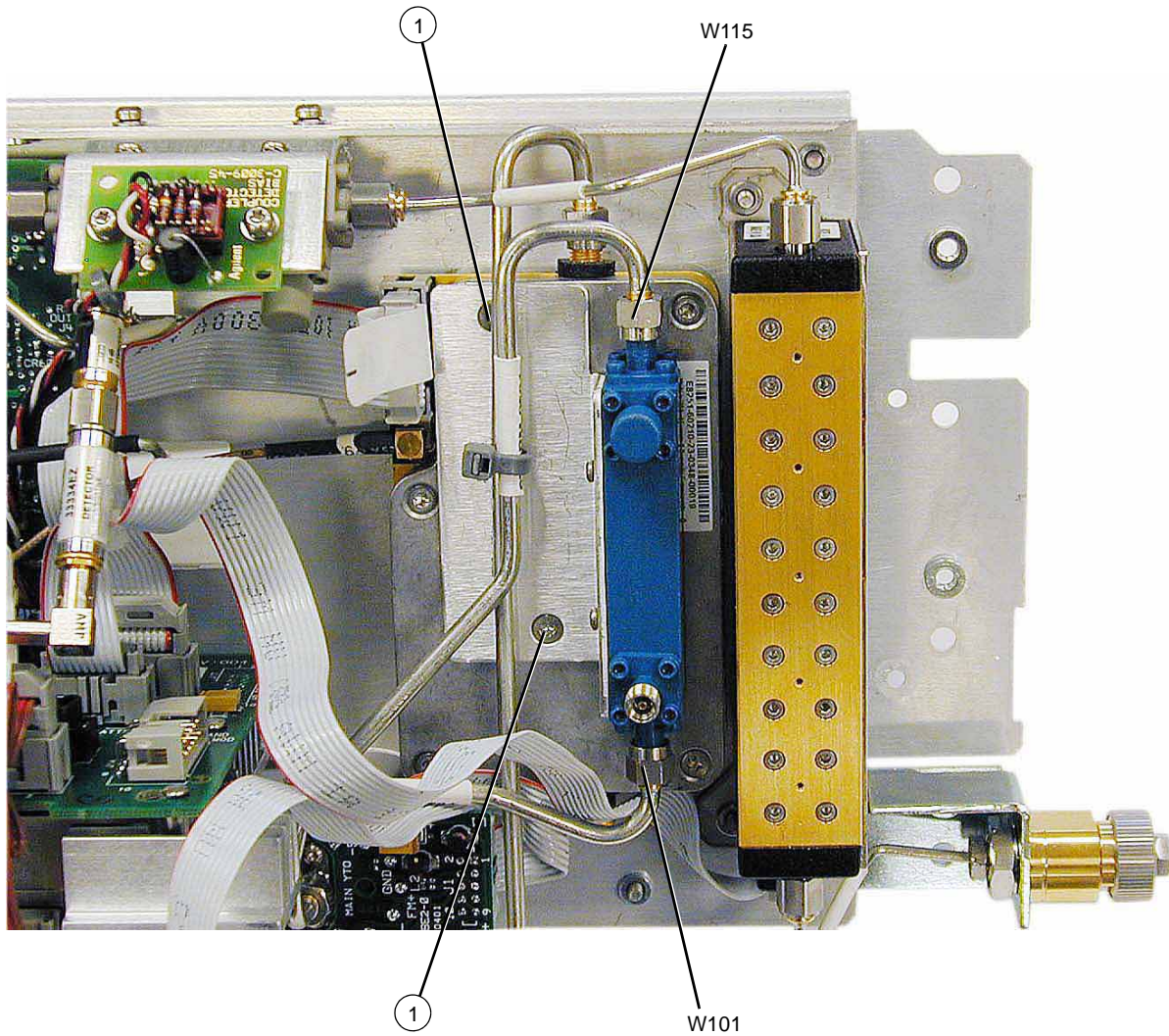
Figure 3-65 A39 Directional Sweep Coupler
