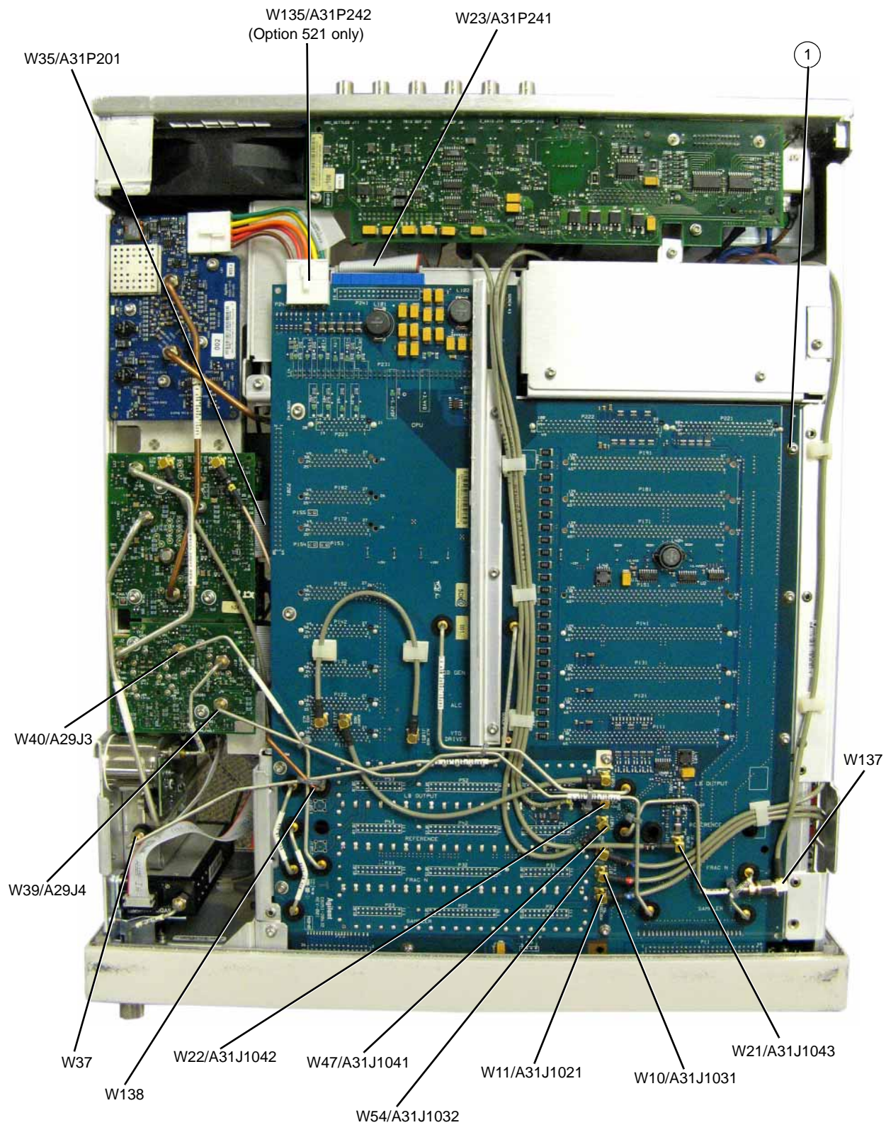
Figure 3-52 A31 Motherboard (E8257D & E8663D)
