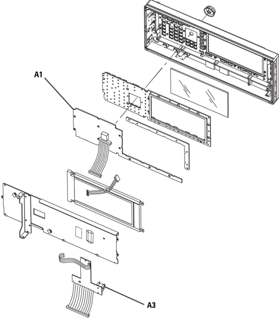
Figure 2-2 Assemblies from the Inside Front Panel View for with serial prefixes > US/MY5XXX3XXX
