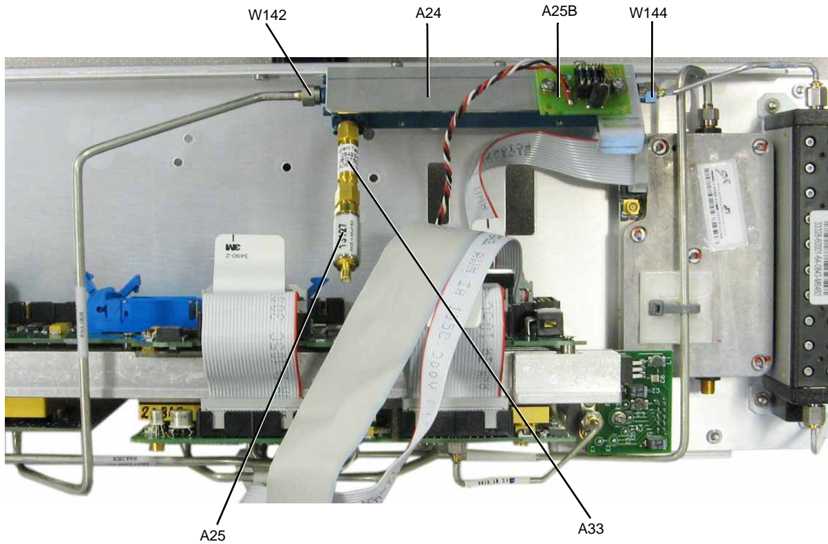
Figure 3-31 A24 20 GHz Highband Coupler (Option 521 - Standard)
