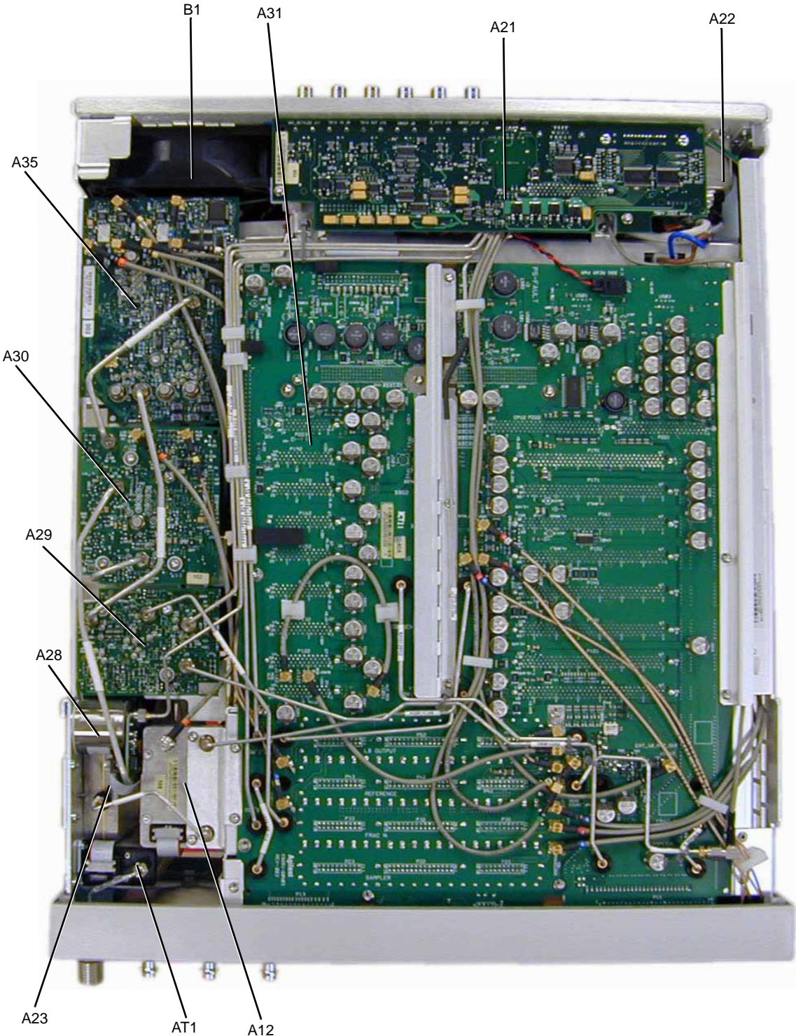
Figure 2-14 Assemblies from a Bottom View (E8267D)
