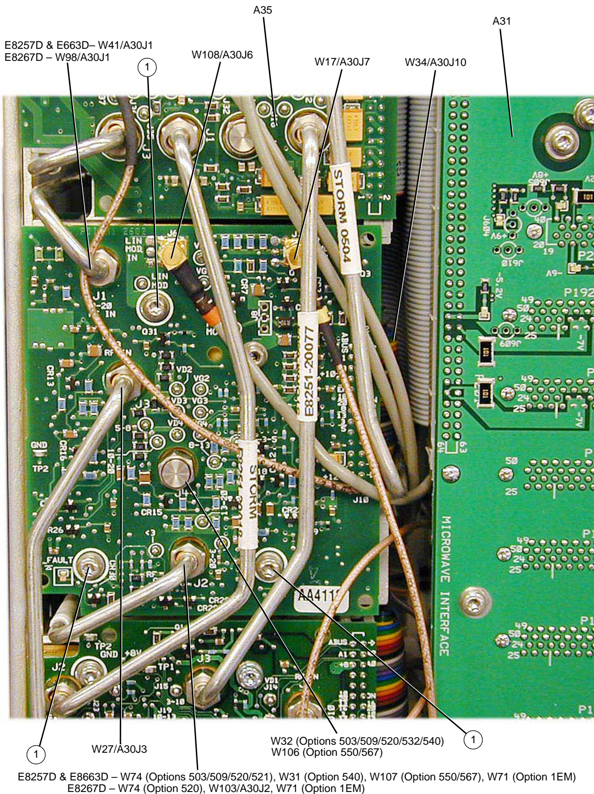
Figure 3-51 A30 Modulator Filter
