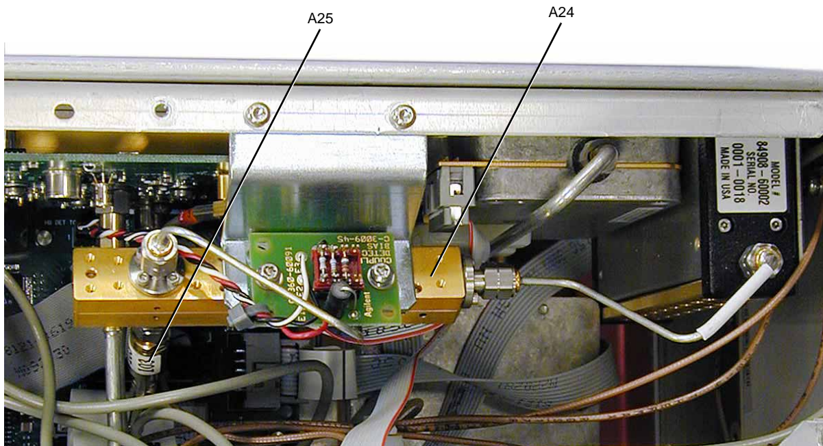
Figure 3-43 A25 67 GHz Highband Detector (Options 550 and 567)
