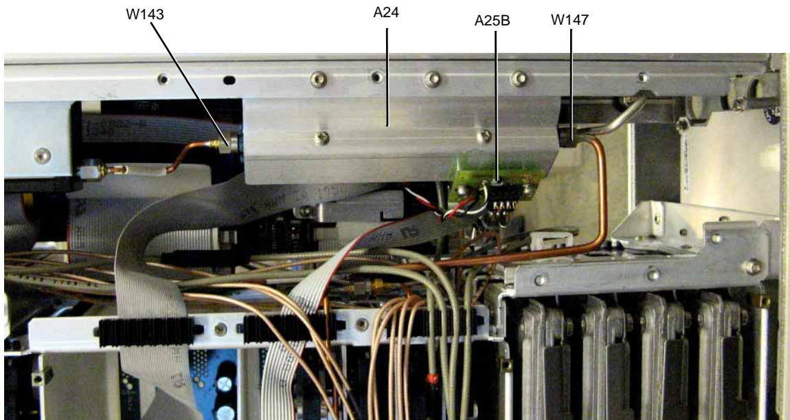
Figure 3-32 A24 20 GHz Highband Coupler (Option 521 - Option 1EM)
