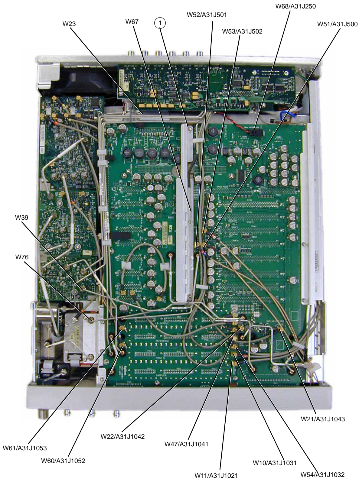
Figure 3-53 A31 Motherboard (E8267D)
