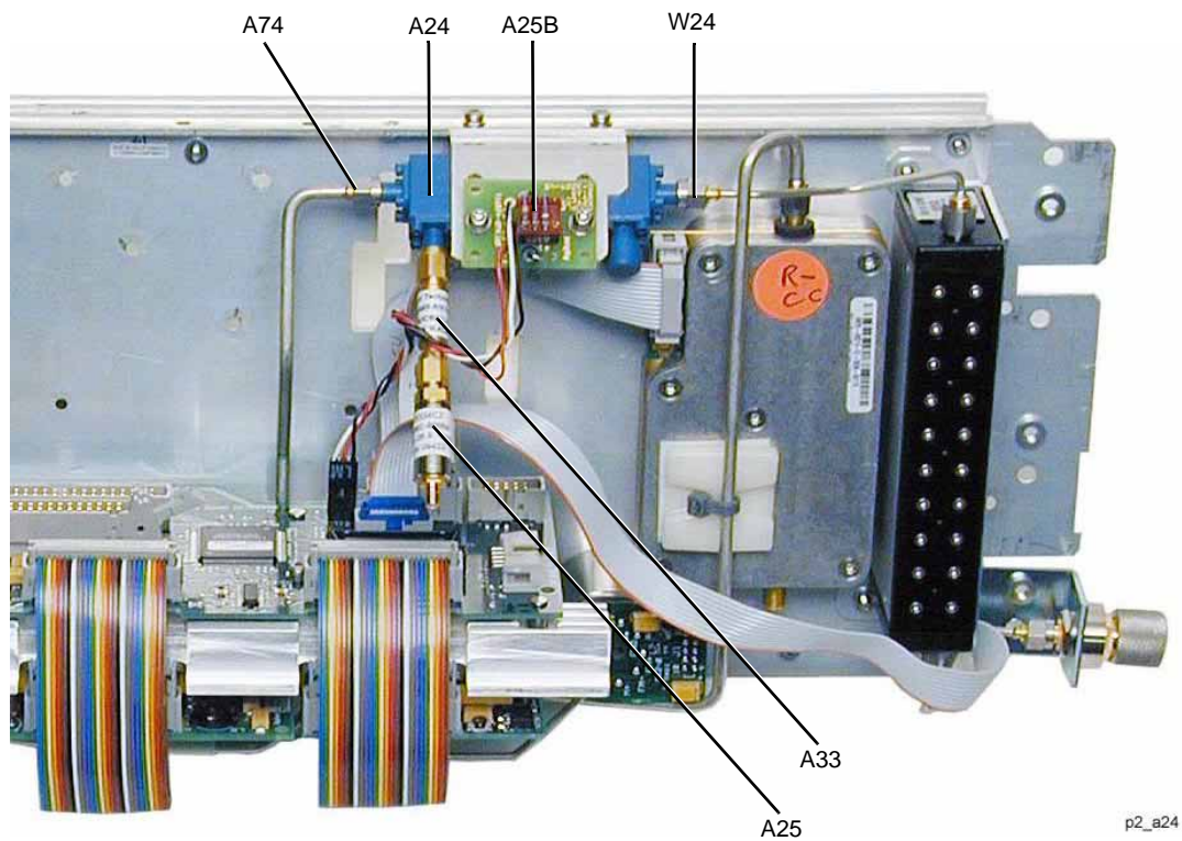
Figure 3-29 A24 20 GHz Highband Coupler (Options 503, 509, and 520 – Standard)
