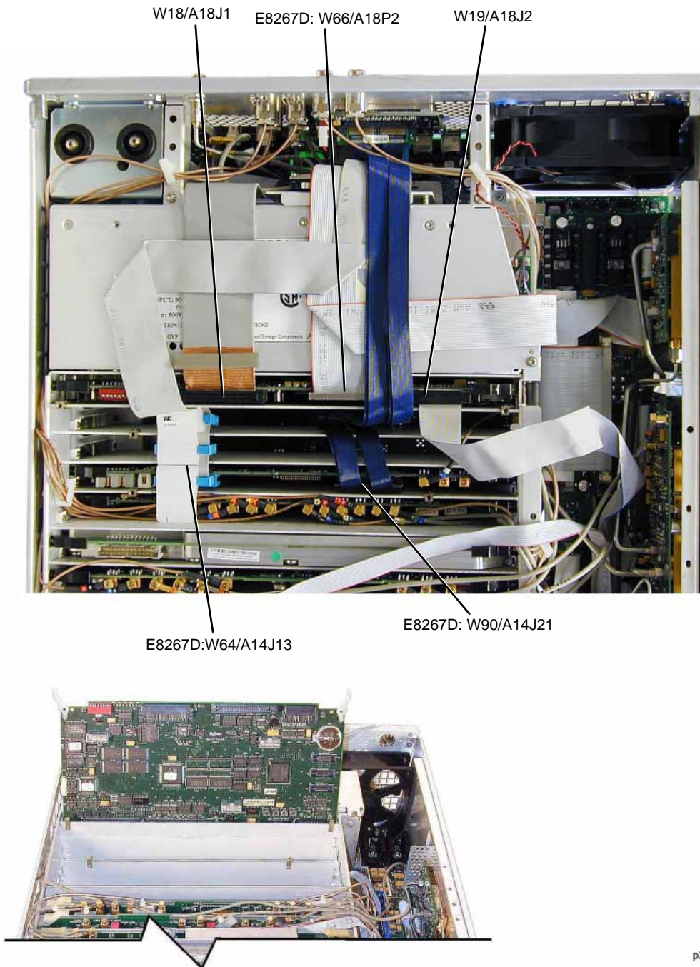
Figure 3-23 A18BT1
