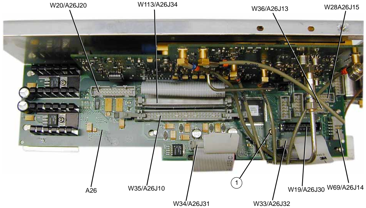
Figure 3-45 A26 MID (E8257D & E8663D)
