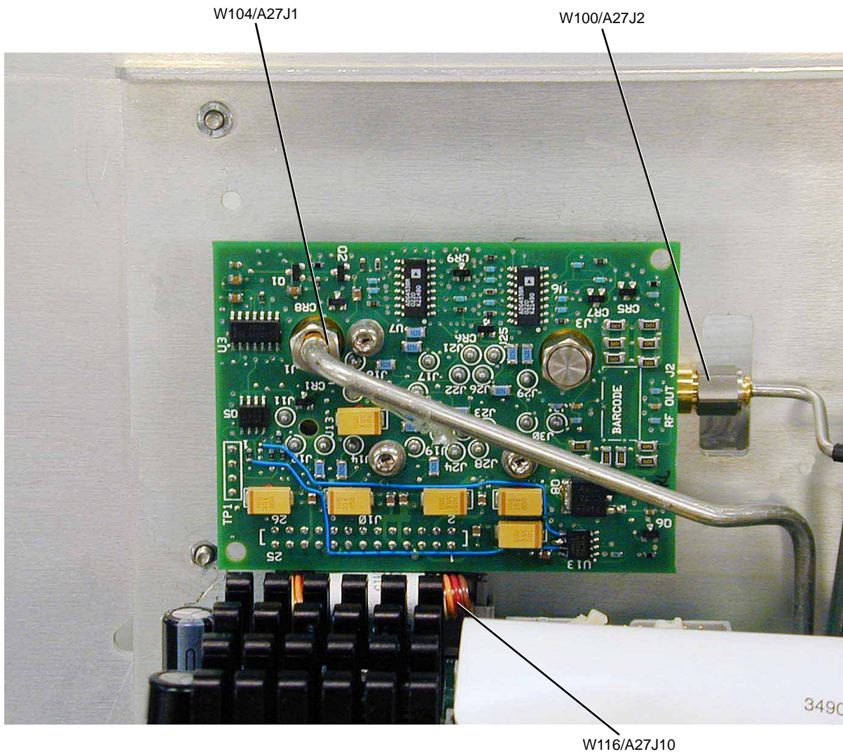
Figure 3-48 A27 40 GHz Doubler (Options 532 and 544)
