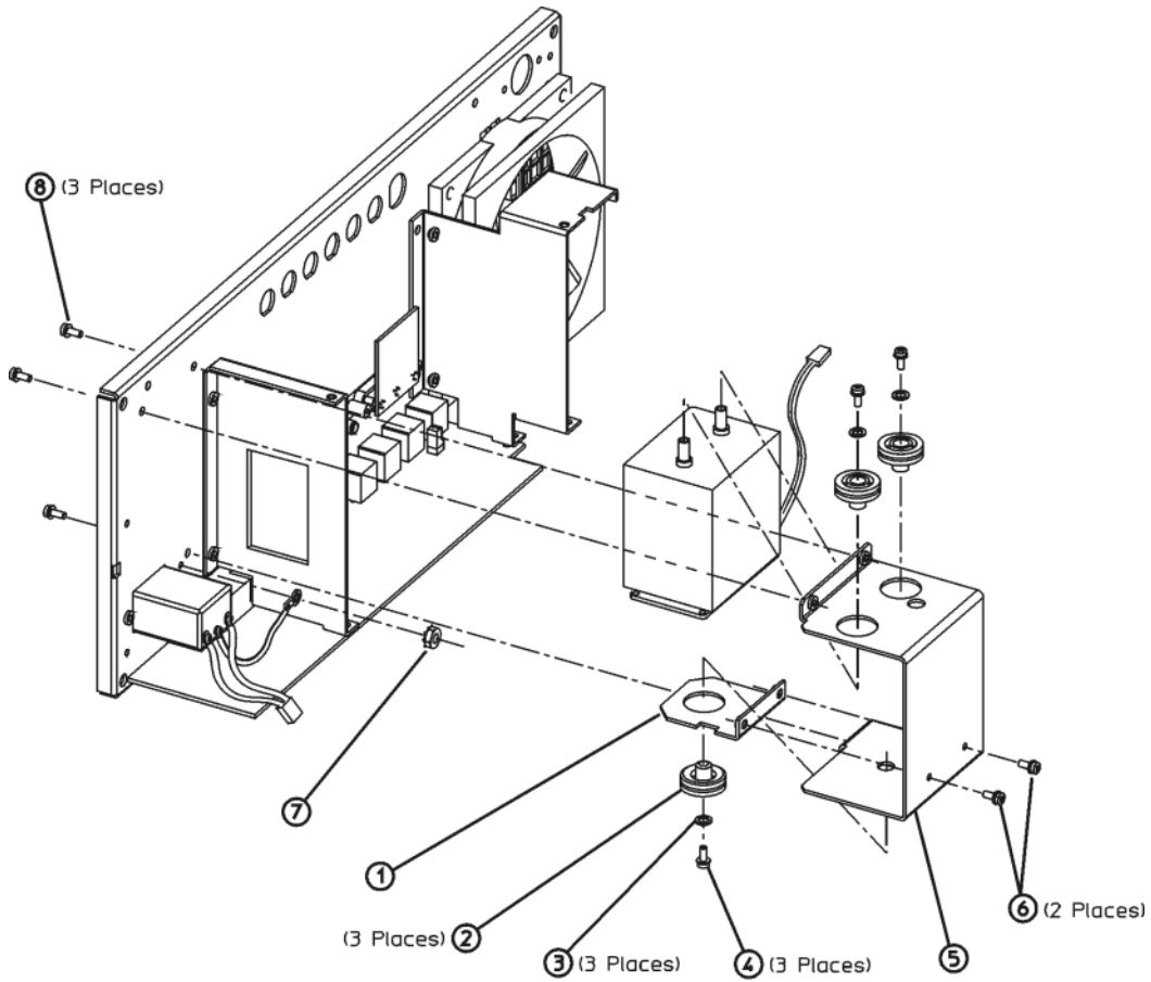
Disassembled A32 10 MHz Crystal Oscillator (Option UNR/UNX and Instruments with Serial Prefixes > US4805/MY4805)
