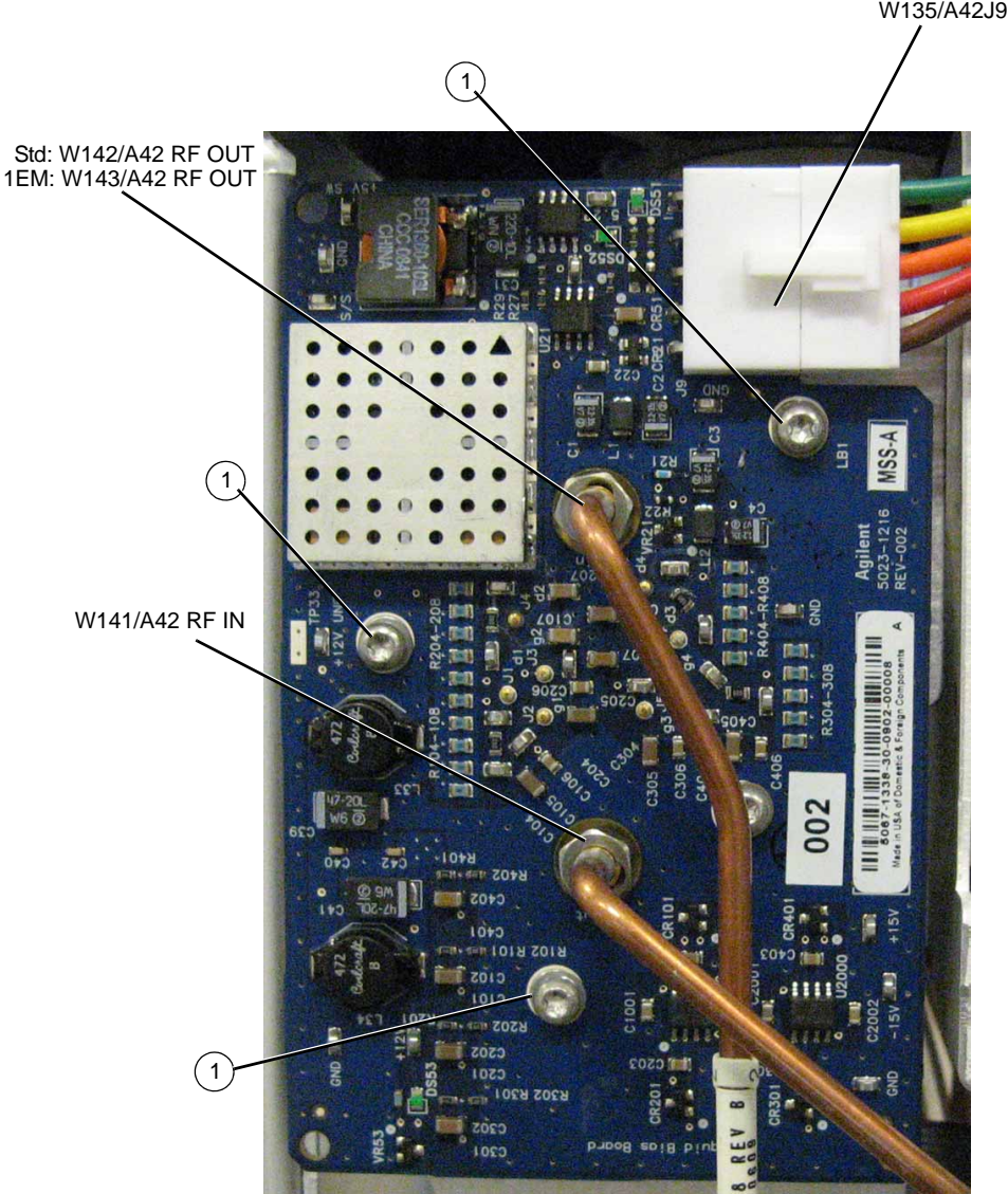
Figure 3-69 A42 20 GHz Power Amp
