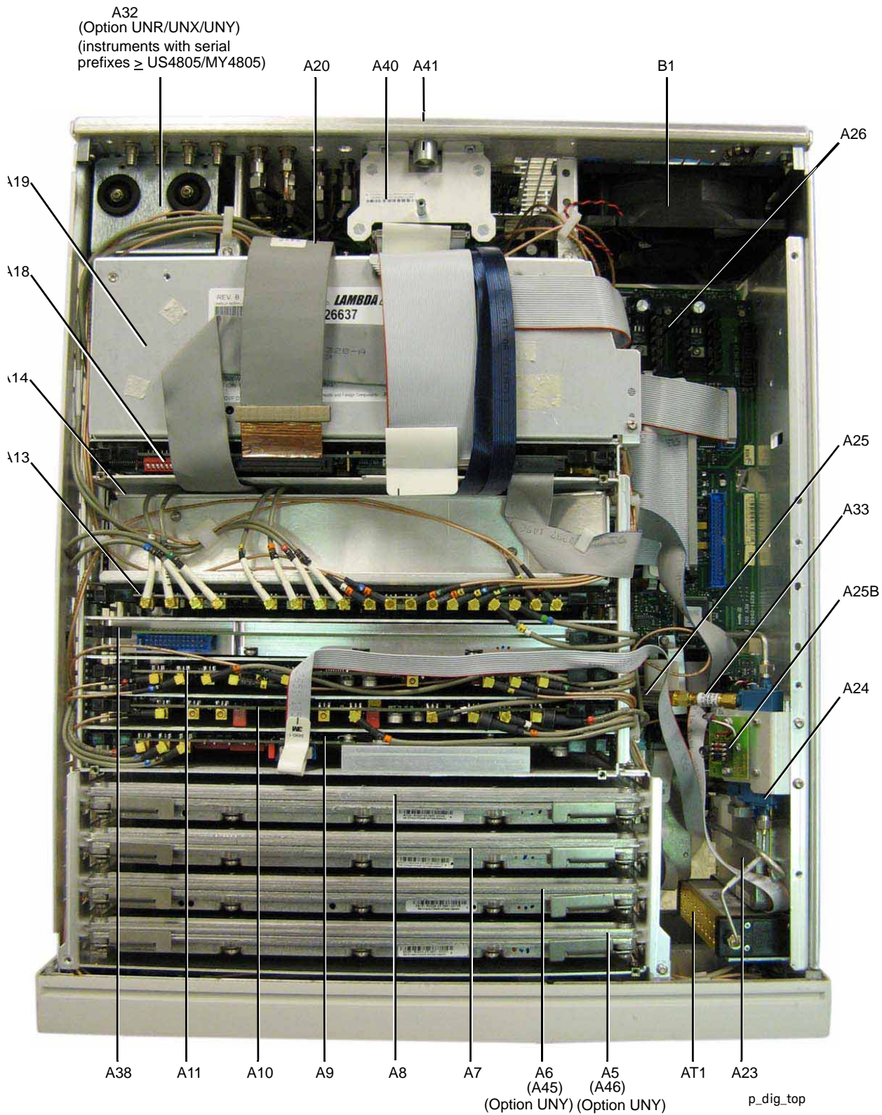
Figure 2-6 Assemblies from a Top View (E8267D Option 520)
