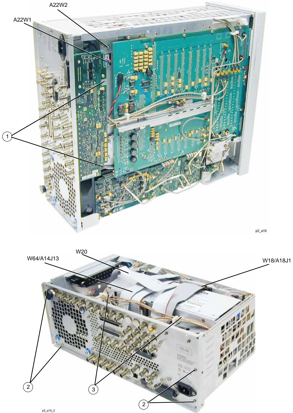
Figure 3-58 Rear Panel Removal (Option 1EM)
