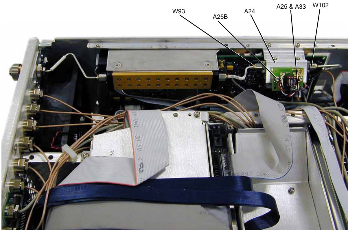
Figure 3-36 A24 50 GHz Highband Coupler (Options 532 & 544 – Option 1EM)
