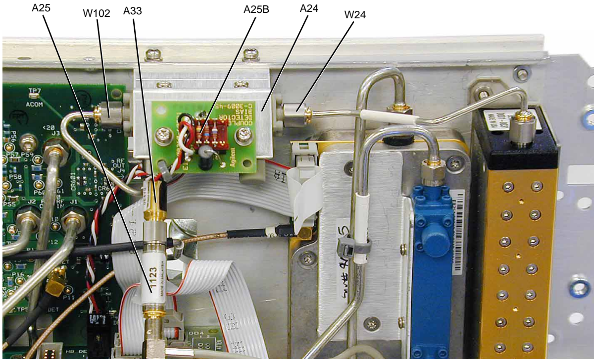
Figure 3-35 A24 50 GHz Highband Coupler (Options 532 & 544 – Standard)
