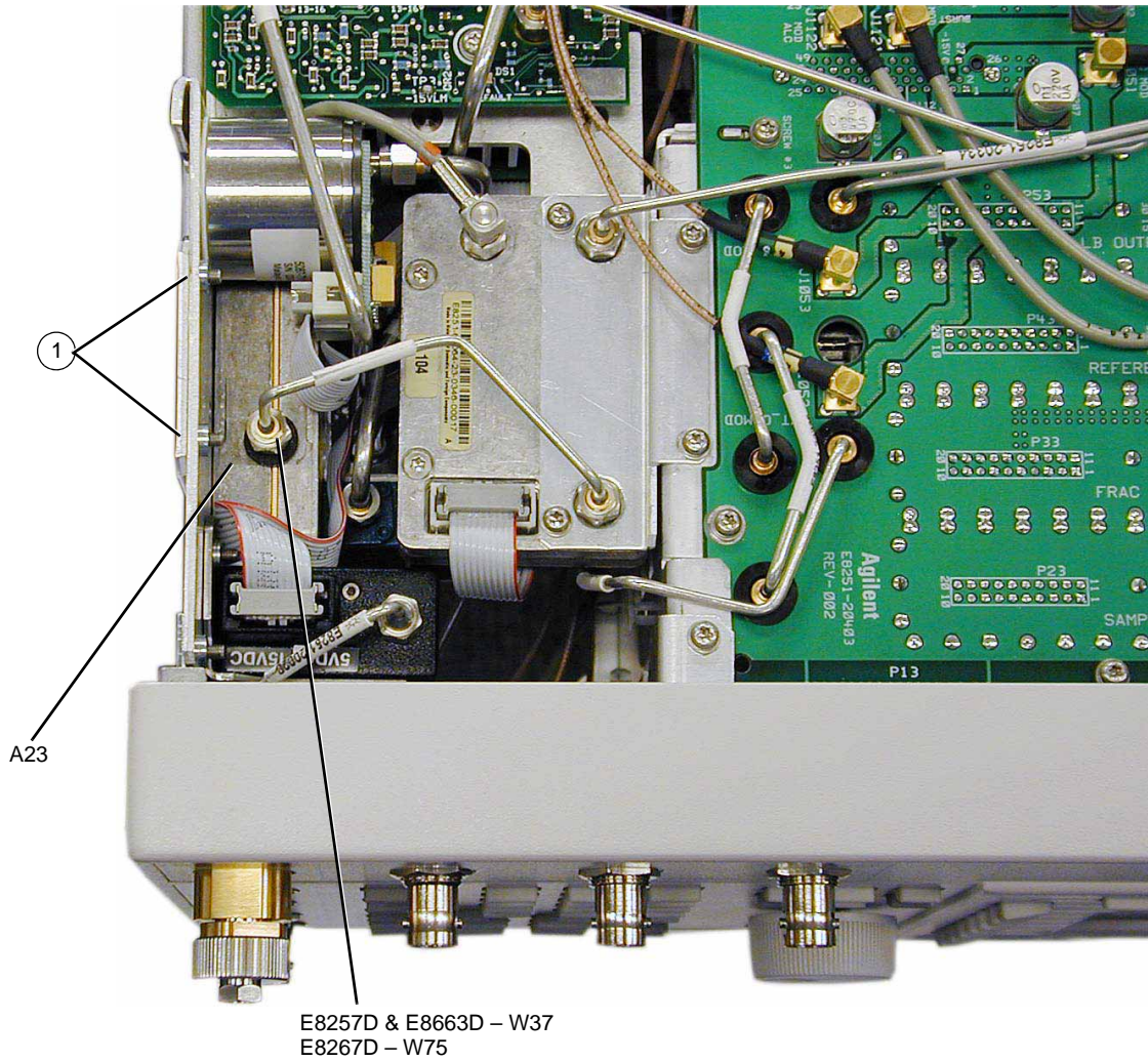
Figure 3-28 A23 Lowband Coupler/Detector
