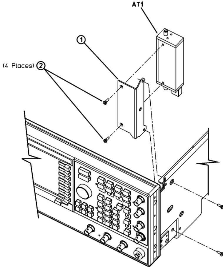
Figure 2-21 Disassembled AT1 90dB/115dB Attenuator View (Option 1E1)
