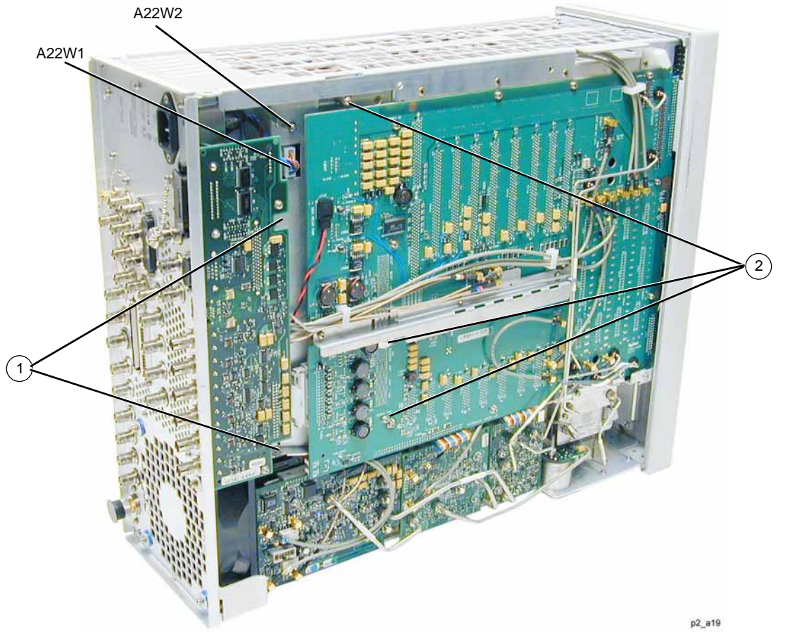
Figure 3-24 A19 Power Supply Removal
