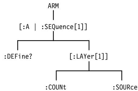
Figure 2–4: ARM subsystem hierarchy
