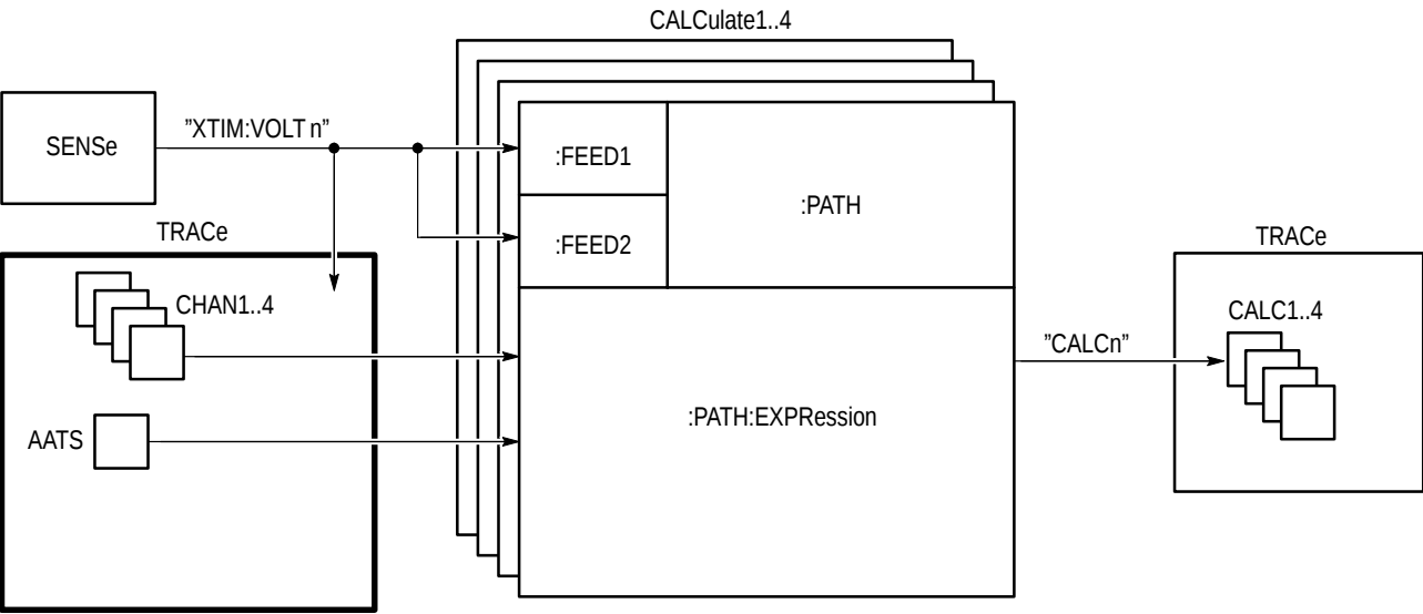
Figure 2-8: CALCulate subsystem functional model
