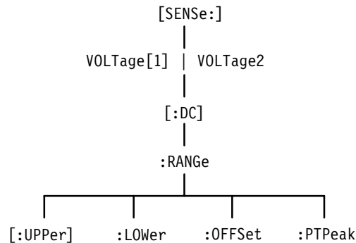
Figure 2–33: VOLTage subsystem hierarchy
