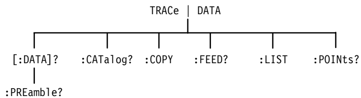
Figure 2–25: TRACe subsystem hierarchy
