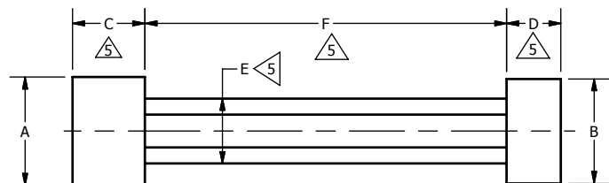
FIG. 2 (TRILOCK TYPE)
