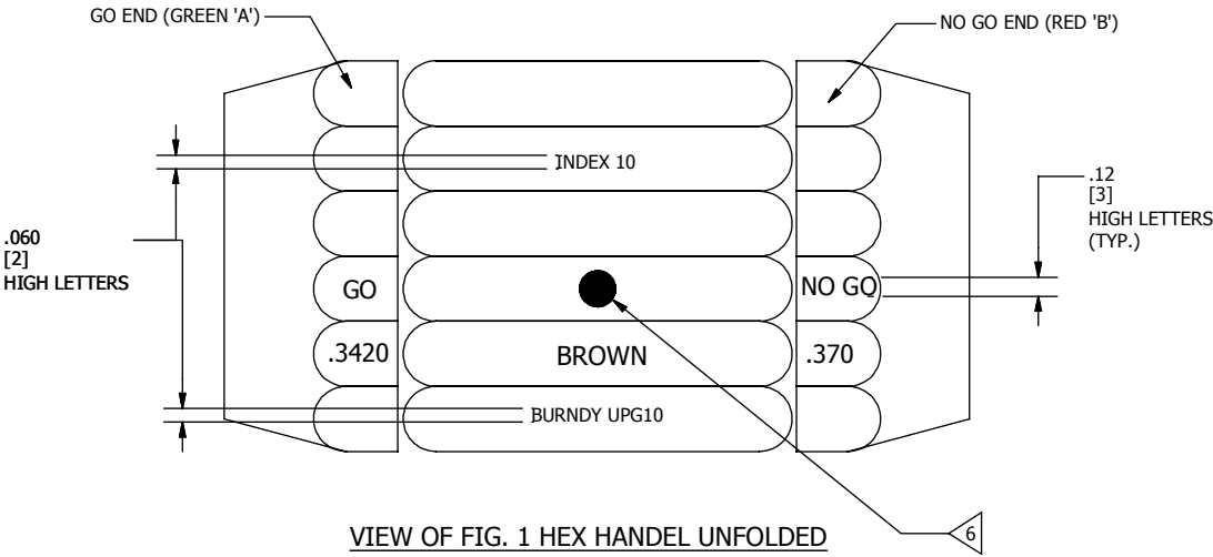
FIG. 1 (WIRE TYPE)
