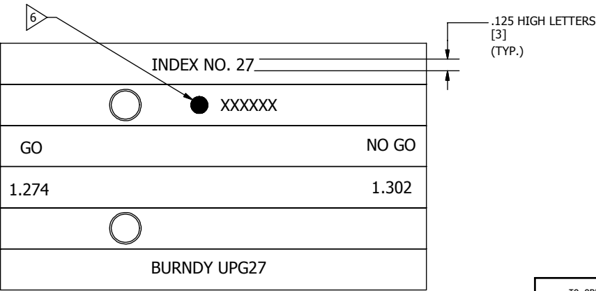
VIEW OF FIG. 3 HEX HANDLE UNFOLDED
