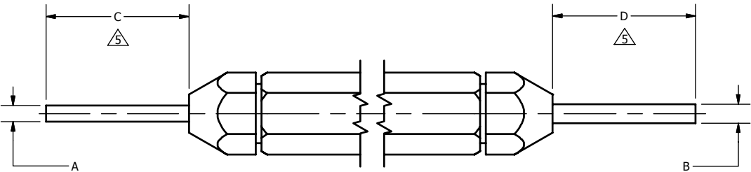
FIG. 1 (WIRE TYPE)
