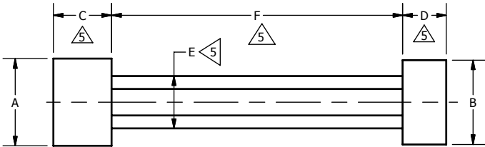
FIG. 2 (TRILOCK TYPE)
