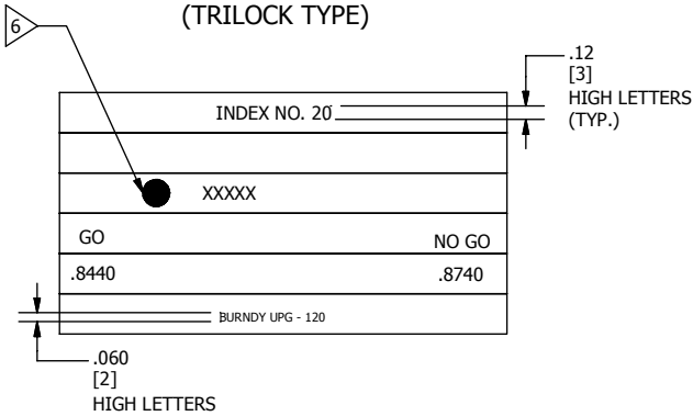
FIG. 2 (TRILOCK TYPE)
