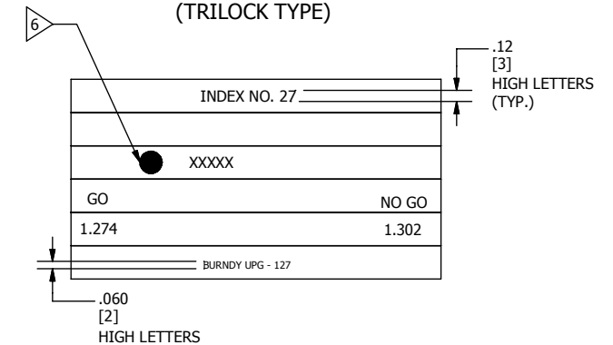
VIEW OF FIG. 2 HEX HANDEL UNFOLDED
