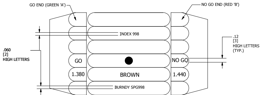
VIEW OF FIG. 1 HEX HANDEL UNFOLDED
