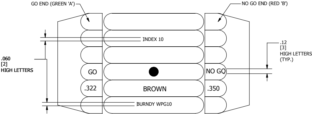
VIEW OF FIG. 1 HEX HANDEL UNFOLDED
