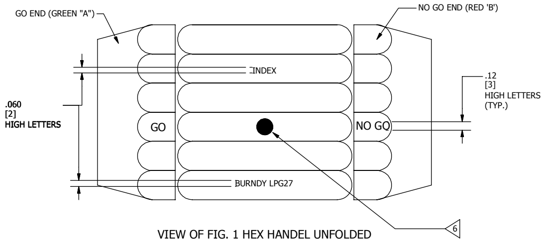
VIEW OF FIG. 1 HEX HANDEL UNFOLDED
