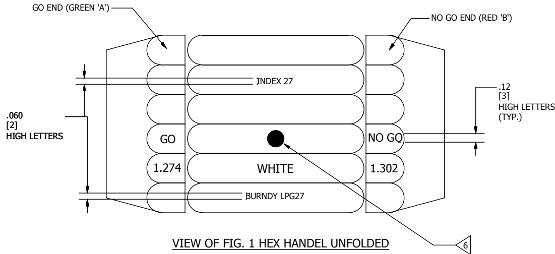
FIG. 1 (WIRE TYPE)
