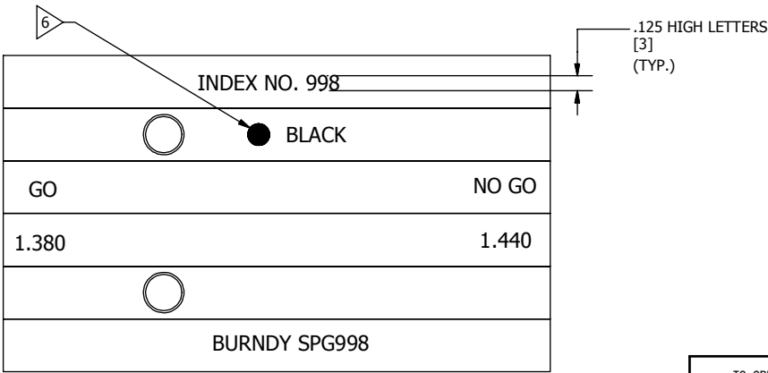
VIEW OF HEX HANDLE UNFOLDED TYP. FOR FIG 3&4
