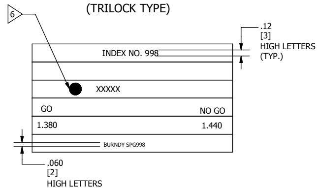
VIEW OF FIG. 2 HEX HANDEL UNFOLDED
