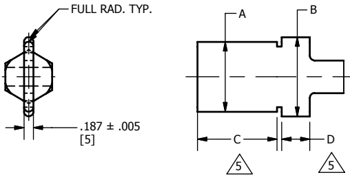
FIG. 4 & 4A (USE SAME HANDLE AS FIG. 3)
